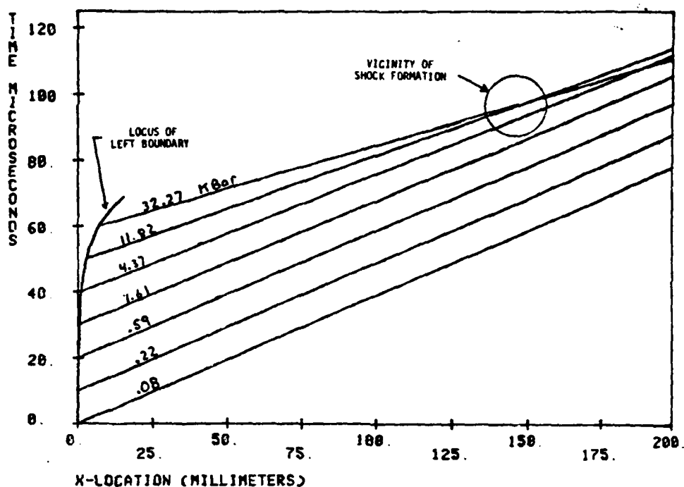
Figure 6a. Characteristics diagram demonstrating the shock formation in a solid (Aluminum, \rho_0 = 1.6 \text{ g/cc} , C_0 = 2.56 \text{ mm}/\mu\text{sec} ) due to compression waves generated by an exponential pressure rise ( P = .08e^{.1t} ).
