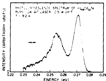
FIG. 1. Photoluminescence intensity vs energy of emitted photon for \text{Hg}_{0.68}\text{Cd}_{0.32}\text{Te} . The high-energy peak is attributed to a band-to-band transition. The low-energy peak is attributed primarily to donor-to-acceptor luminescence below \sim 10 K, and band-to-acceptor luminescence at higher temperature. The fine structure seen on the low-energy peak is due to absorption by water vapor.
