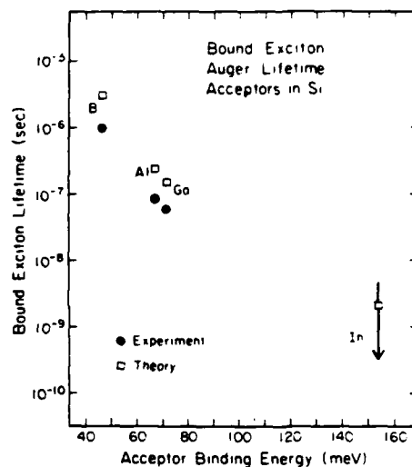
Fig. 1. Bound exciton lifetimes vs impurity binding energy for the four common acceptors in Si. The hollow squares are our calculations of the Auger lifetime and the solid circles are our measured values. In Si:In, we have only been able to set an upper bound on the measured lifetime of 5 nsec (indicated by the top of the arrow). Schmid[8] has recently found a measured lifetime of 2.7 nsec for Si:In.
