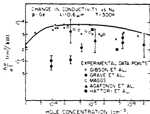
FIG. 1. Values of (-\Delta\sigma/\sigma) versus the hole concentration in p -Ge for \text{CO}_2 laser excitation at 10.6 \mu\text{m} , room temperature, and low light intensities. The calculated values of (-\Delta\sigma/\sigma) are shown by the solid curve. The experimental data are taken from \times , Ref. 4; \bullet , Ref. 5; \circ , Ref. 6; \bullet , Ref. 7; and \circ , Ref. 9. Error bars are reported only in Refs. 5 and 7.
