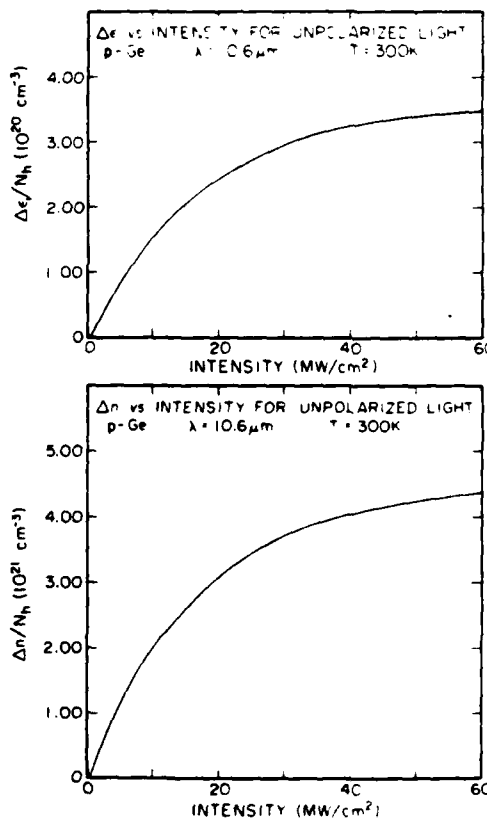
FIG. 2. The top panel gives the calculated values of the change in the real part of the dielectric constant (divided by the density of free holes) as a function of intensity for p\text{-Ge} at \lambda = 10.6 \mu\text{m} , T = 300 \text{ K} , and for unpolarized light. The corresponding values for the change in the index of refraction are given in the lower panel.
