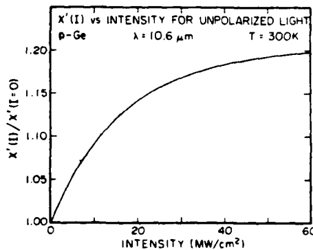
FIG. 1. Calculated values of \chi'(I)/\chi'(I=0) as a function of intensity for unpolarized light in p\text{-Ge} . The calculation was done for light with a wavelength of 10.6 \mu\text{m} and a temperature of 300 \text{ K} .
