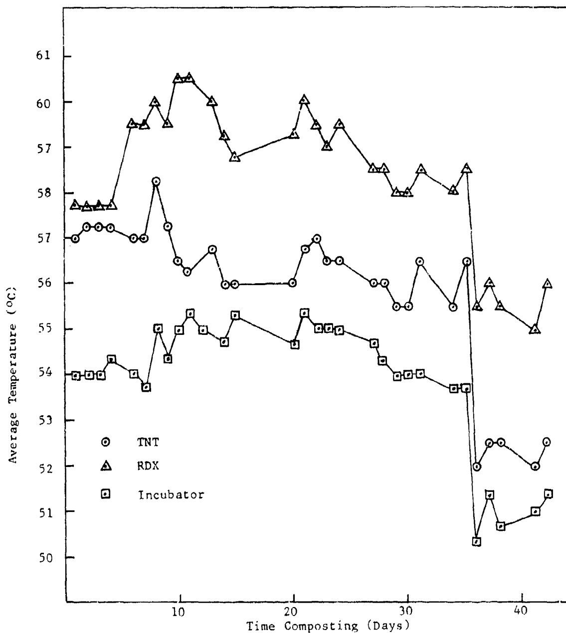
Figure 1Q Comparison of Compost Temperatures for Leachate Study
