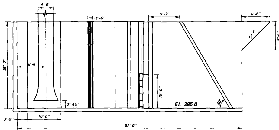
ELEVATION VIEW
