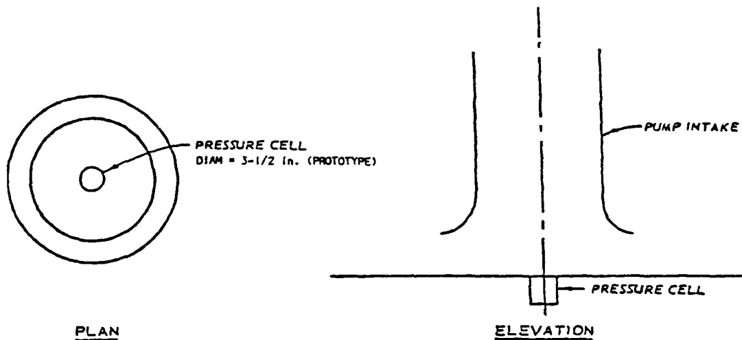
Figure 3. Pressure cell location
