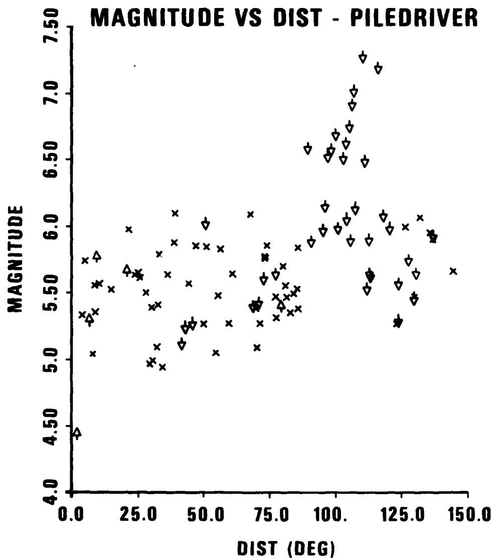
Figure 1a. Magnitude (max/GT) versus distance for PILEDRIVER. Downward and upward pointing arrows indicate noise and clipping limits respectively. The distance amplitude relation used is that of Veith and Clawson (1972) to 95° and of Sweetser and Blandford (1973) beyond, both for zero kilometers depth.
