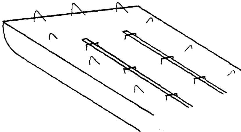
Figure 2.5 Jacket Positioning and Fendering System
