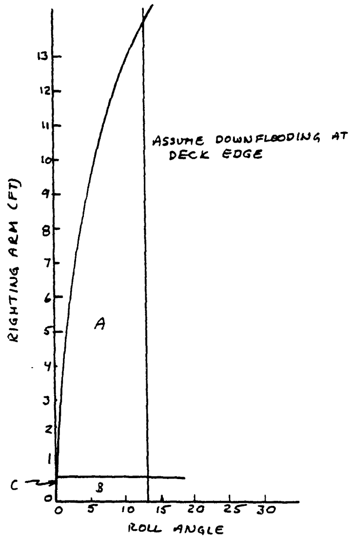
Figure 2.3 Wind Stability Criteria
