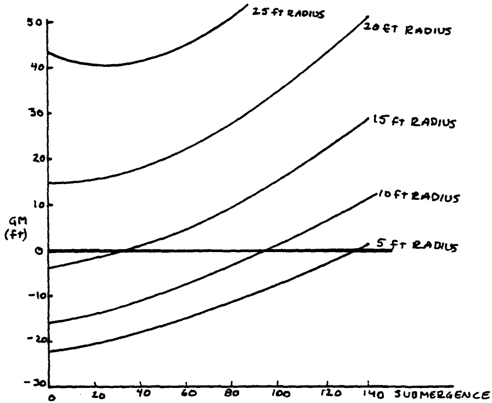
Figure 3.6 GM vs. Submergence, 6 Pontoons
