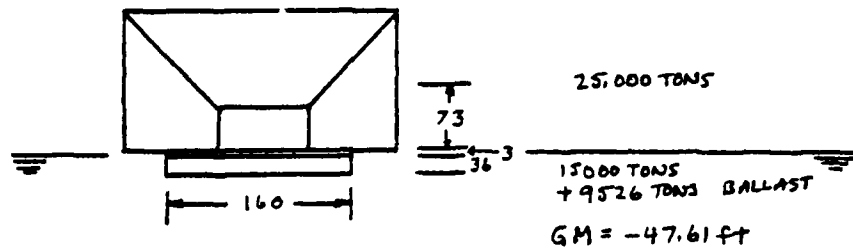
Figure 2.7 GM of Jacket Barge Combination
