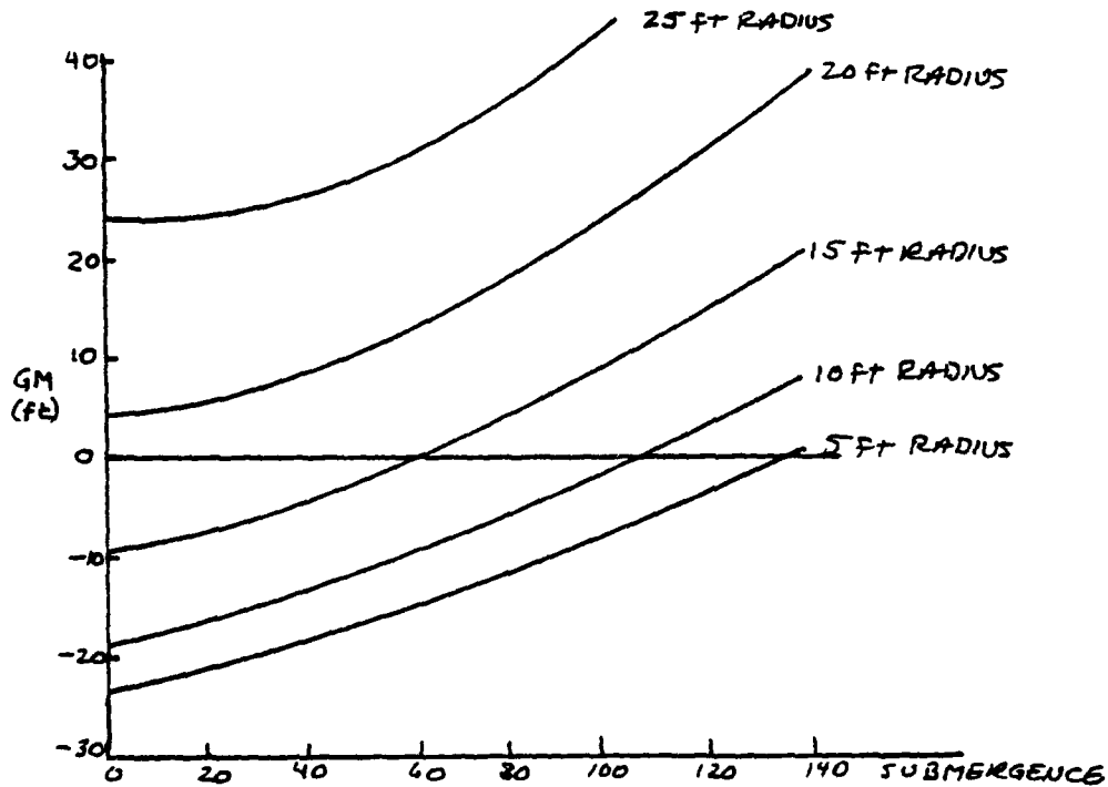
Figure 3.5 GM vs. Submergence, 4 Pontoons
