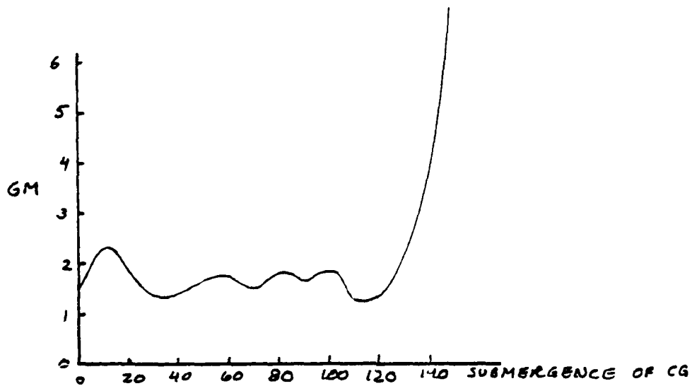
Figure 3.9 GM vs. Center of Gravity Submergence for Asymmetric Pontoons
