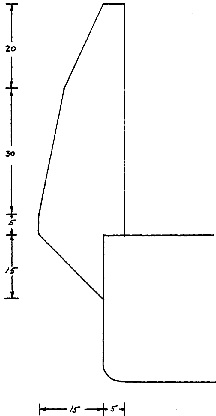
Figure 4.1 Forward End of Starboard Superstructure (Facing Aft)
