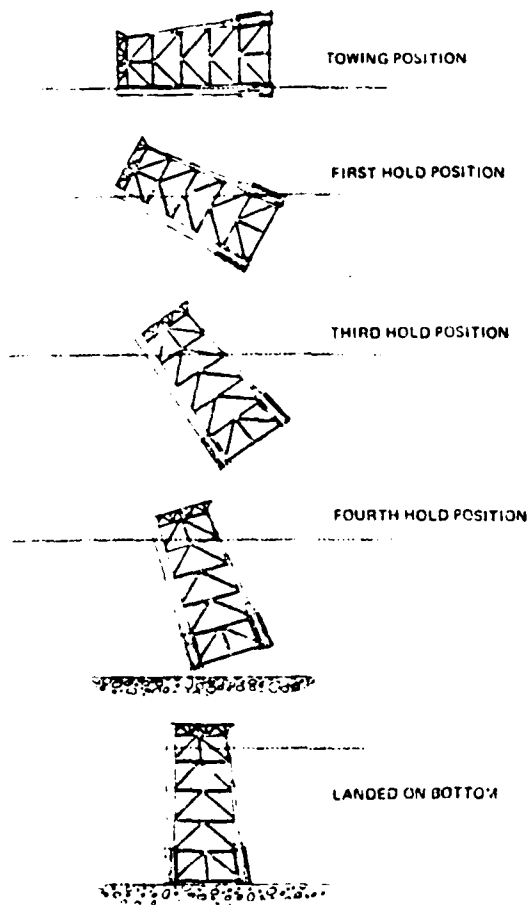
Figure 1.4 Self-Floating Tower Righting Sequence (taken from Ref. 6)
