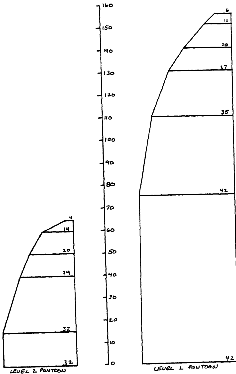
Figure 3.8 Asymmetric Clamp-On Pontoon
