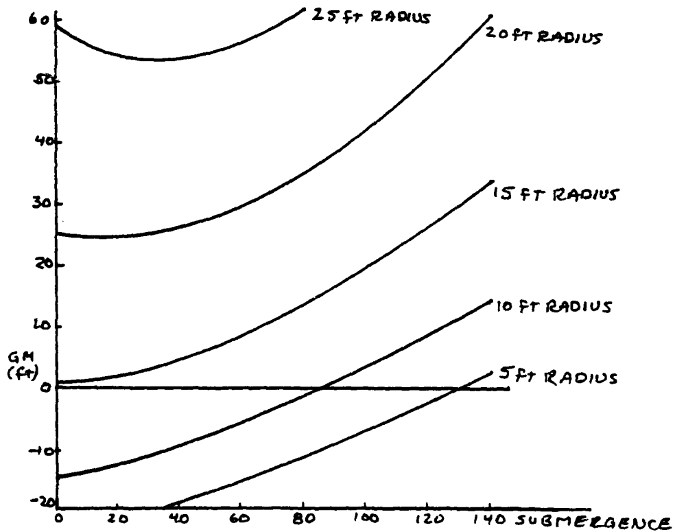
Figure 3.7 GM vs. Submergence, 8 Pontoons
