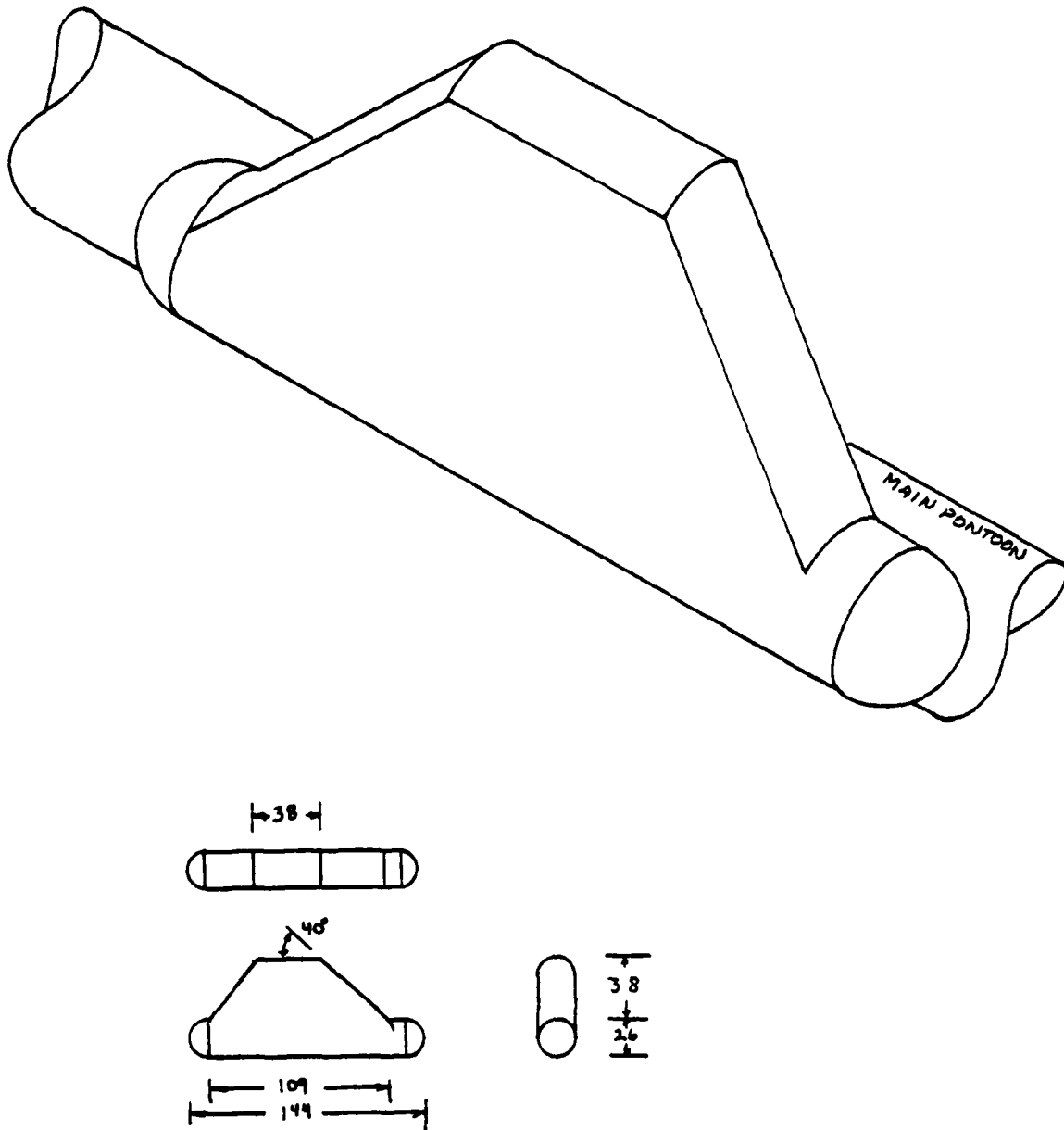
Figure 5.1 Modified Barge Sponson
