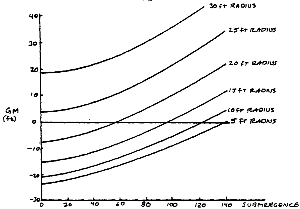
Figure 3.4 GM vs. Submergence, 2 Pontoons
