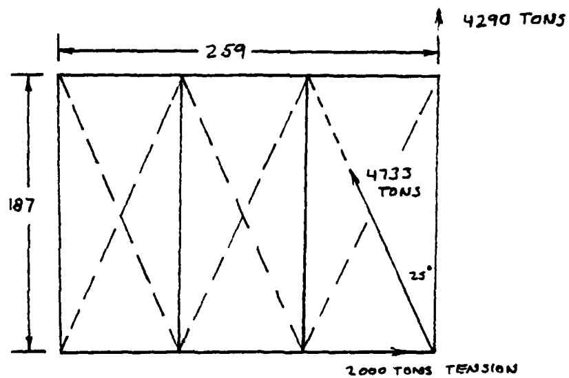
Figure 3.2 Buoyant Pontoon Force on Jacket
