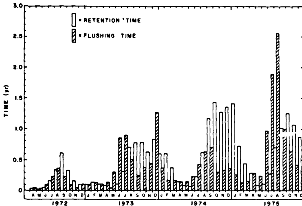
Figure 7. Monthly retention and flushing times for Lake Koonanusa, 1972 through 1975.
