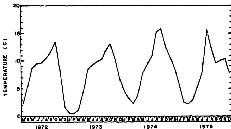
Figure 6. Monthly mean temperatures (°C) of water released from Libby Dam, measured once daily, 1972 through 1975.
