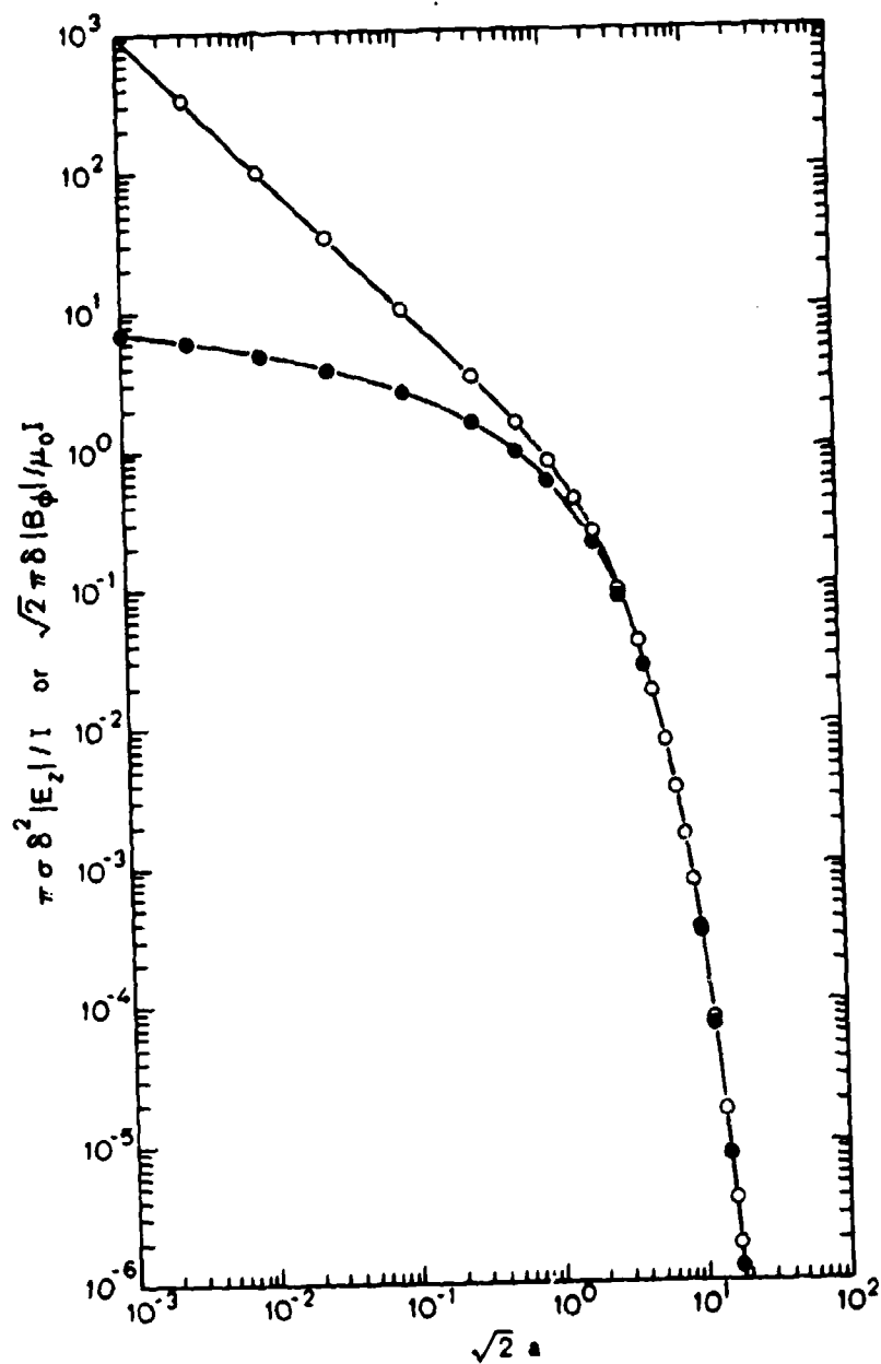
Figure IV.4. Variation with parametric distance \sqrt{2} a (where a = \rho \delta = \rho / \delta ) of the parametric expressions for the amplitude of the electric field (crossed circles) and the magnetic field (dotted circles) produced in a conducting medium of infinite extent by a linear current source of infinite length carrying an alternating current of amplitude 1.
