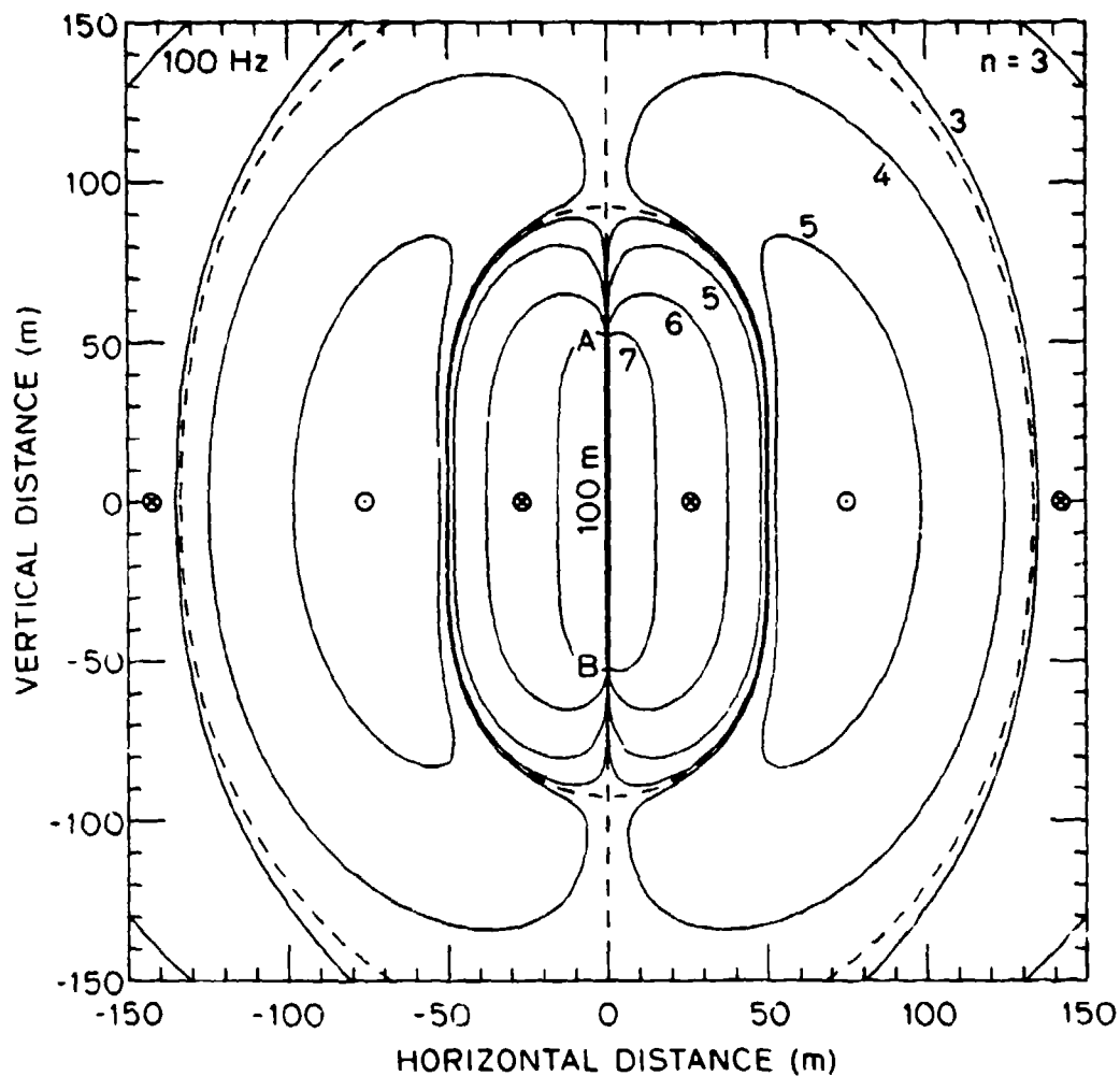
Figure III.4. Variation of the total magnetic field (which has only the one component B_\phi ) produced in sea water by a linear current source of finite length (100 m) carrying an alternating current of amplitude 1000 A and frequency 100 Hz at the time instant when there is maximum current flowing in the direction from B to A. The magnetic field magnitudes are given by B_\phi = 10^n pT, where n is given for each contour in the figure ( B_\phi = 0 on the dashed contours.) As indicated, the direction of B_\phi is either into the paper or out of the paper depending on the region between the dashed lines. The field pattern is cylindrically symmetric around the axis of the source.
