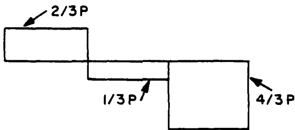
Fig. 6 - Shear diagram
