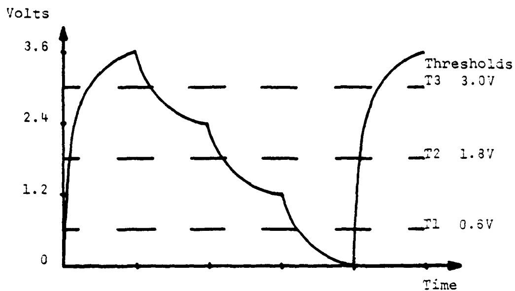
Fig. A.17. Amplitude Decision Circuit Input Levels
