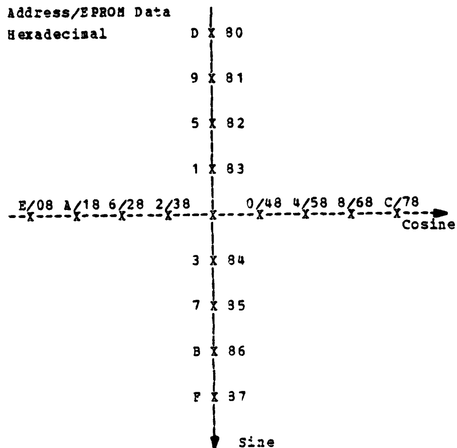
Fig. B.4. Phase Plane Codes - Case 0
