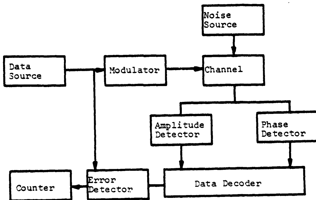
Fig. 4.3. Experimental System
