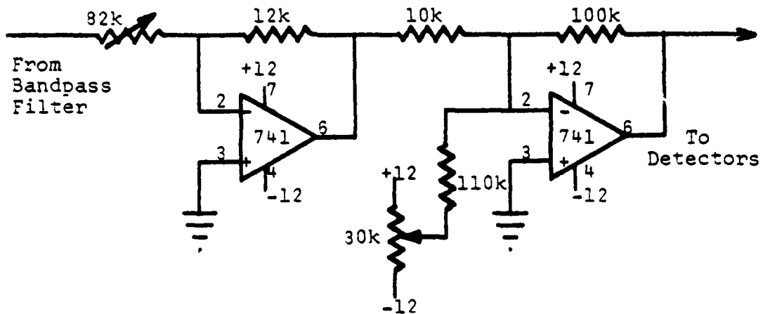
Fig. A.11. Predetection Amplifier Circuit Diagram
