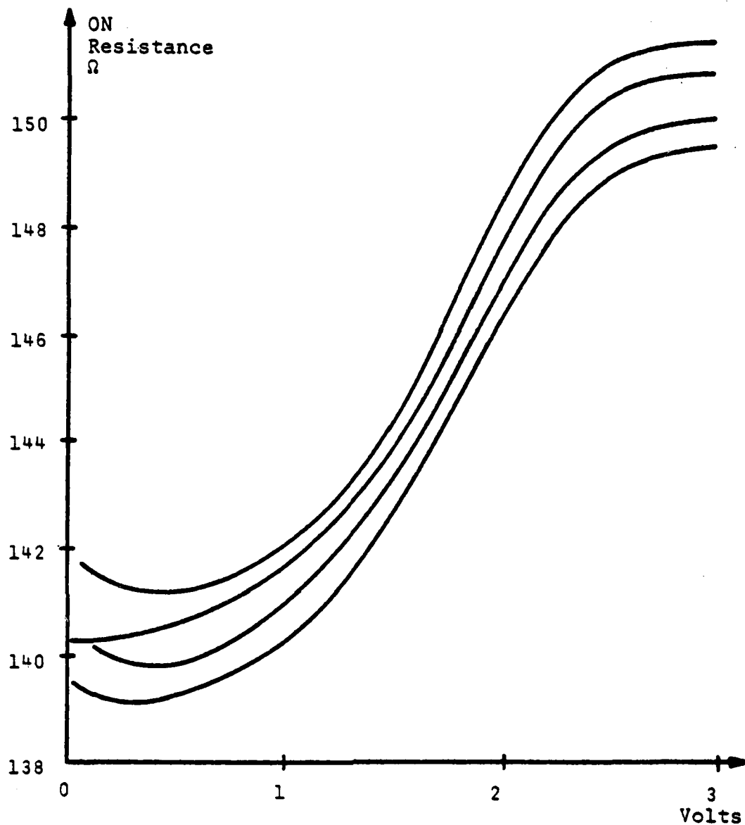
Fig. 2.2. ON Resistance of the 4051 Switches
