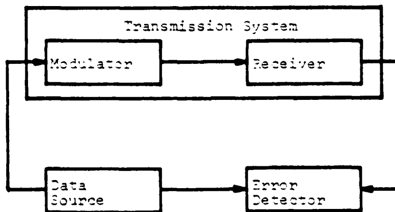
Fig. A.31. Test System Block Diagram
