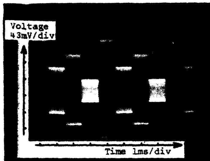
Figure A.9. General Analog Multiplexer Modulator Output - Periodic Data
