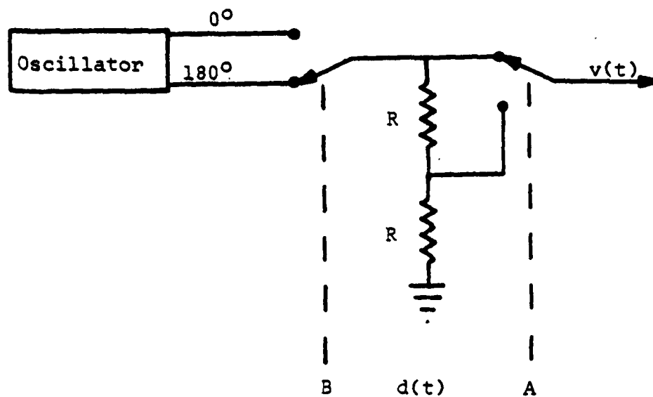
Fig. 1.3. 2-Phase, 2-Amplitude Modulator Circuit Diagram
