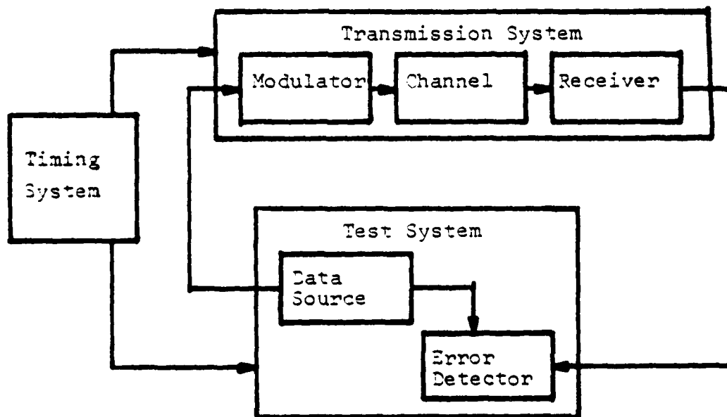
Fig. A.1. Experimental System Block Diagram
