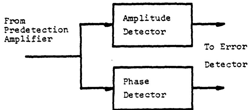
Fig. A.12. Receiver Block Diagram
