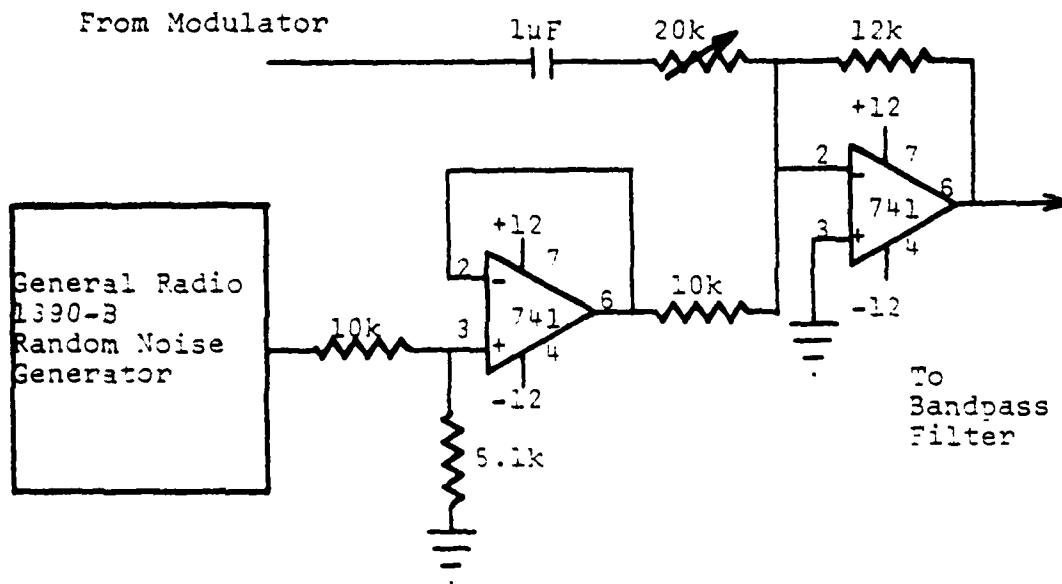
Fig. A.4. Noise Summer Circuit Diagram
