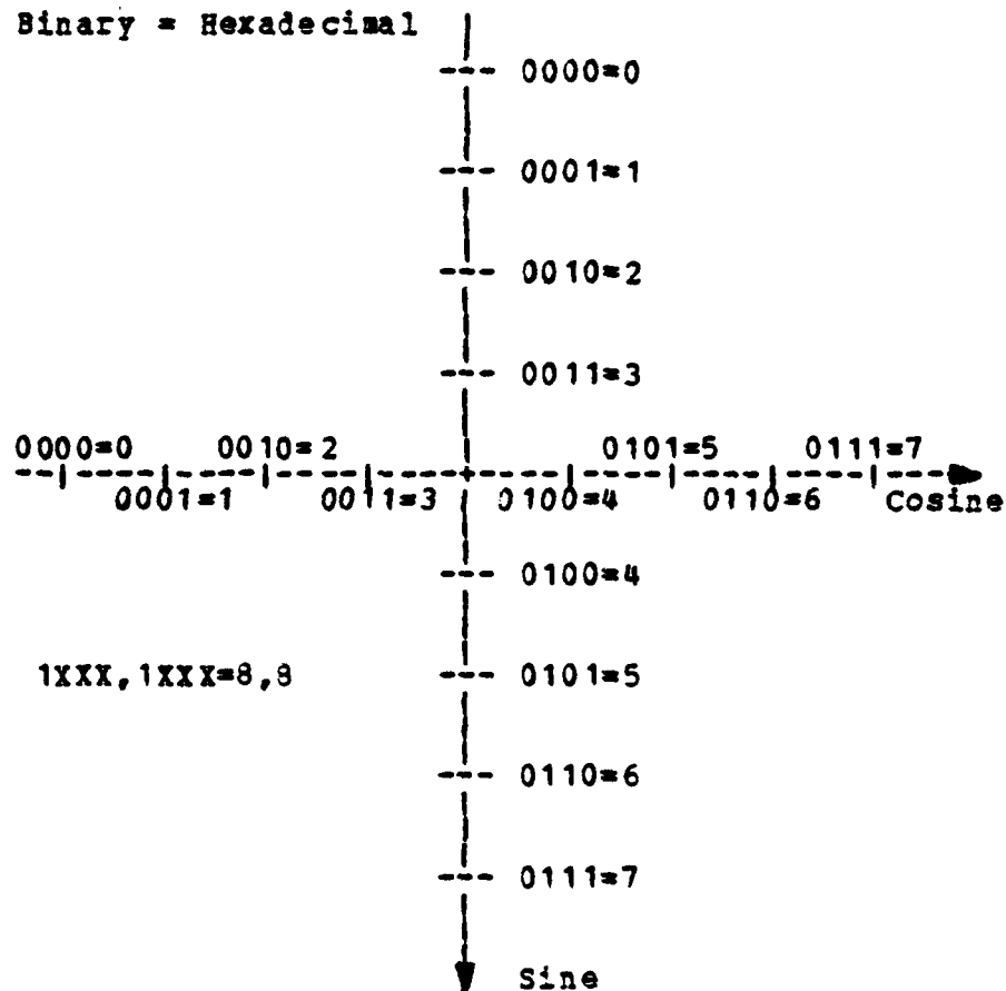
Fig. B.2. Multiplexer Control Codes
