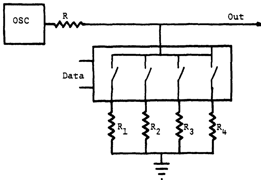
Fig. 3.5. Amplitude Modulator Block Diagram
