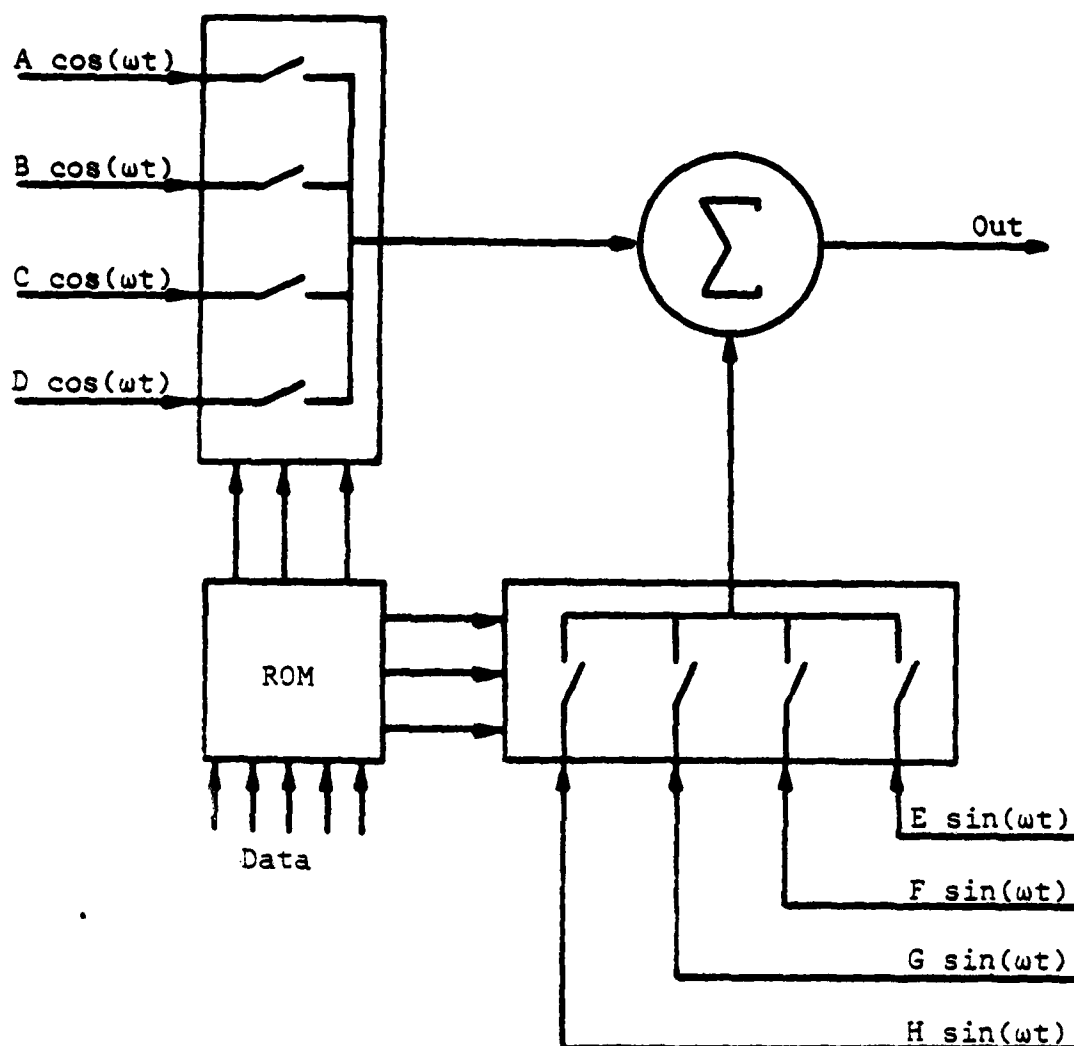
Figure 3.12. General Analog Multiplexer Modulator Block Diagram
