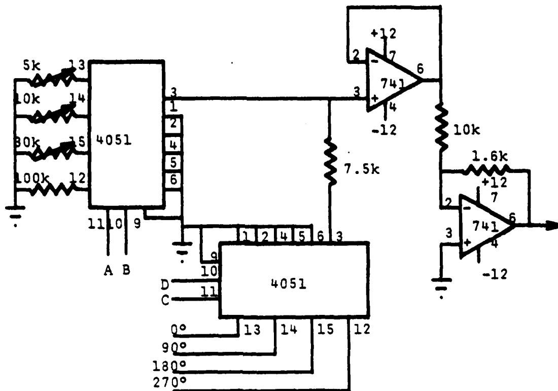
Fig. 3.11. 4-Phase, 4-Amplitude Modulator Circuit Diagram
