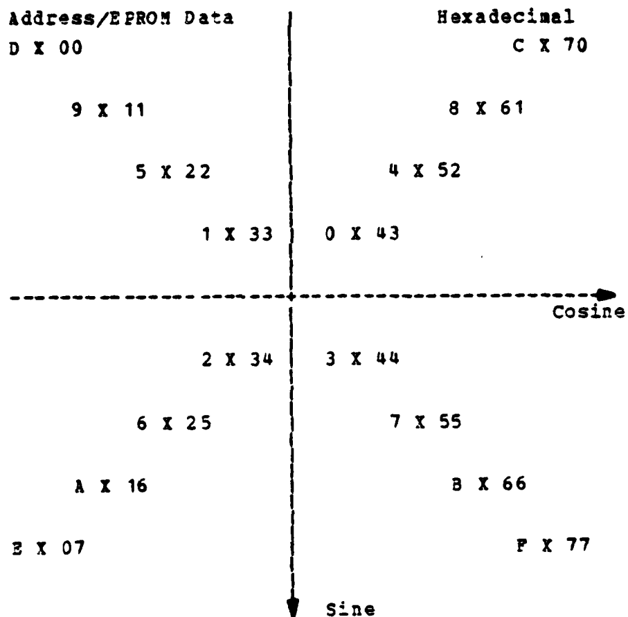
Fig. B.5. Phase Plane Codes - Case 1
