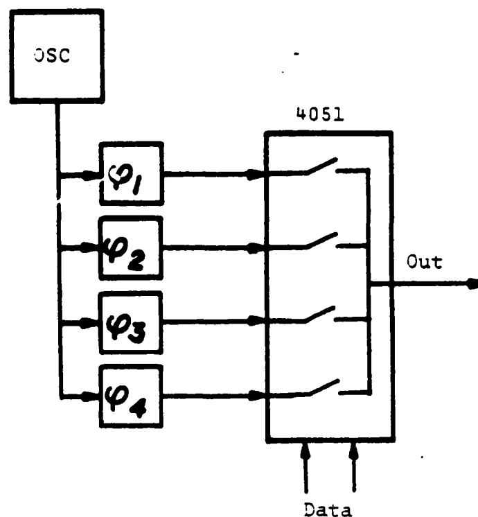
Fig. 3.1. Phase Modulator Block Diagram
