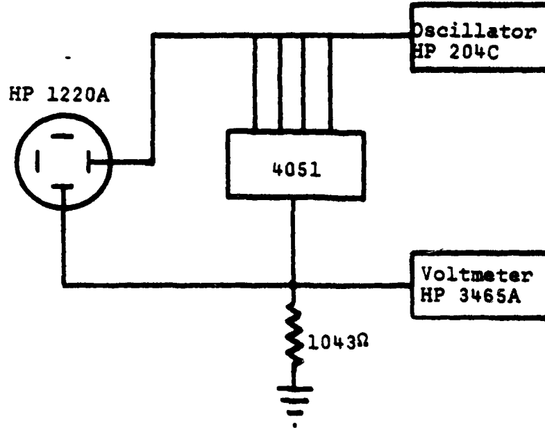
Fig. 2.1. ON Resistance Test Circuit
