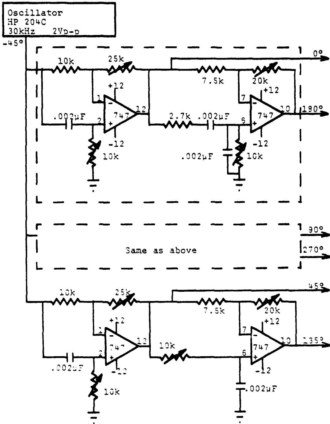
Fig. A.29. Multi-Phase Source Circuit Diagram
