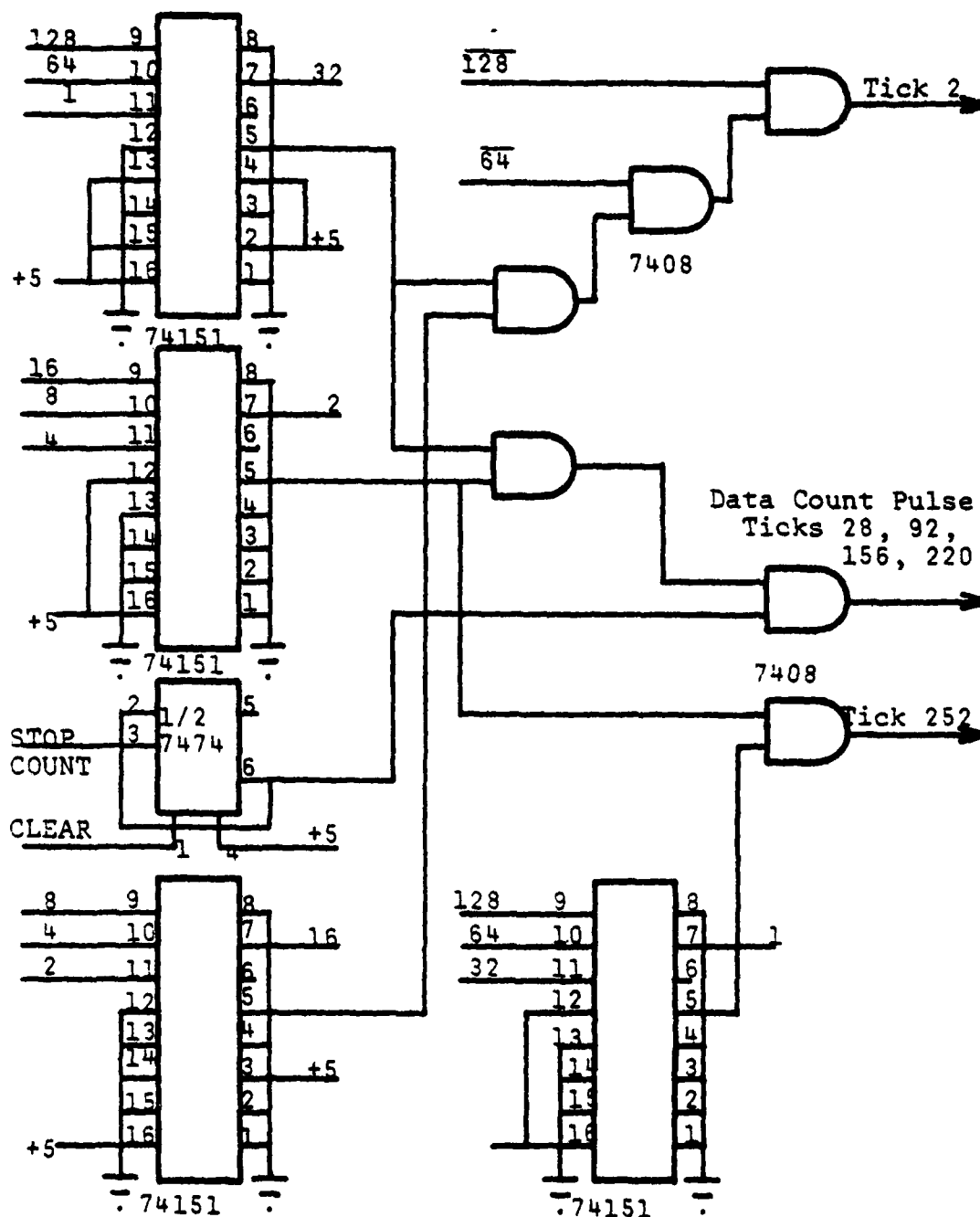
Fig. A.41. Pulse Generator Combinational Logic
