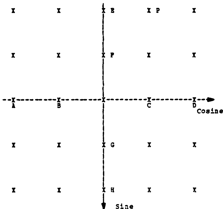
Figure 3.13. General Analog Multiplexer Modulator Phase-Plane Diagram
