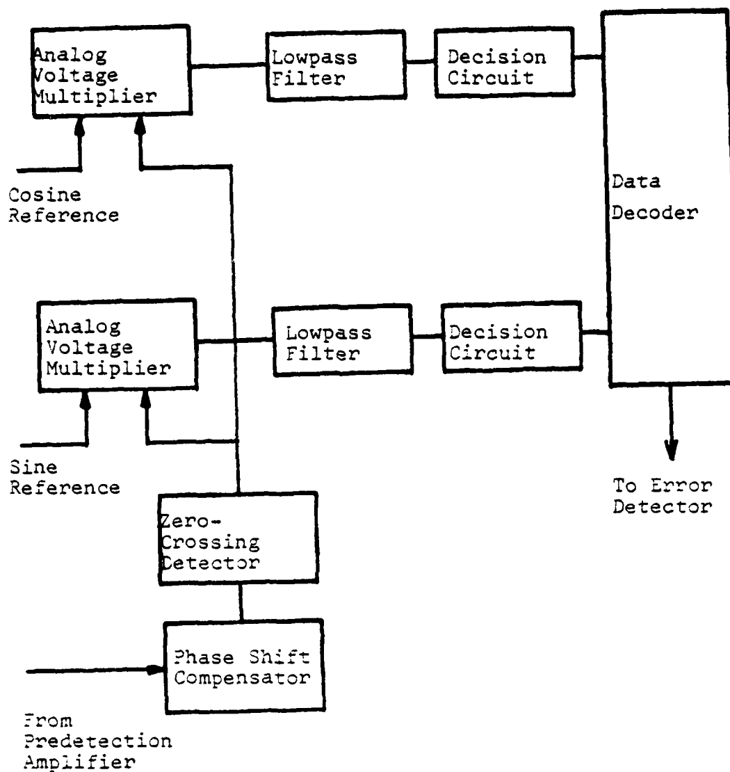
Fig. A.21. Phase Detector Block Diagram
