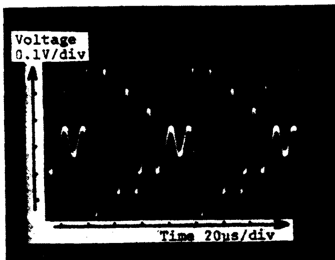
Fig. 3.9. 4-Phase, 4-Amplitude Modulator Output - 10 kHz
