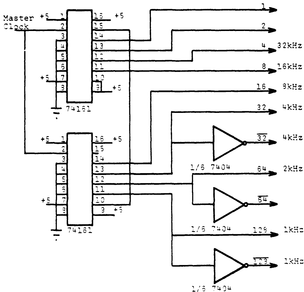
Fig. A.40. Clock Divider Circuit Diagram
