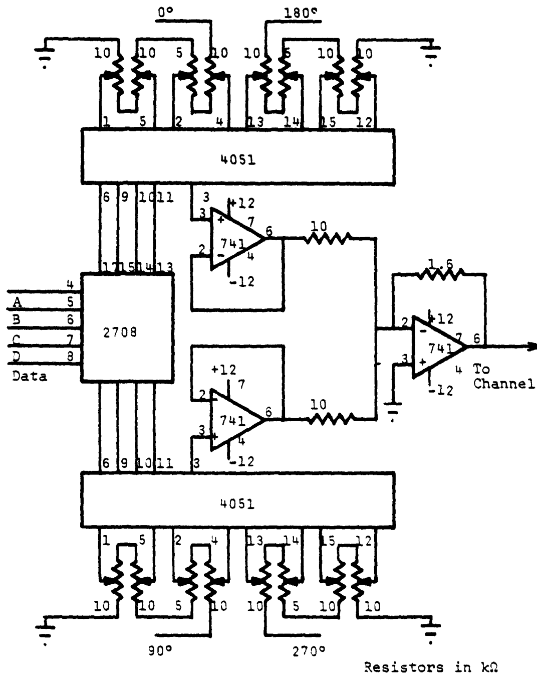
Figure 3.14. General Analog Multiplexer Modulator Circuit Diagram
