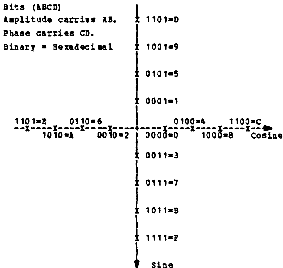
Fig. B.1. Phase Plane Address Codes
