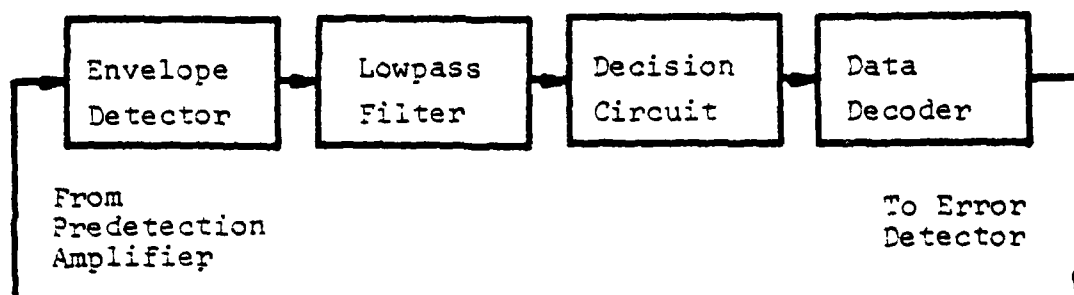
Fig. A.13. Amplitude Detector Block Diagram
