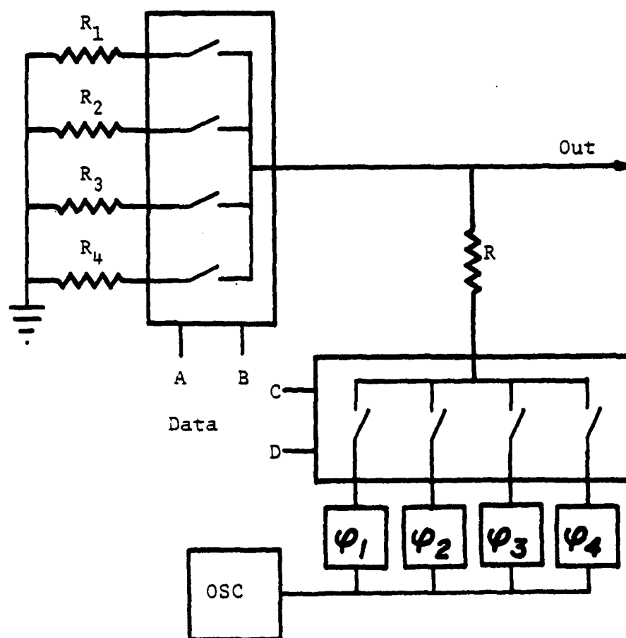
Fig. 3.8. 4-Phase, 4-Amplitude Modulator Block Diagram
