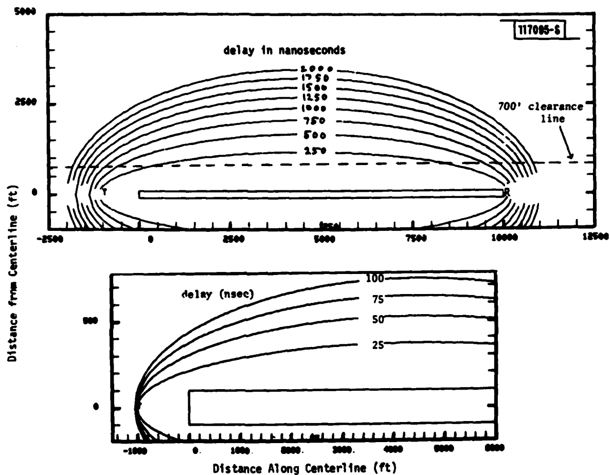
Fig.1-2. Constant delay contours on airport surface.
