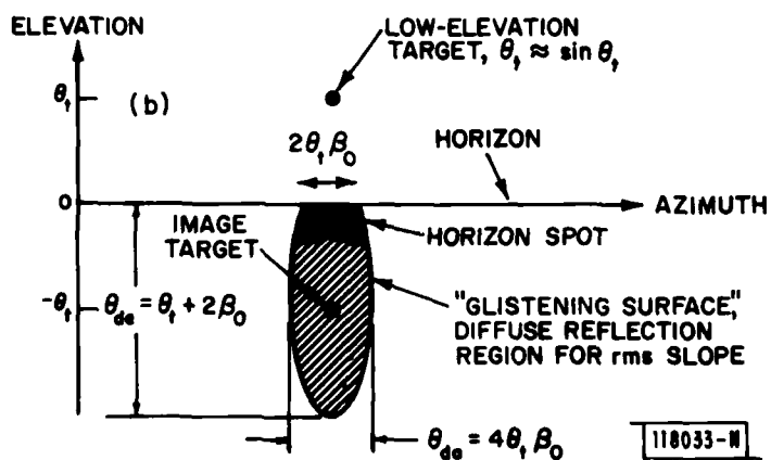
Fig.3-5. Diffuse multipath level and spatial distribution: (a) specular and diffuse scattering coefficient vs. roughness factor and (b) angular extent of glistening surface for rough surface scattering.
