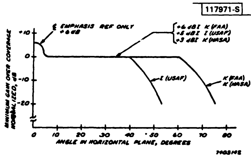
Fig.2-9. Hazeltine AZ antenna azimuth pattern showing centerline emphasis.
