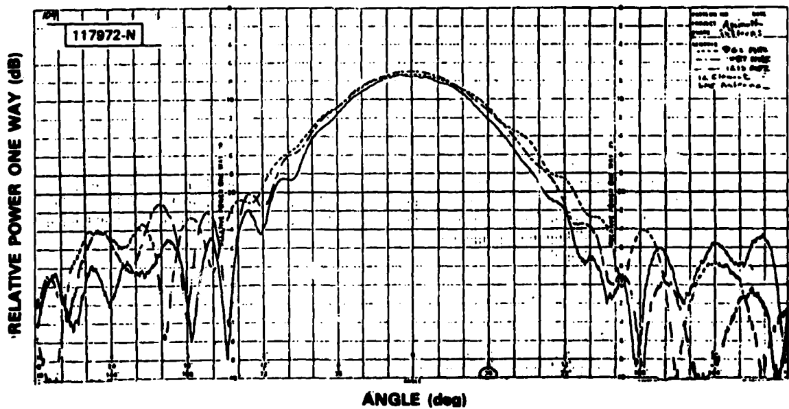
Fig.2-10. Measured horizontal pattern of ground antenna (from [37]).
