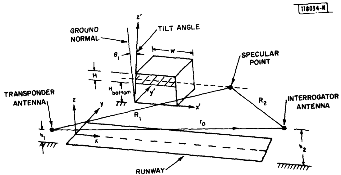
Fig.3-6. Configuration used to determine multipath parameters due to scattering from building.
