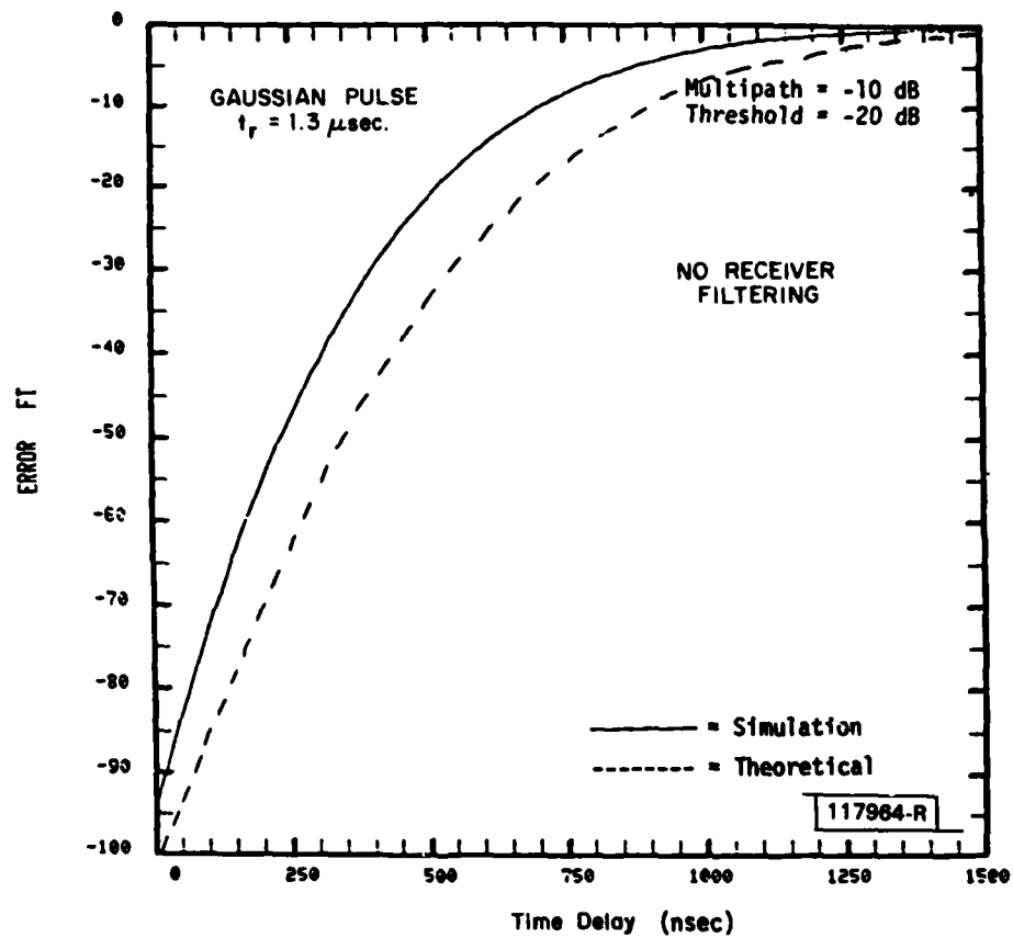
Fig.2-3. Fixed thresholding error vs. multipath delay.
