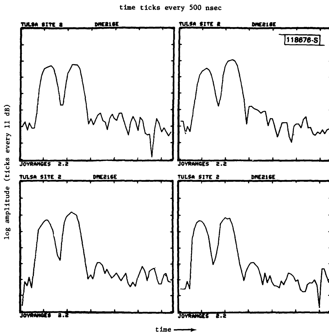
Fig.5-25. Tulsa site 2 waveforms near threshold.
