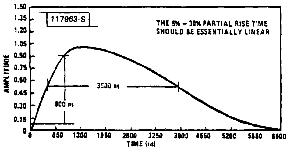
Fig.2-2. DME/P \cos-\cos^2 waveform.
