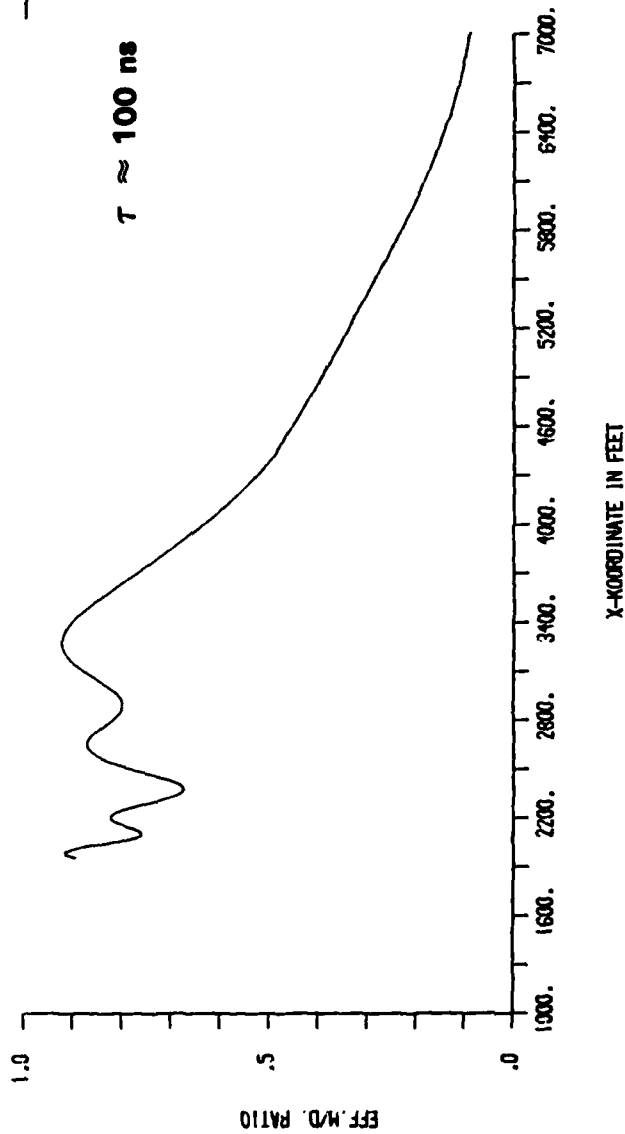
Fig. 4-28(b). Effective M/D ratio for Building #1 in AWOP scenario 3 (from [42]).
