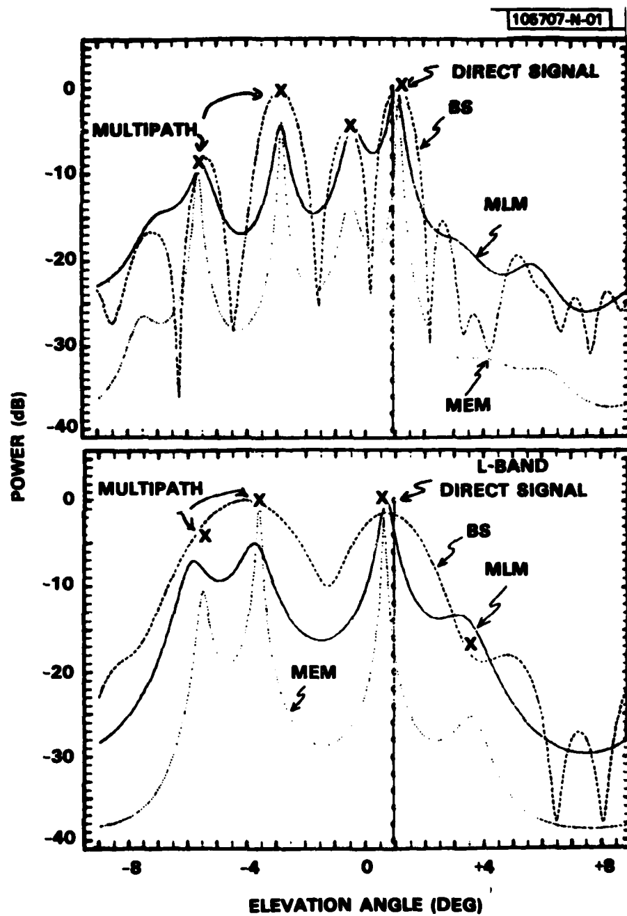
Fig.7-3. Received power vs. elevation angle at Camp Edwards site #2.
