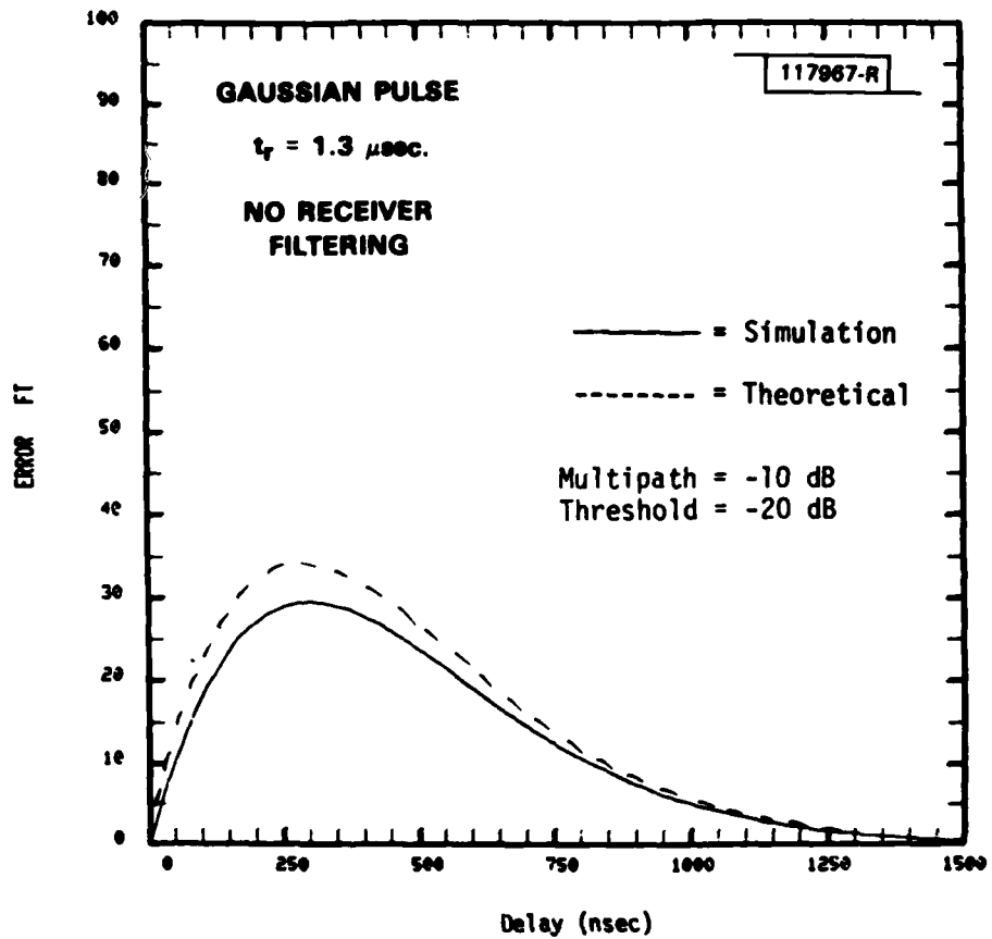
Fig.2-6. Delay-and-compare error vs. multipath delay.
