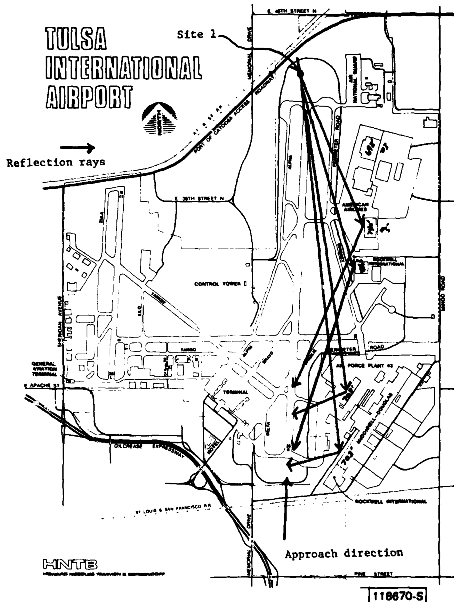
Fig.5-20. Tulsa site 1 measurement geometry and reflection rays.
