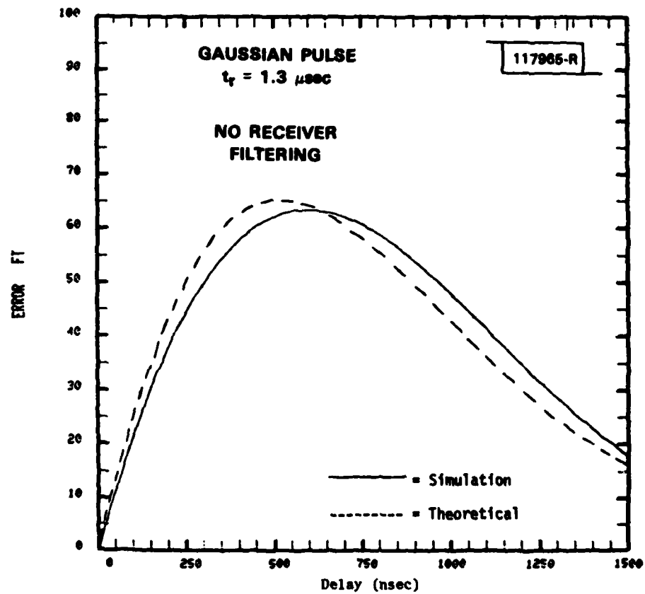
Fig.2-4. Adaptive thresholding error vs. multipath delay.
