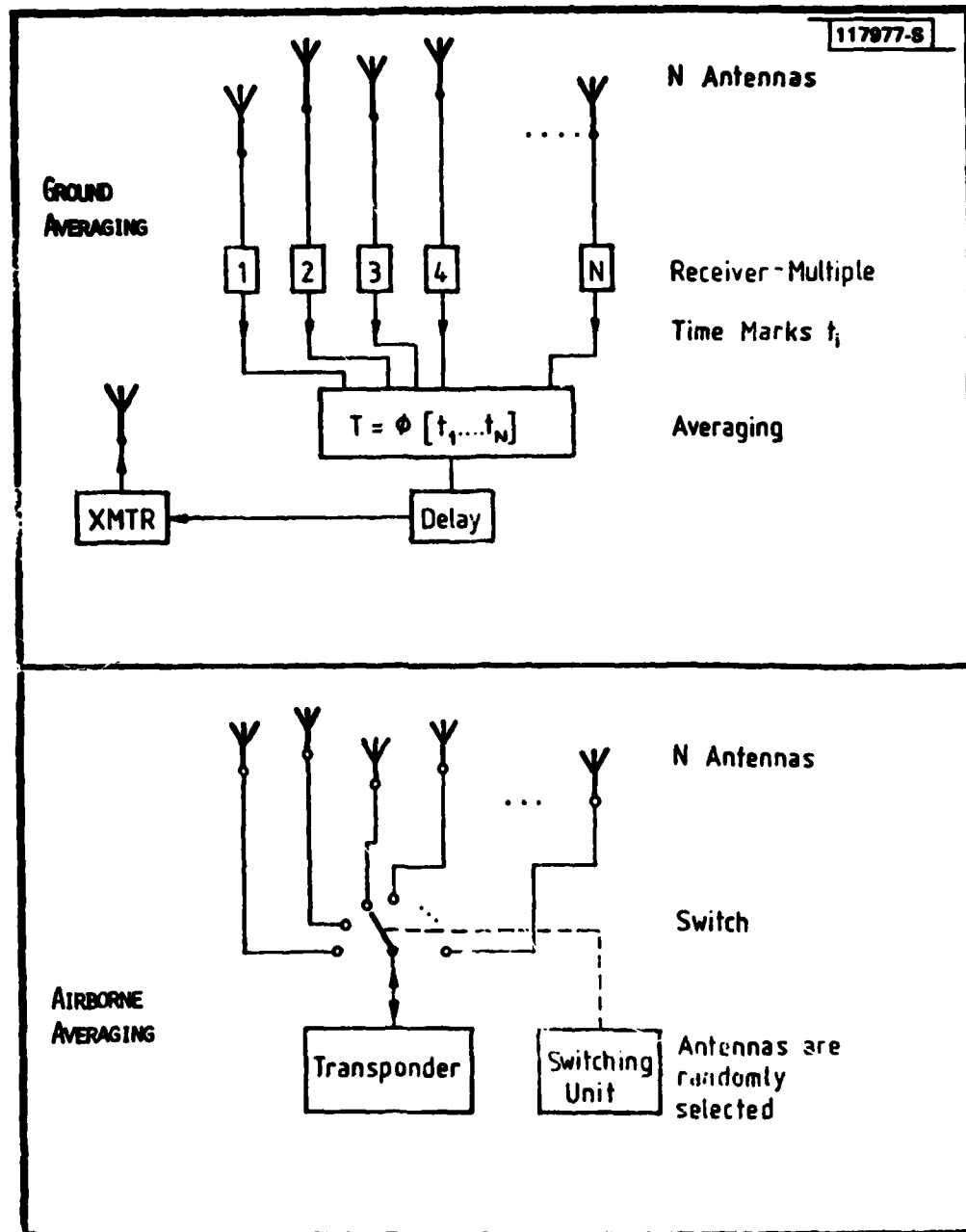
Fig.2-14. Lateral diversity DME/P transponder.
