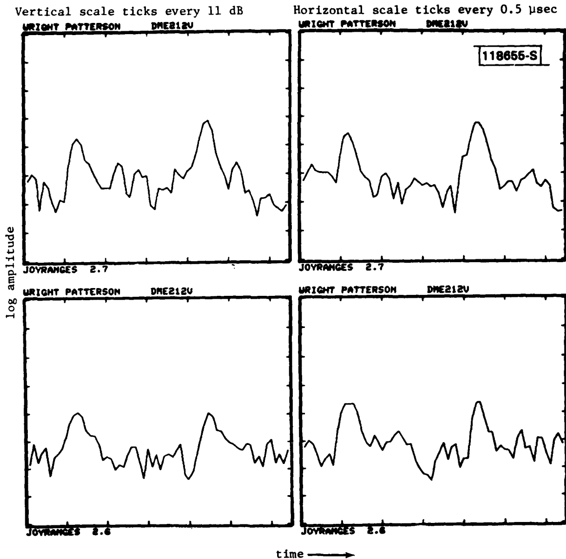
Fig.5-9. WPAFB waveforms near threshold.
