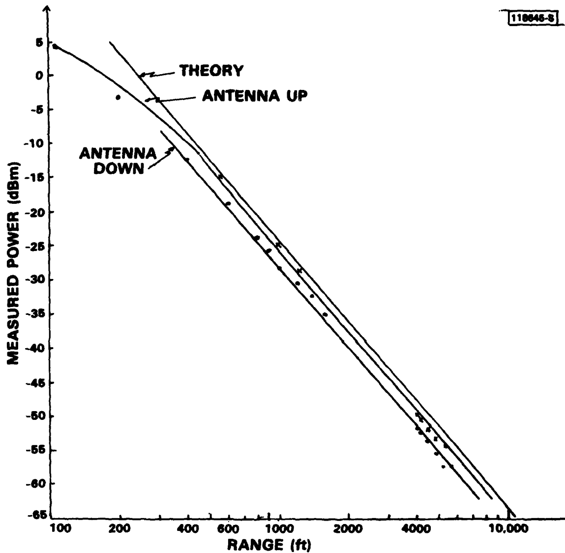
Fig.5-1. Measured signal level along Hanscom taxiway with both antennas at 5 feet, dipole pointed down (from McGarty [22]).
