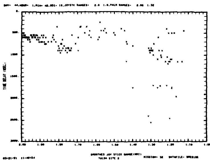
Fig.5-26(b). Tulsa site 2 data summary for 50 ft. threshold crossing height.
