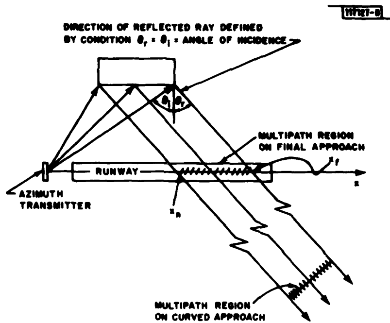
Fig.6-1. Determination of MLS multipath by ray tracing.
