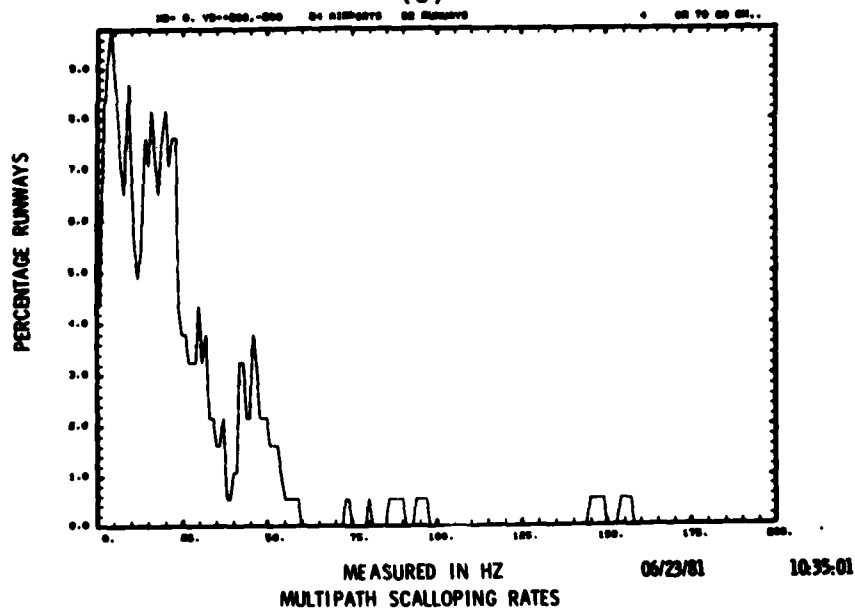
Fig.6-7. Distribution of scalloping frequencies when DME/P is sited with azimuth transmitter building: (a) buildings near threshold and (b) buildings near runway stop end.
