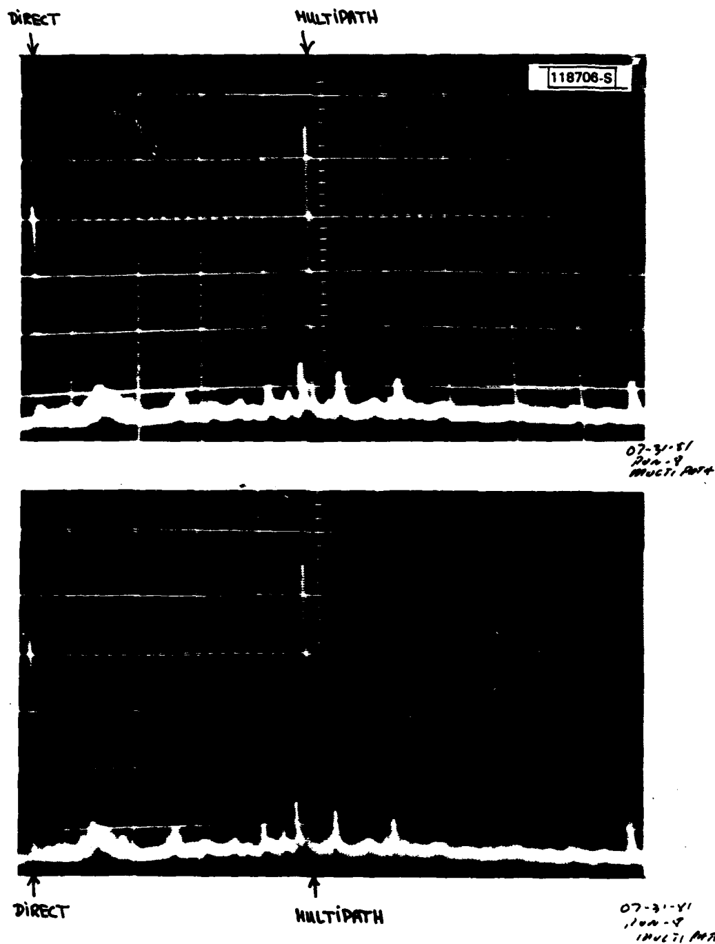
Fig.5-54. Site 2 multipath near 125 ft. altitude.
