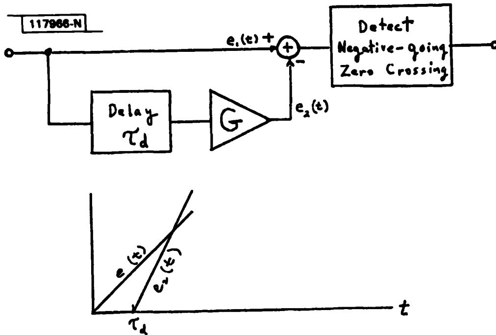
Fig.2-5. DME leading edge comparator circuit.
