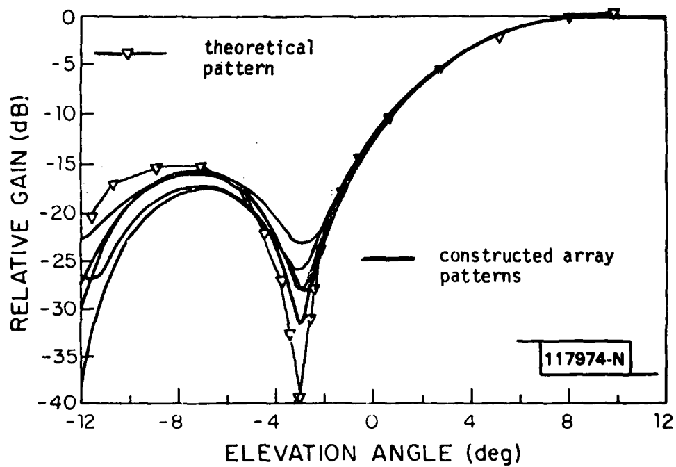
Fig.2-11(b). Patterns of five PALM elements.
