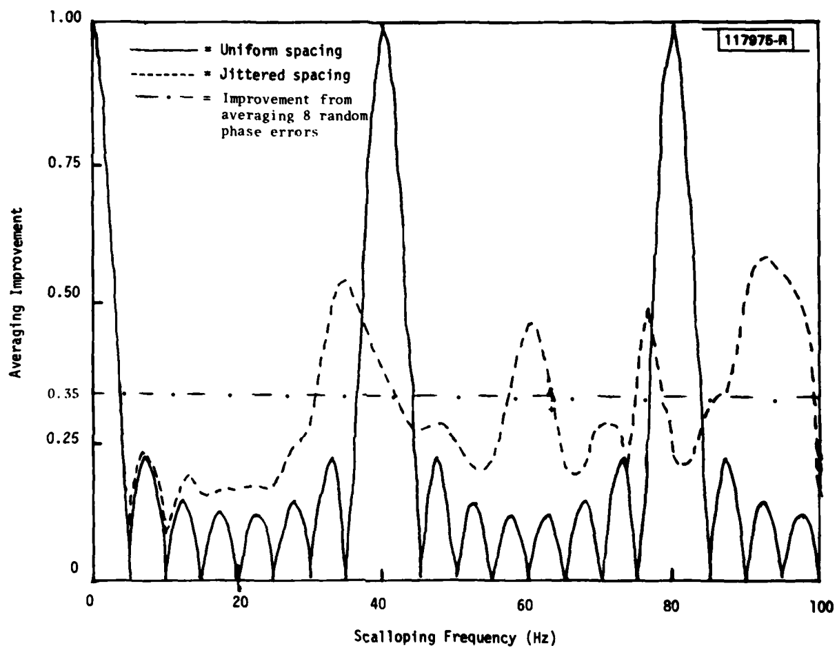
Fig.2-12. Averaging factor for uniform and jittered spacing (TRSB).
