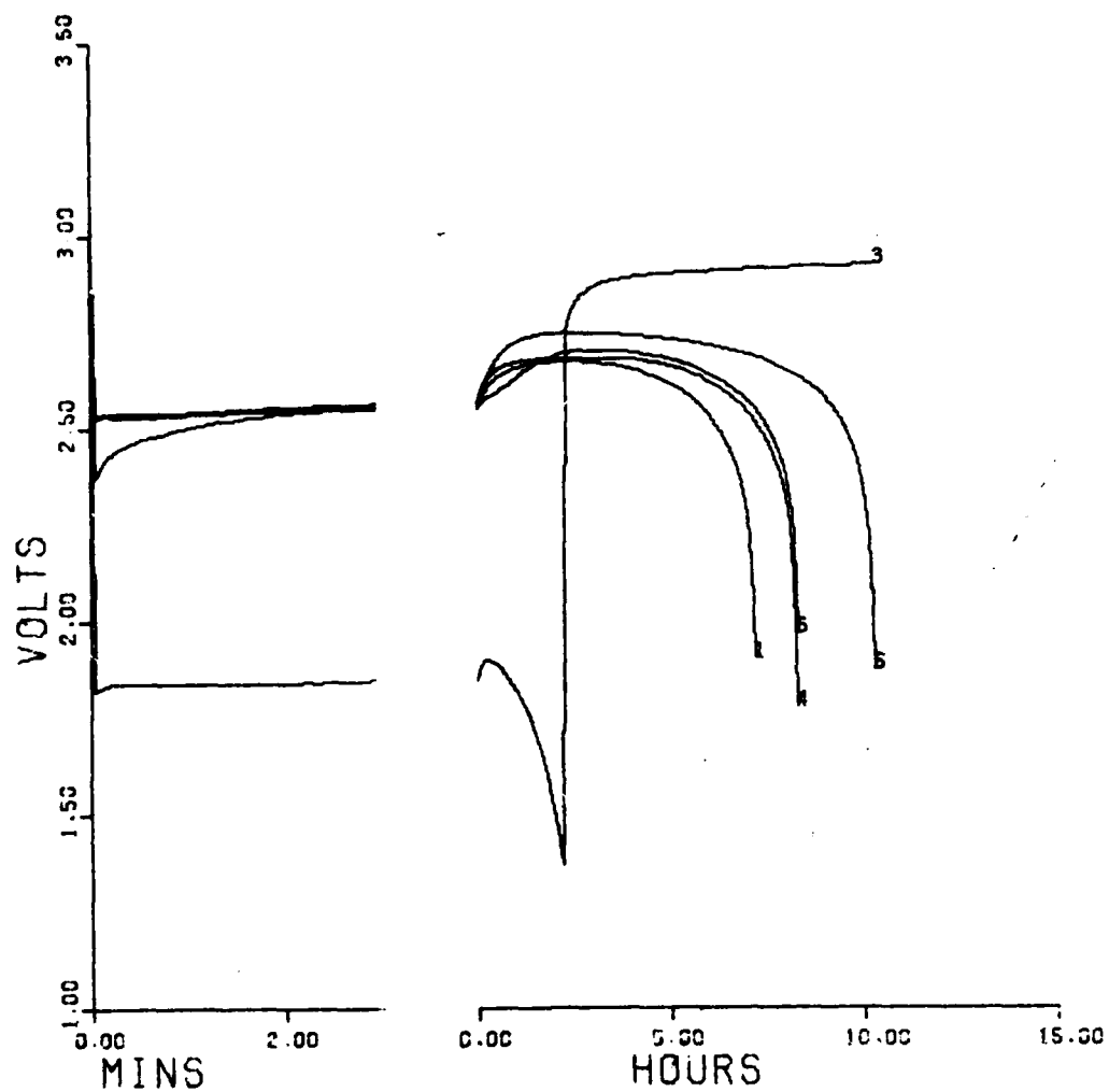
Figure C-16. Computer Plot - HW .6D LI-SO2 Cells HTS: 9 Months: 300 MA DISCH At 70 F
