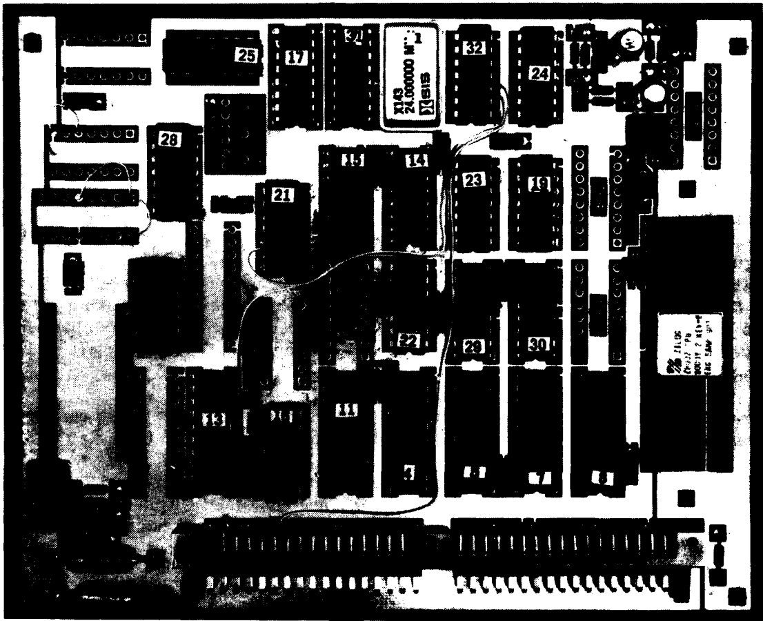
Figure 9. CPU Brassboard
