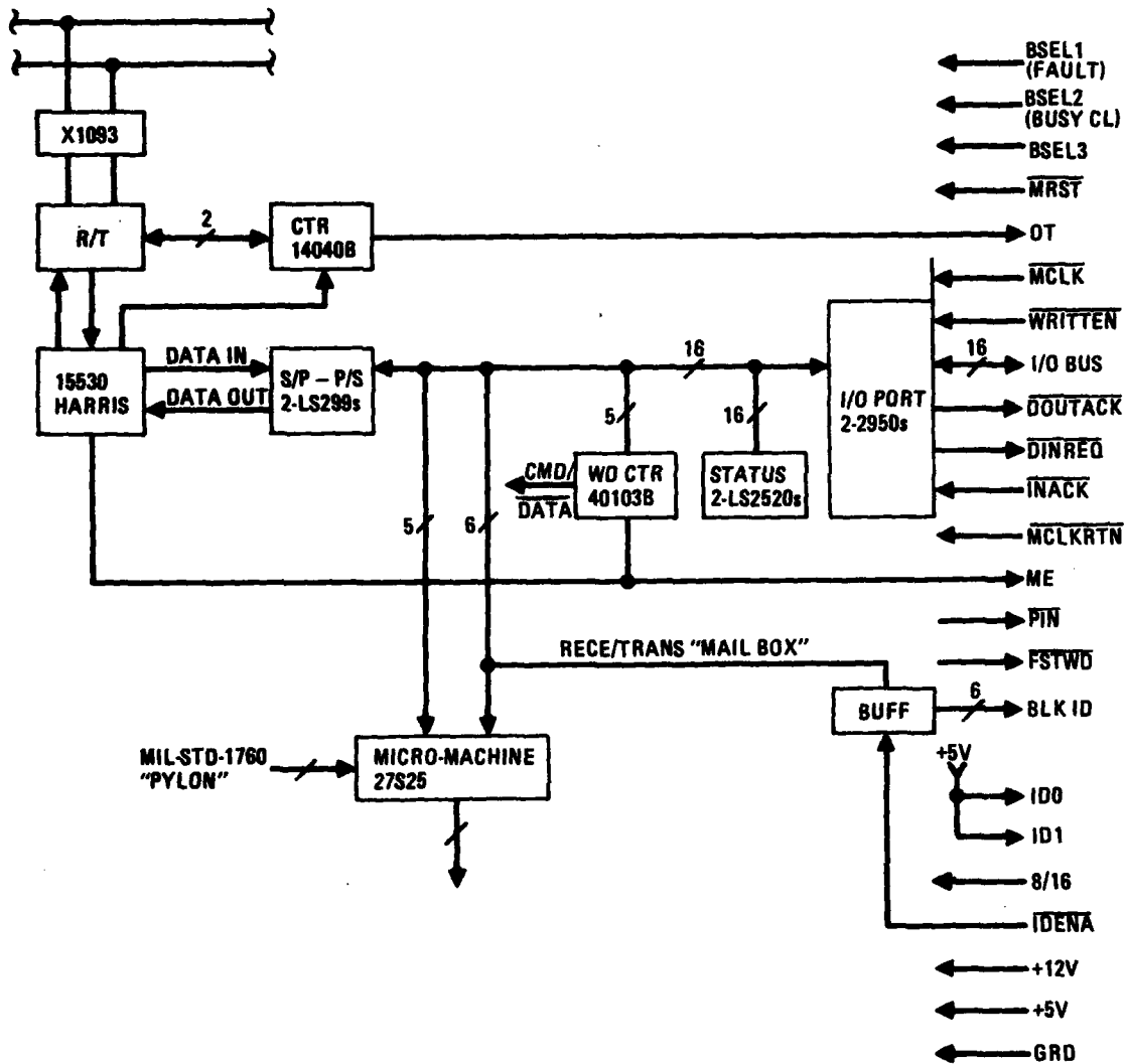
Figure 32. Single Channel 1553B I/O Card Block Diagram
