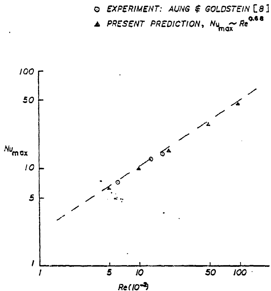
Figure 46. Variation of Maximum (Peak) Nusselt Number with Reynolds Number Downstream of Back-Step
