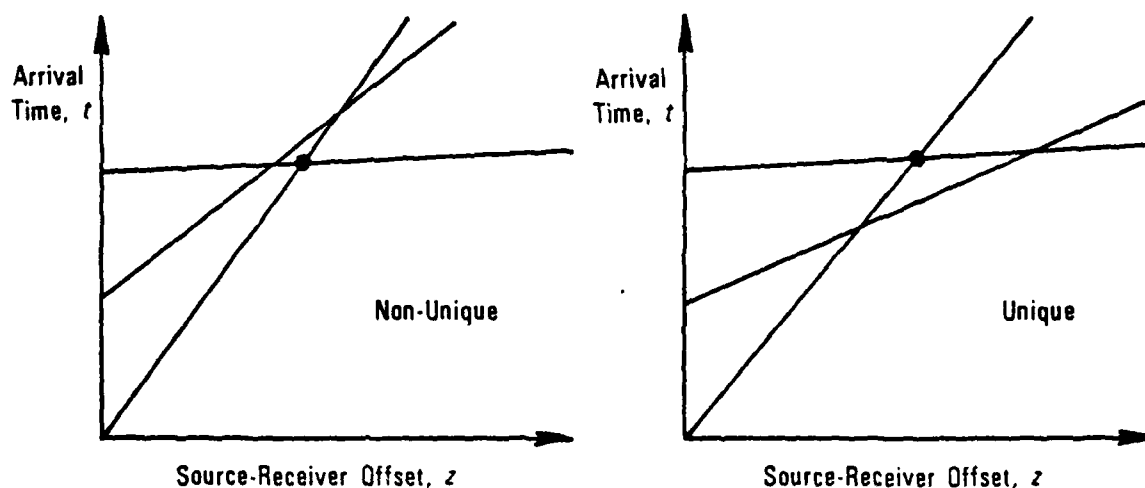
Figure 2-6. Non-uniqueness of first-arrival-time inversion
