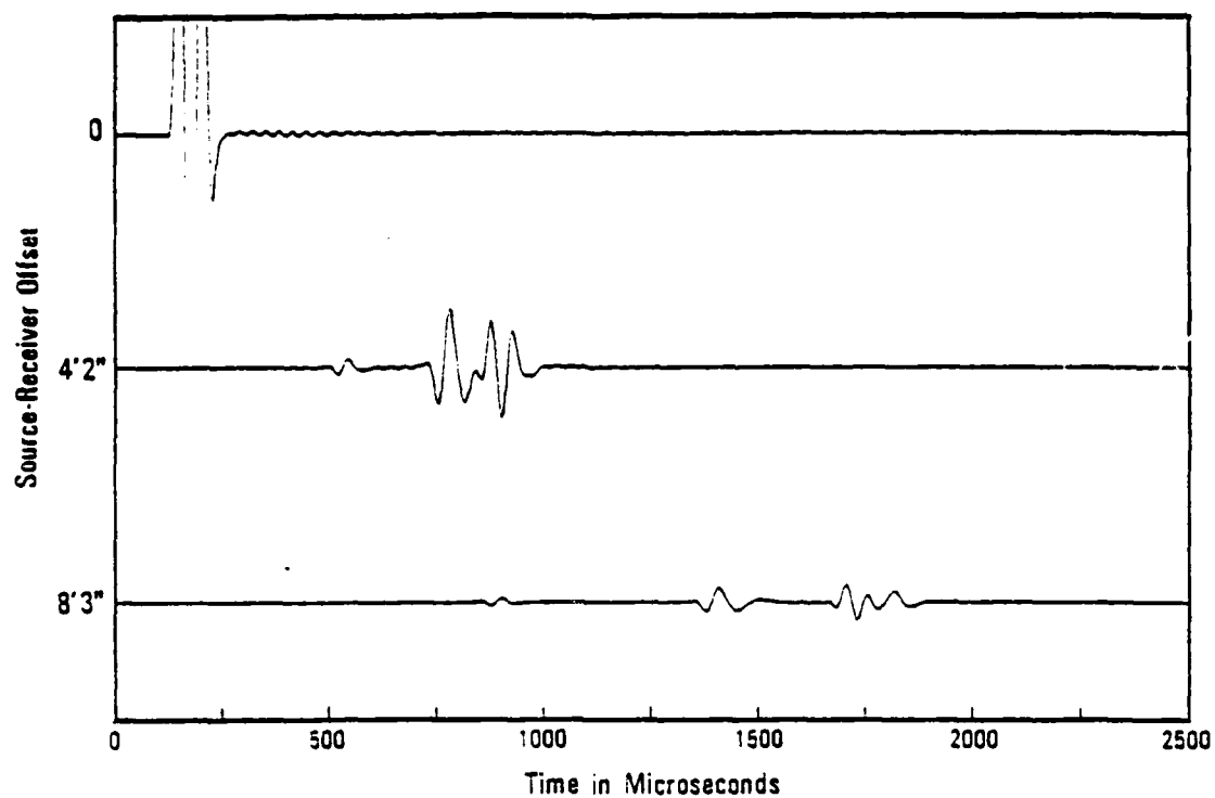
Figure 2-13. The primary reflection at three source-receiver offsets
