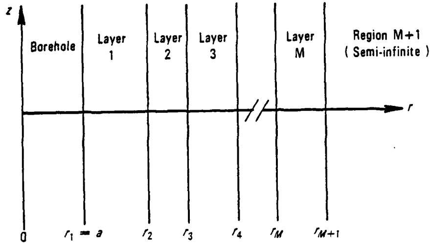
Figure 4-6. The cylindrically layered liquid formation geometry
