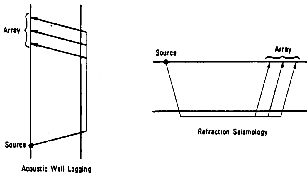
Figure 1-9. The analogy between acoustic logging and refraction seismology
