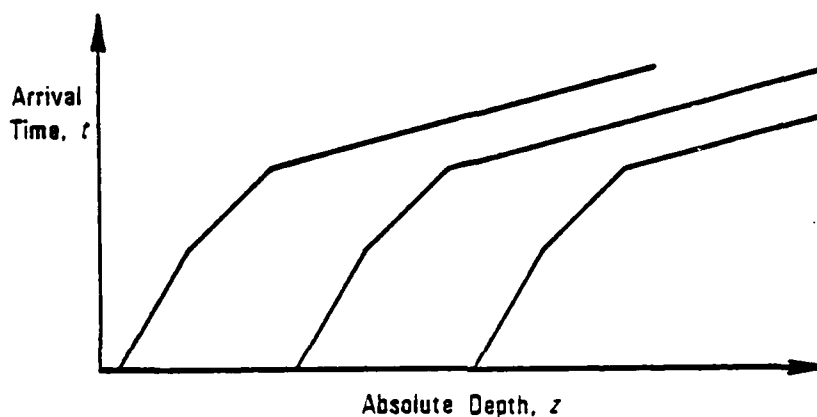
Figure 2-7. First-arrival-time curves associated with different source shots
