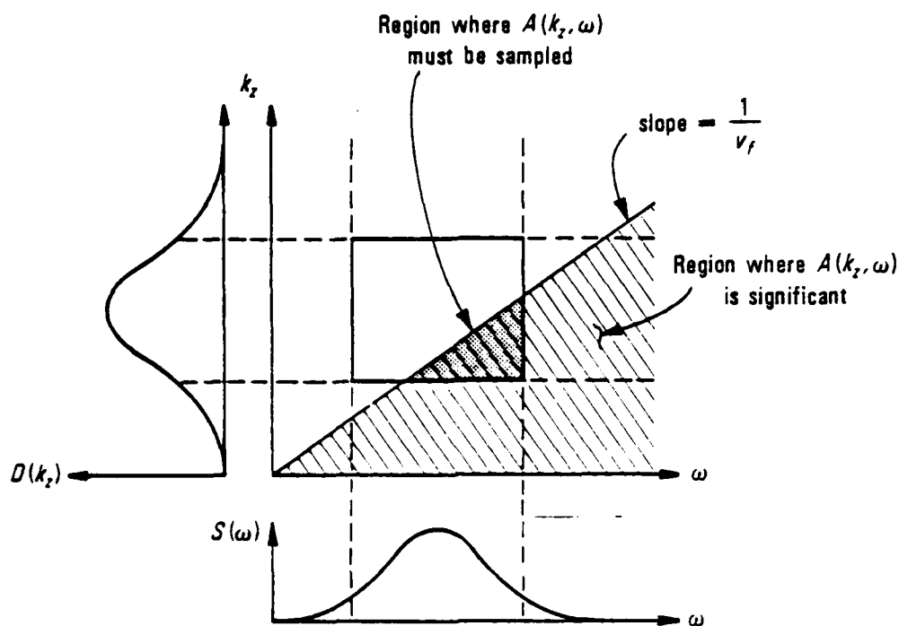
Figure 4-1. The region of integration
