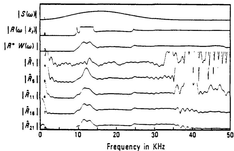
Figure 6-14 Experiment 2. Reflection coefficient estimates. Infinite array no noise added, 38 dB SNR
