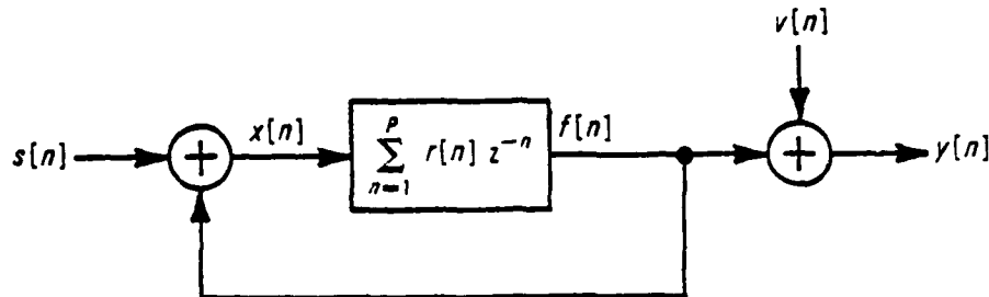
Figure 6-2. The discrete time dereverberation system
