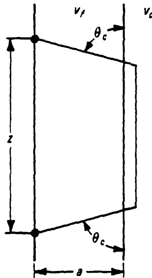
Figure 2-2. The least-time ray
