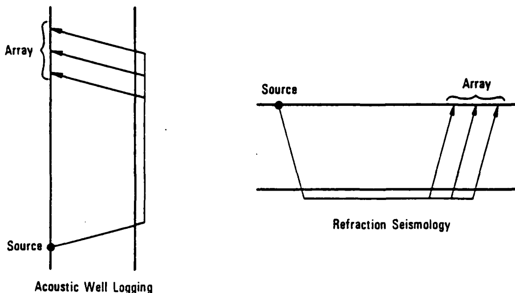
Figure 2-3. Planar and cylindrical geometry analogs
