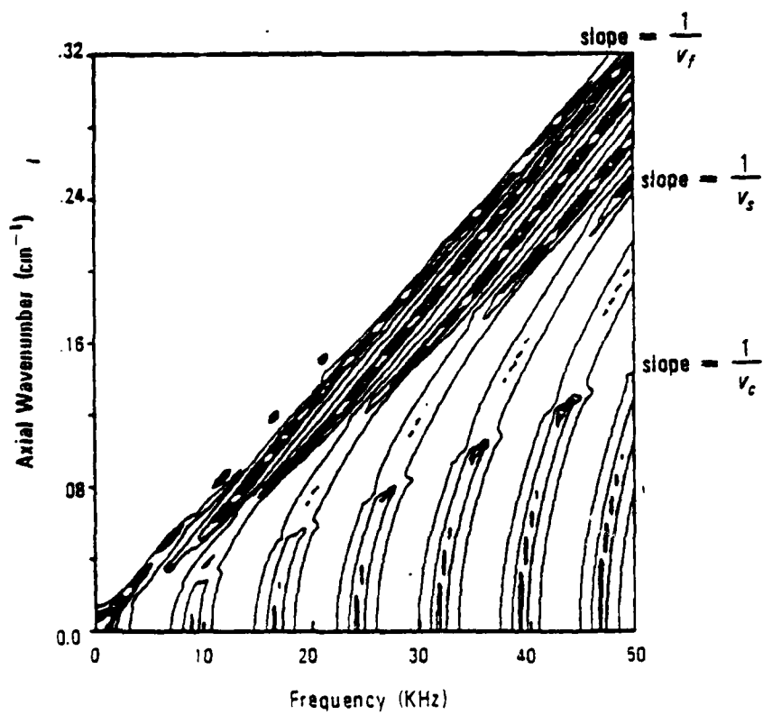
Figure 1-4. The magnitude of the cylindrical wave modal coefficient
