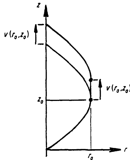
Figure 2-12. A migration interpretation of travel-time inversion
