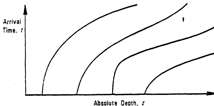
Figure 2-11. First-arrival-time curves for a heterogeneous formation model
