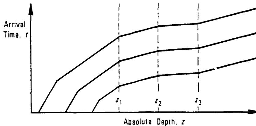
Figure 2-10. First-arrival-time curves for successive source shots
