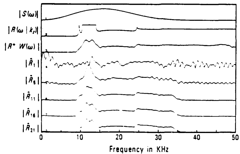
Figure 6-15 Experiment 3. Reflection coefficient estimates. Infinite array no noise added, 18 dB SNR
