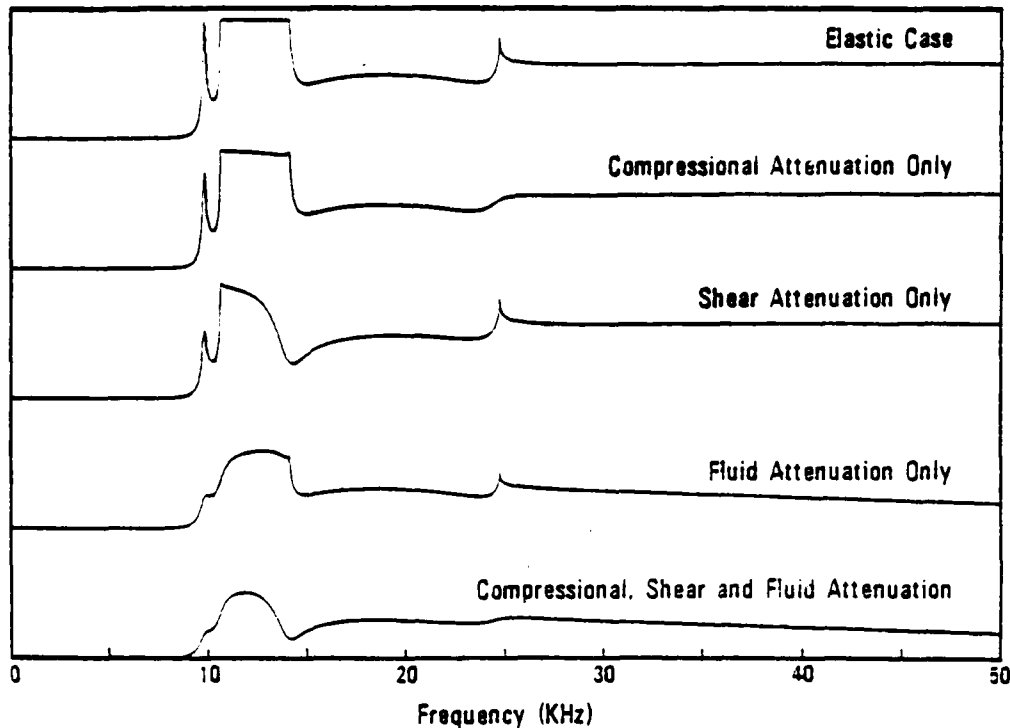
Figure 2-18. A slice of the reflection coefficient and sensitivity to attenuation
