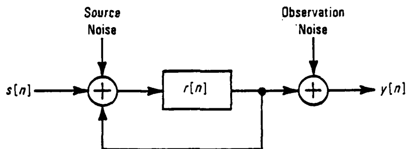
Figure 1-8. The discrete domain dereverberation signal processing model
