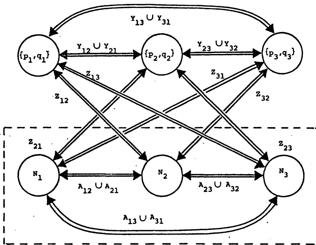
(a) \tilde{G} = (\tilde{N}, \tilde{A})
