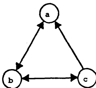
(a) G = (N, A)
