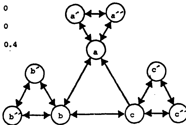
(b) \tilde{G} = (\tilde{N}, \tilde{A})
