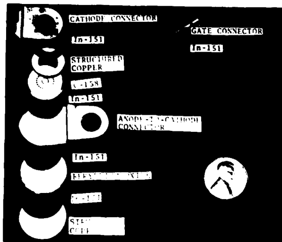
Figure 6. Subassembly Parts
