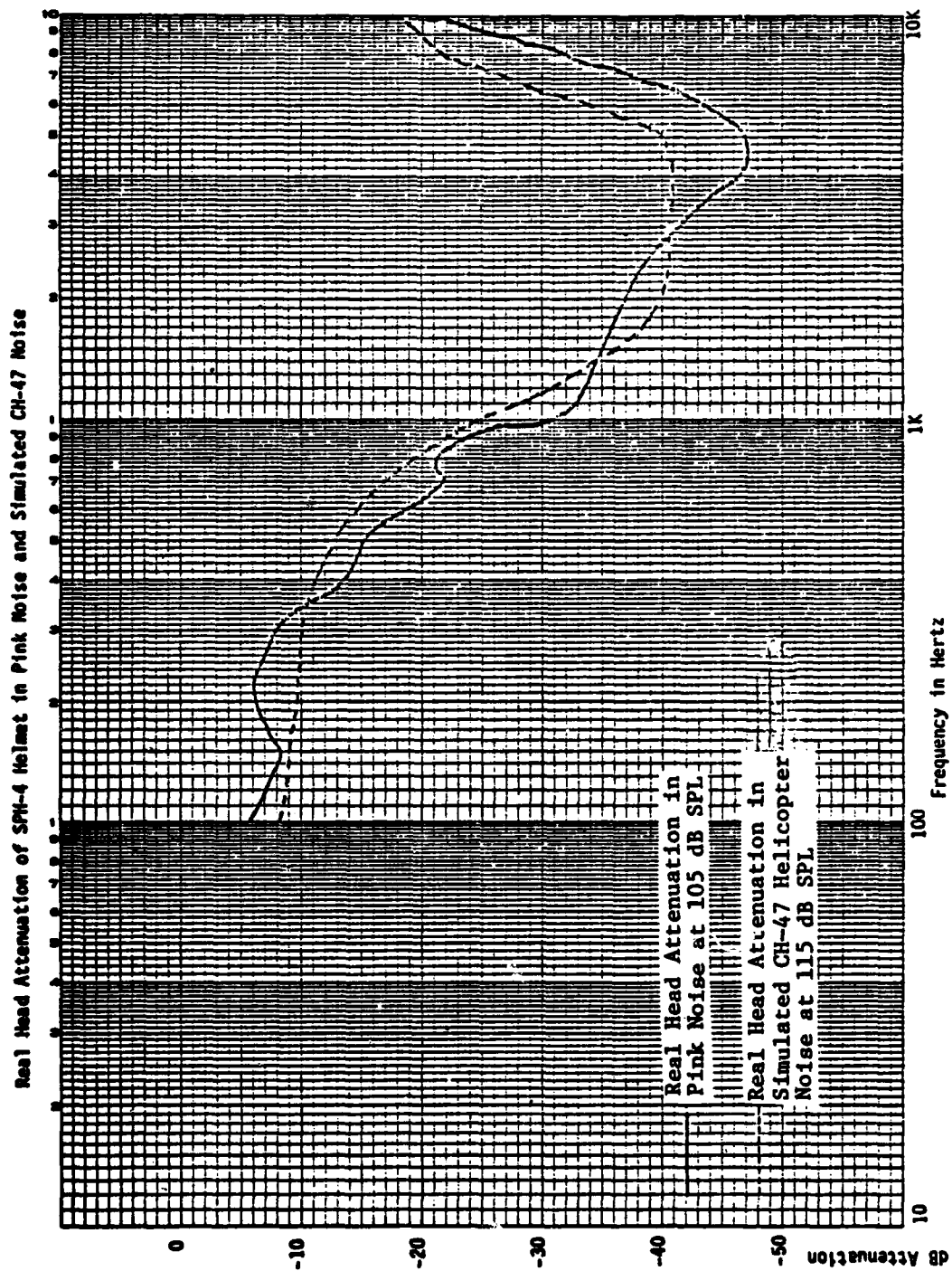
Figure 3. Real Head Attenuation of SPH-4 Helmet in Pink Noise and Simulated CH-47 Noise
