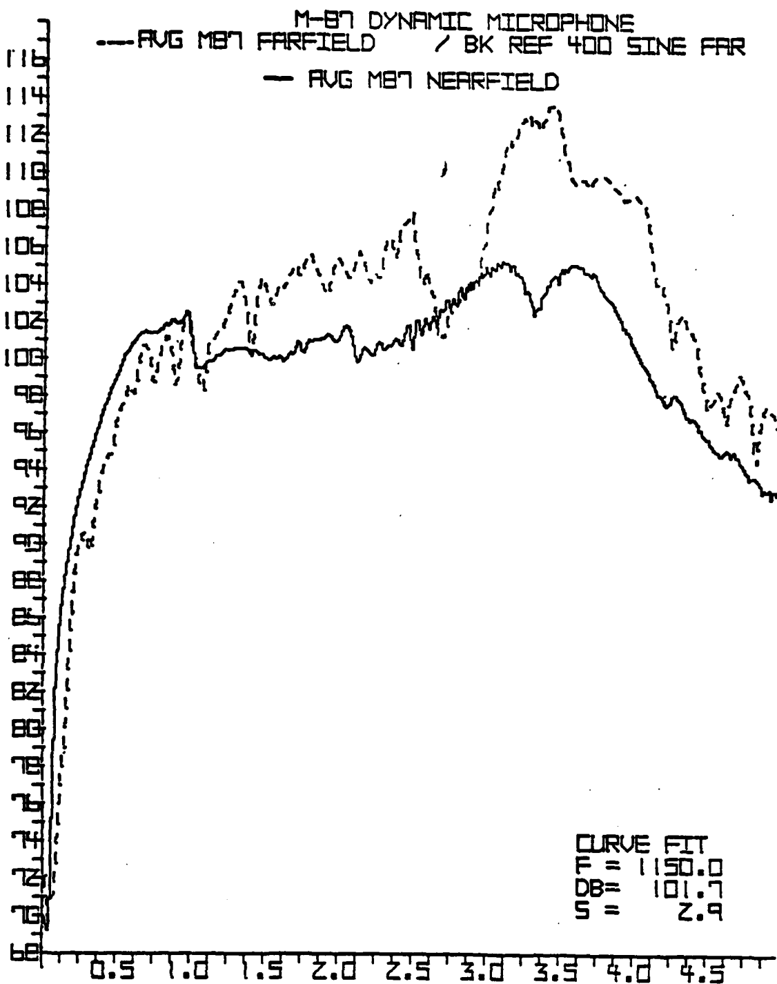
Figure 7. M-87 Dynamic Microphone
