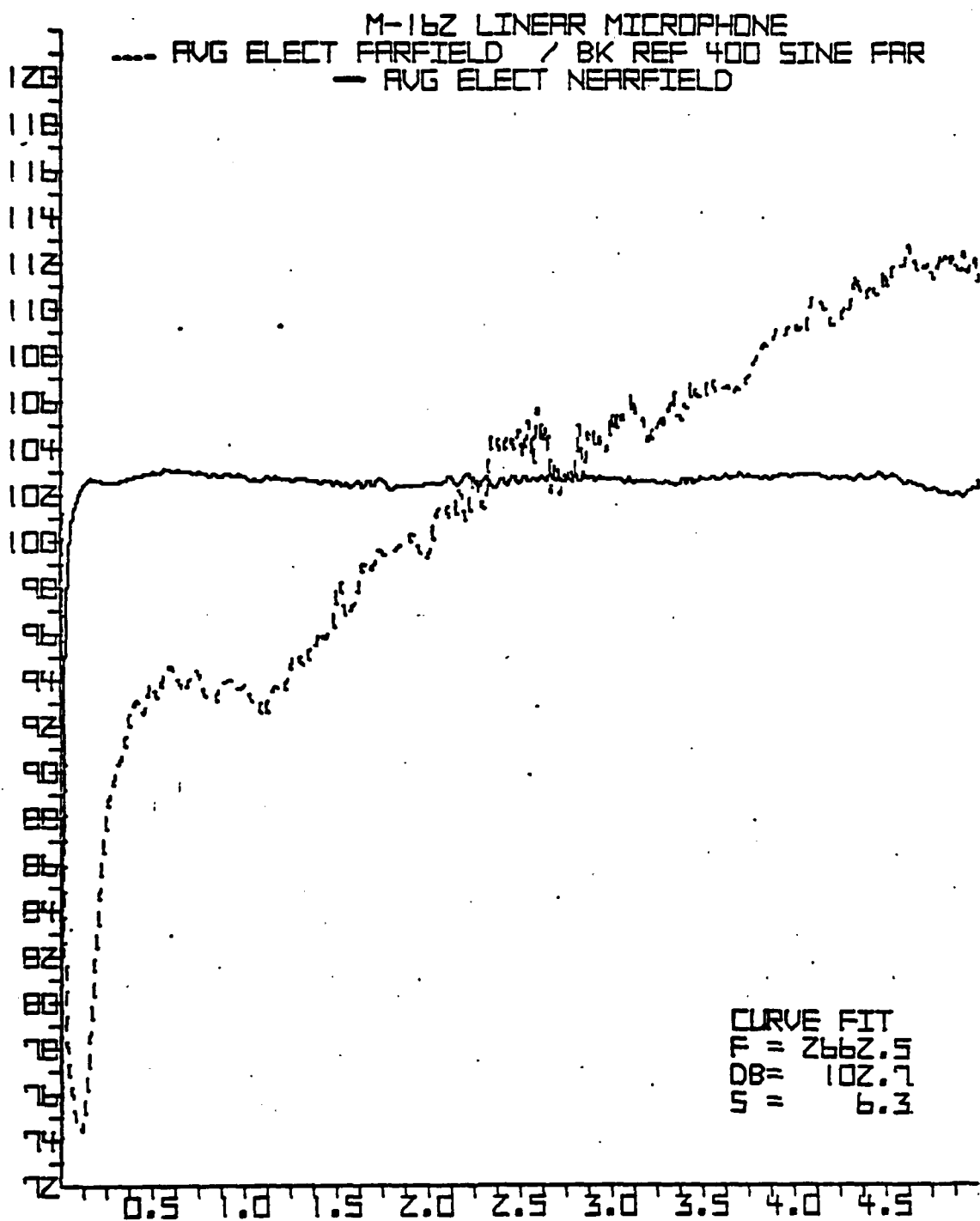
Figure 8. M-162 Linear Microphone
