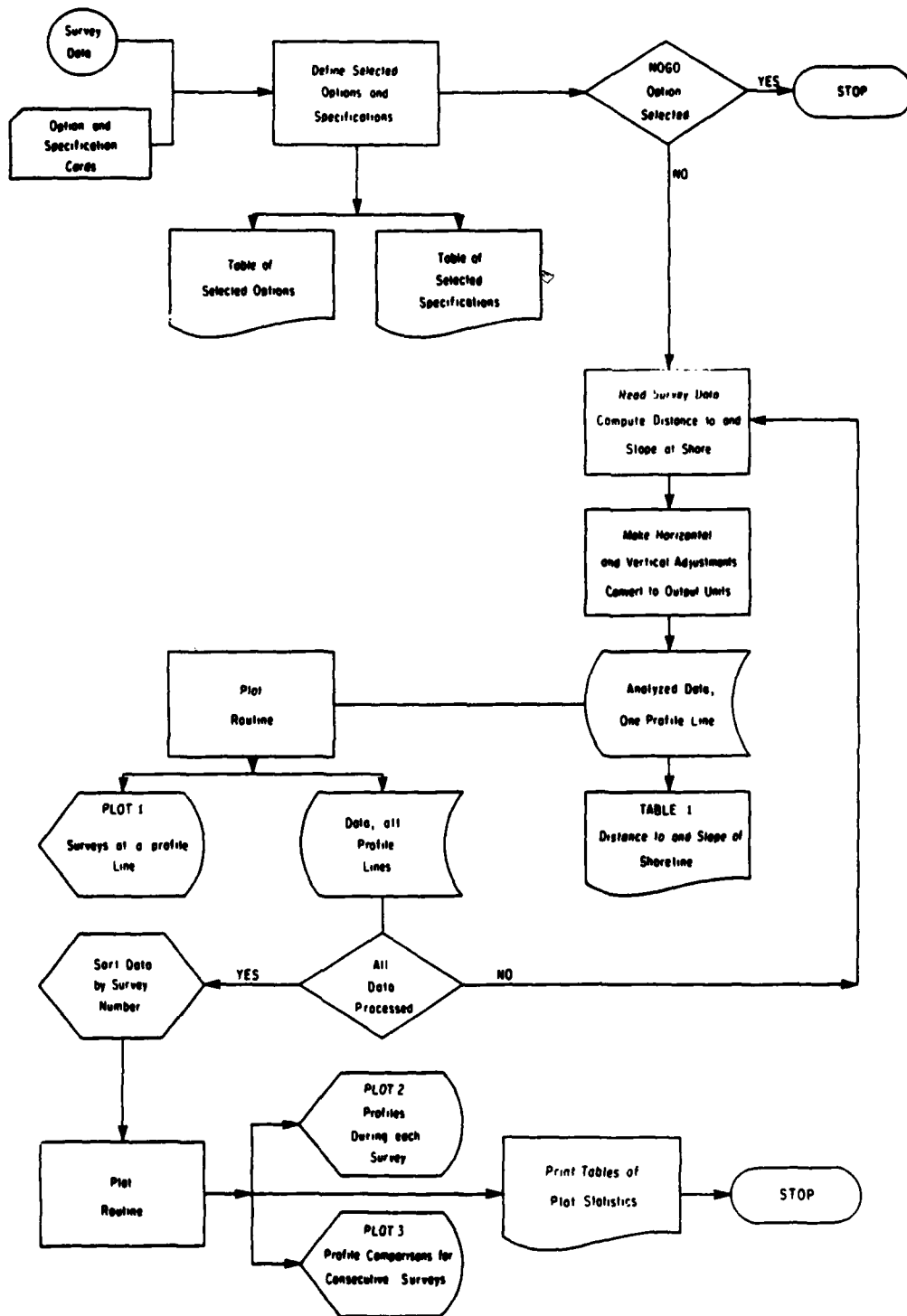
Figure 2. Analysis module SURVY1.
