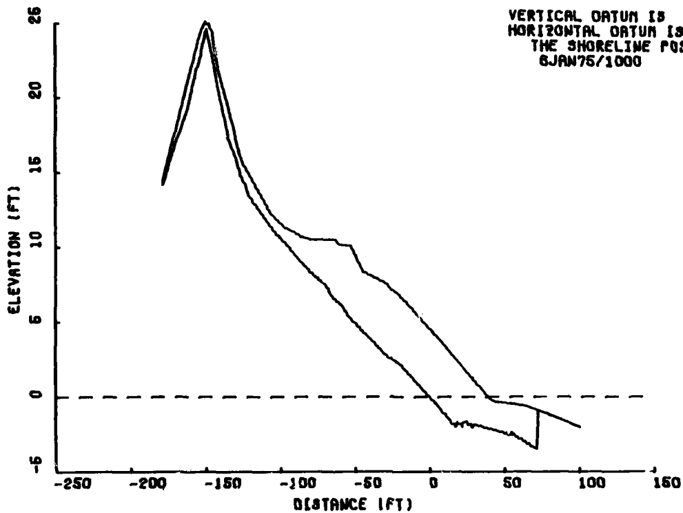
PROFILE ENVELOPE FOR PROFILE LINE 1 AT TEST BEACH 8JAN75/1000 - 15DEC76/0900
