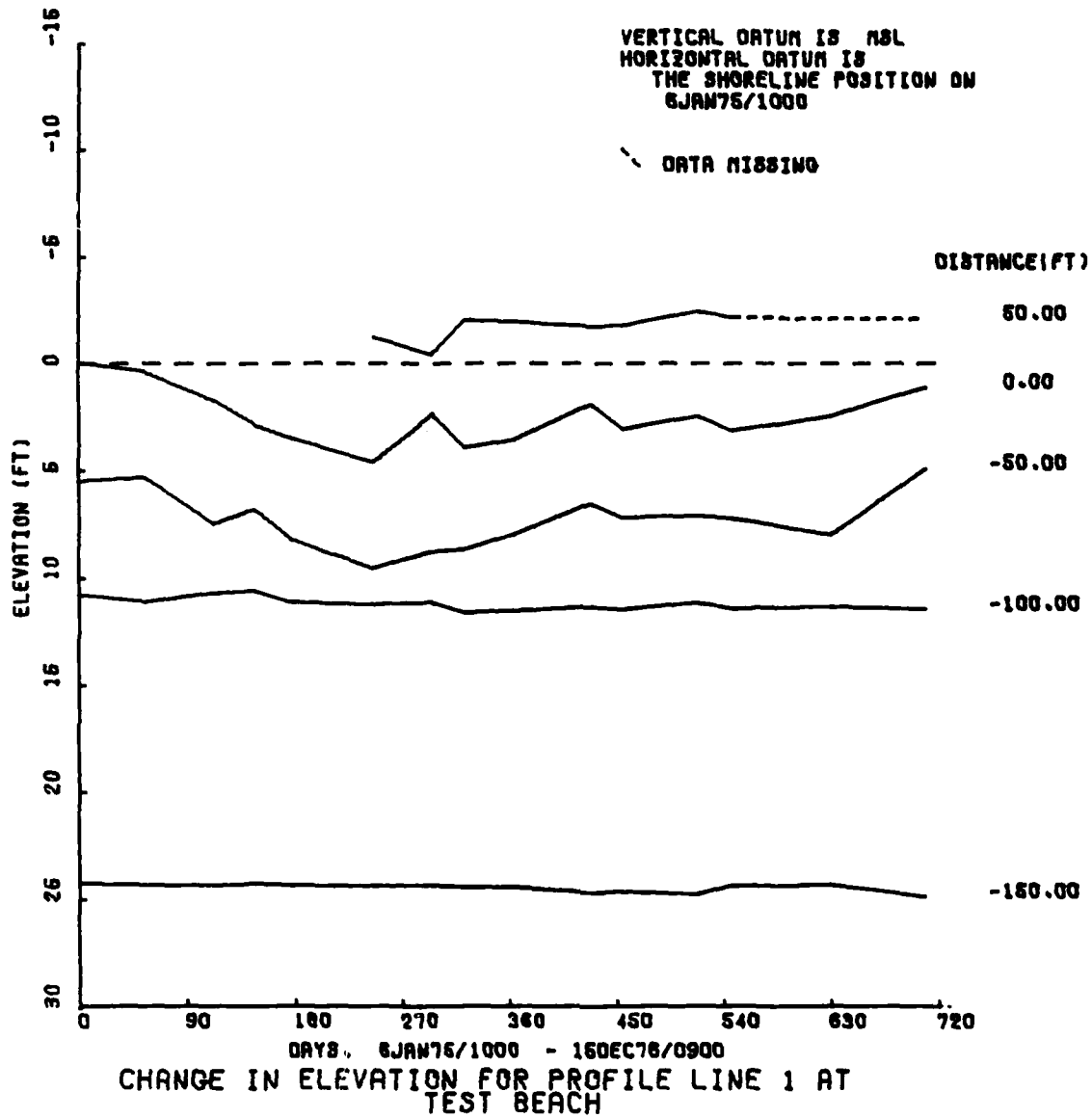
Figure 7. Sample ELVDIS output--change in elevation at specific distances, PLOT19.
