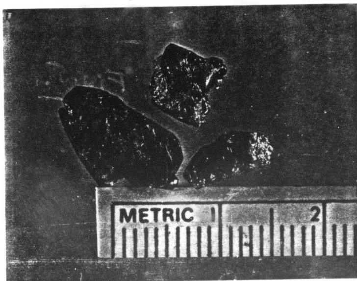
Figure 8. NAB crystals.
