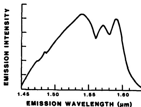
Figure 29. Emission spectra of ErP_5O_{14} , LiErP_4O_{12} , and ErAl_3(BO_3)_4 in eye-safe region.
