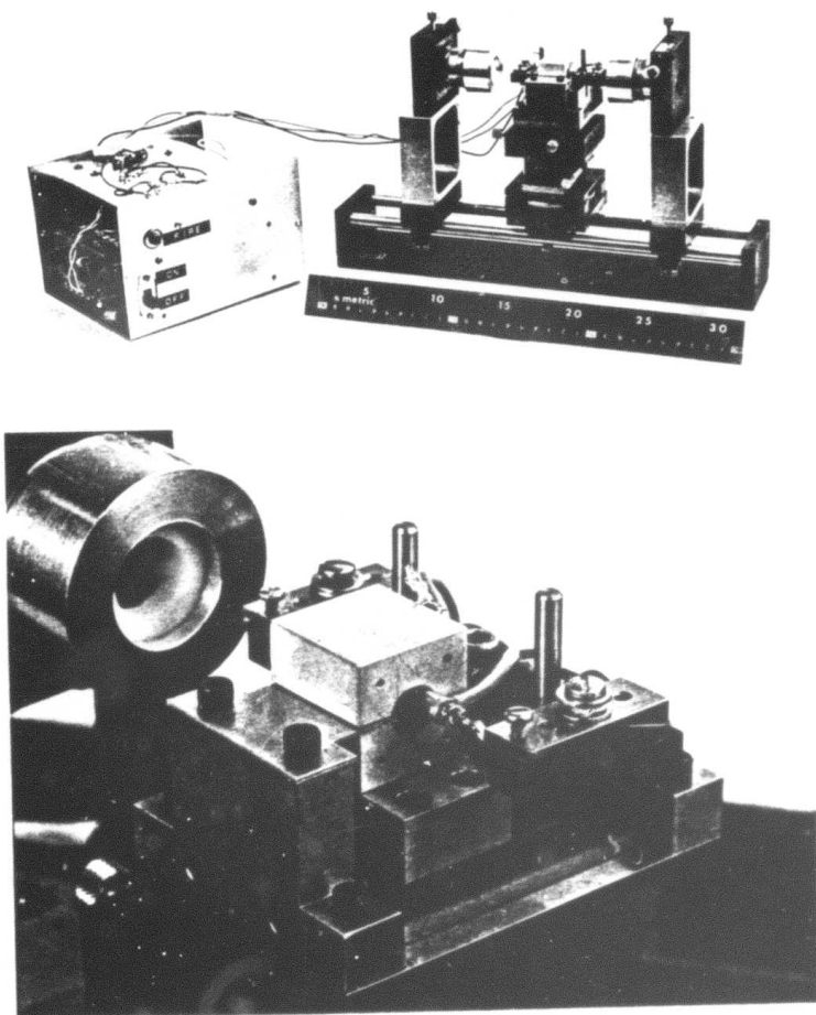
Figure 19. Experimental laser setup (SE) and laser head showing pump cavity, flashlamp, and NPP laser rod.
