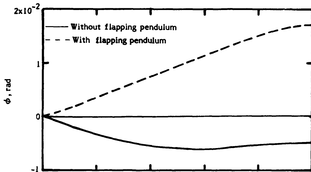
(c) Torsional deflection.
