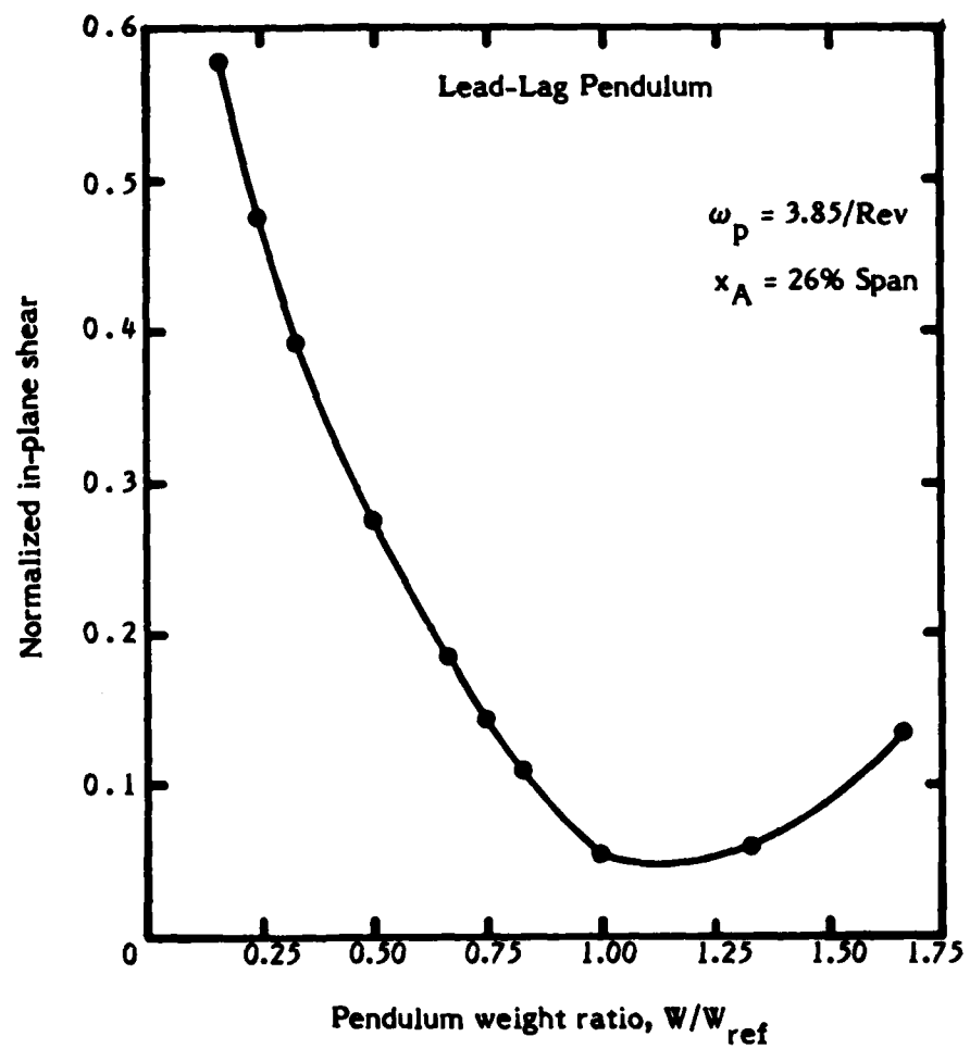
Figure 29. - Root in-plane shear for 4/Rev concentrated excitation, nonuniform blade, W_{\text{ref}} = 133.45 \text{ N} , \eta_A = \zeta_A = 0 .
