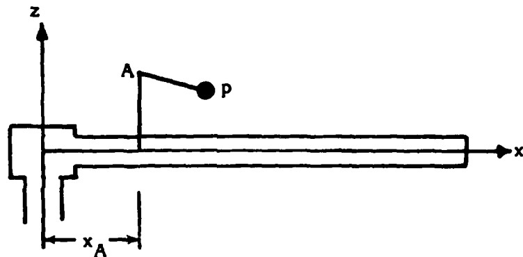
Figure 3. - Blade-mounted flapping pendulum before deformation.
