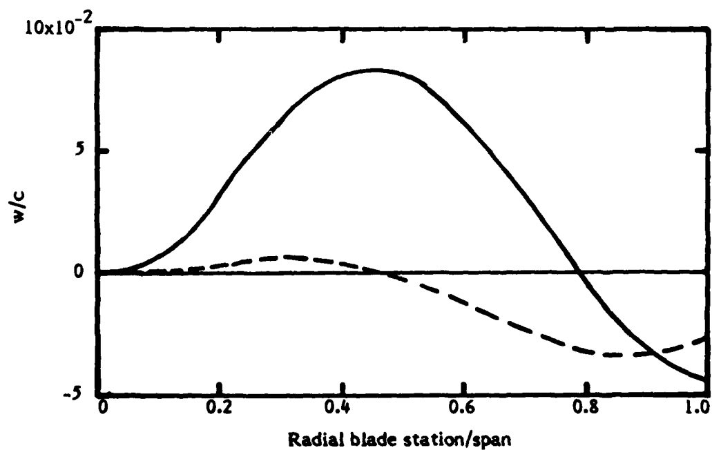
(b) Flapwise deflection.
