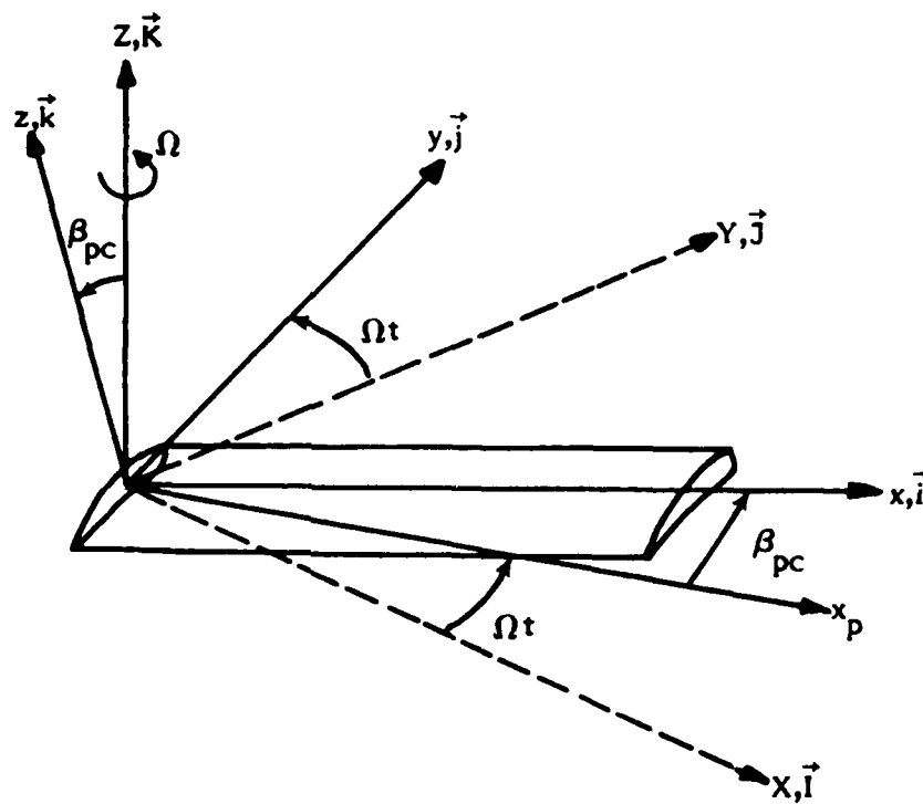
Figure A-1. - Undeformed coordinate system.
