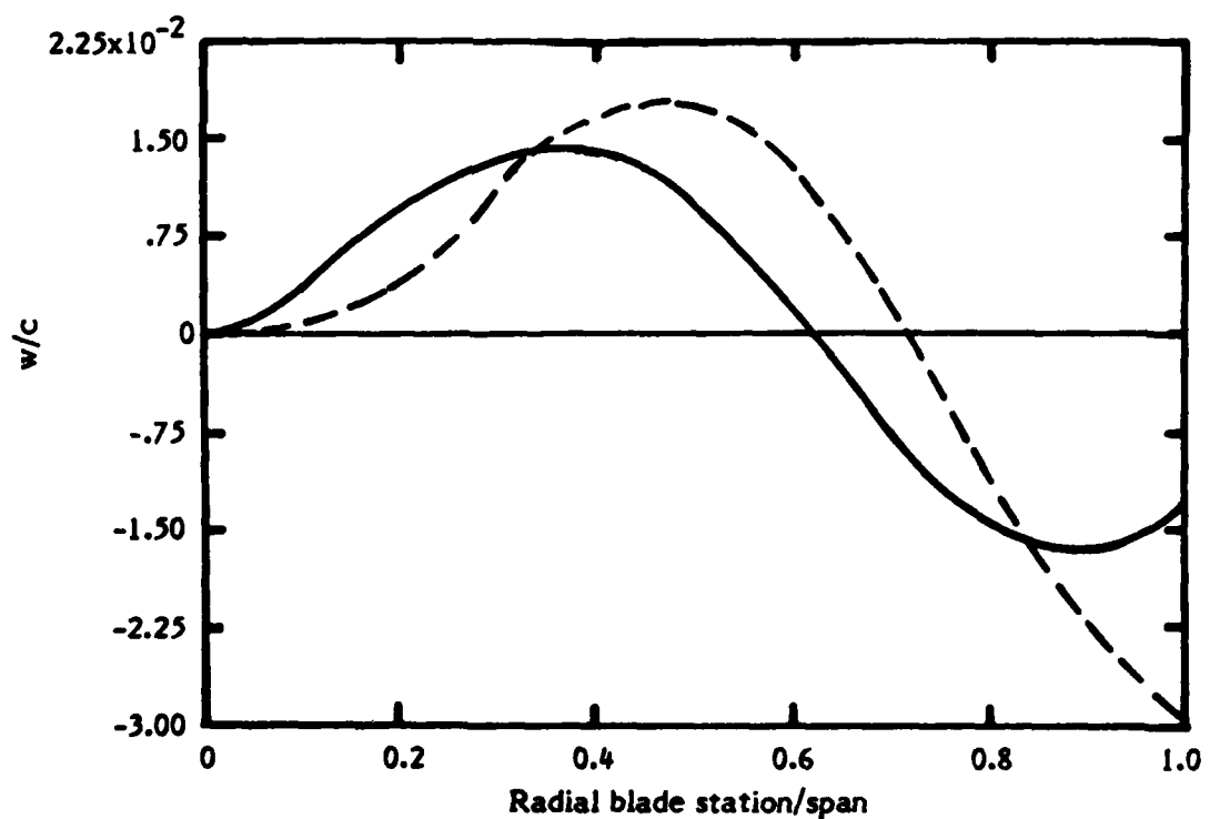
(b) Flapwise deflection.
