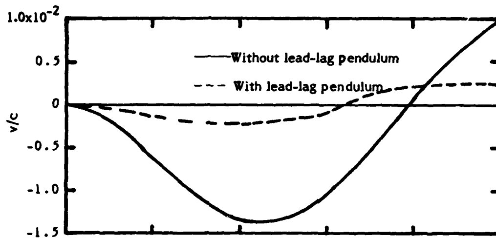
(a) Lead-lag deflection.
