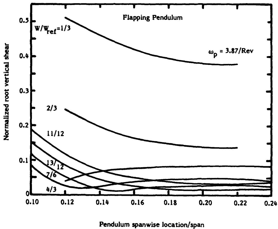
Figure 10 - Root vertical shear for 4/Rev concentrated excitation, uniform blade, W_{ref} = 66.73 \text{ N} , \eta_A = \zeta_A = 0 .
