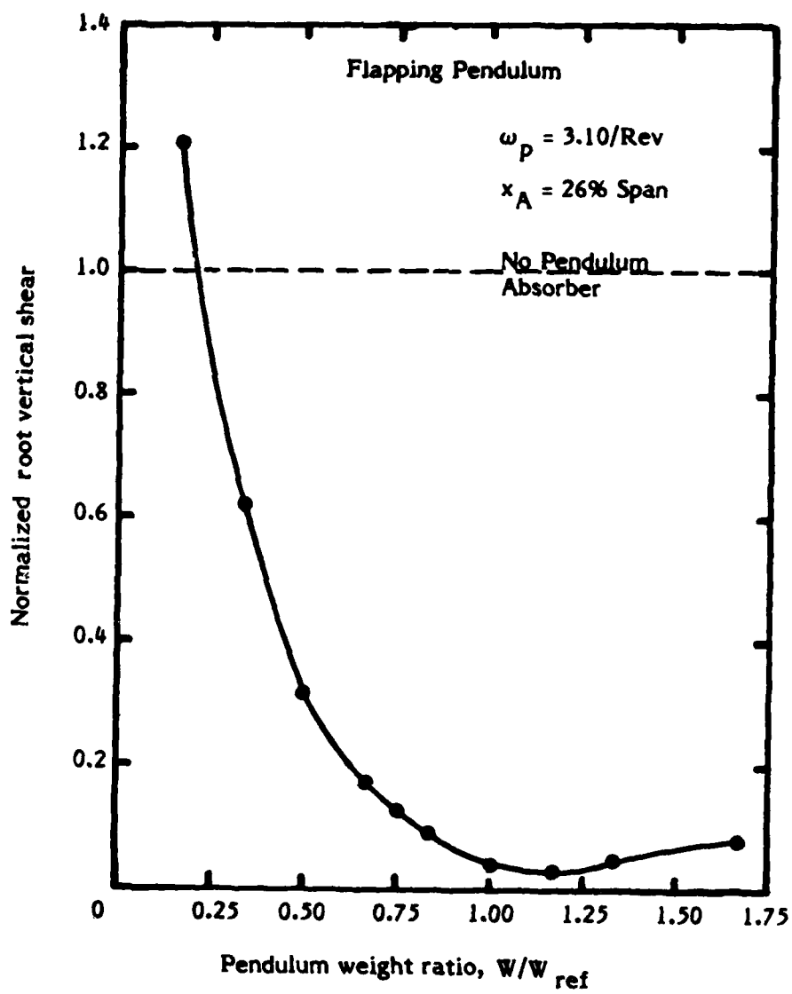
Figure 27. - Root vertical shear for 3/Rev distributed airload excitation, nonuniform blade, W_{ref} = 133.45 \text{ N} , \eta_A = \zeta_A = 0 .
