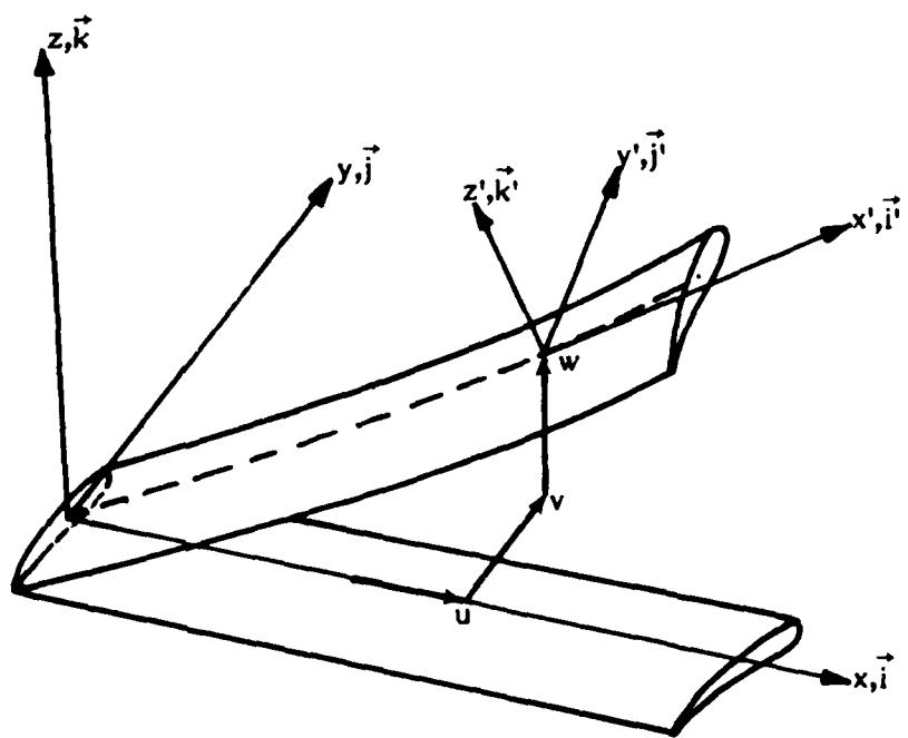
Figure A-2. - Blade elastic displacements.
