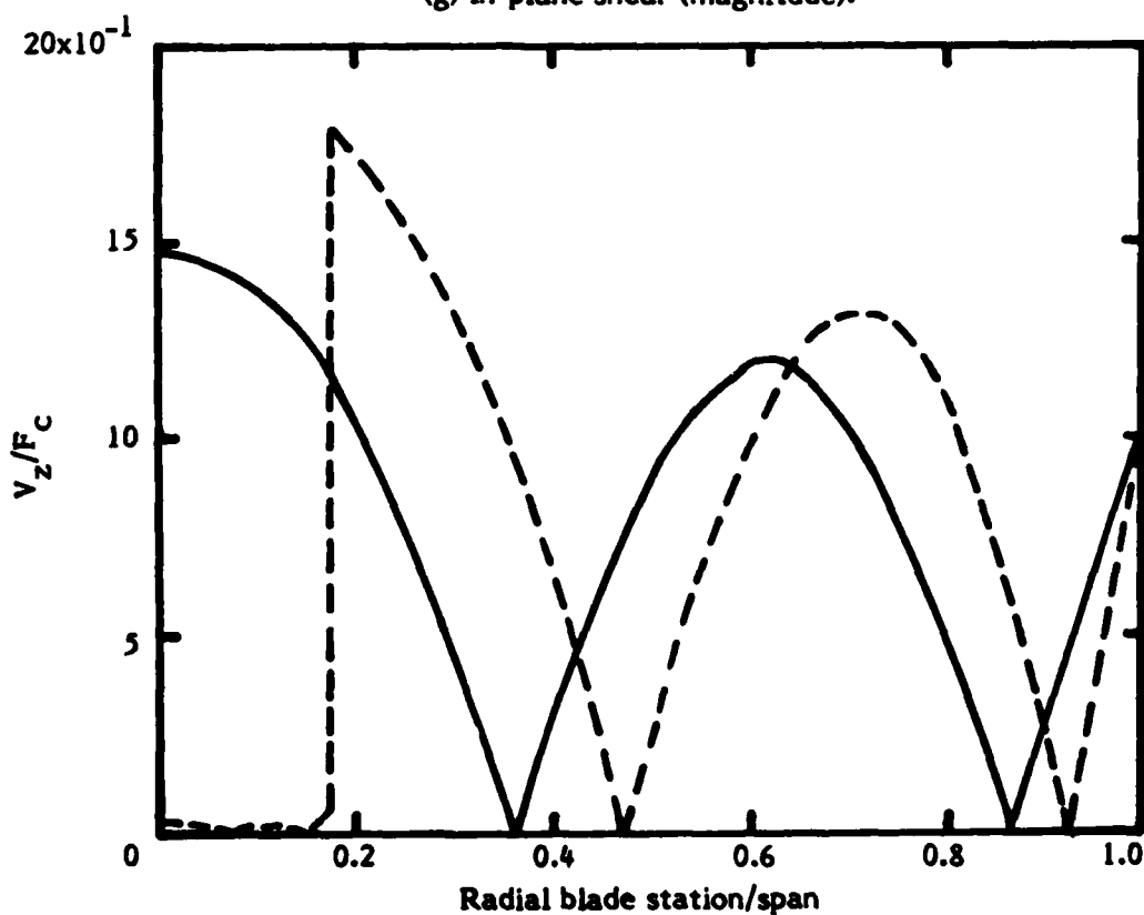
(h) Out-of-plane shear (magnitude).
