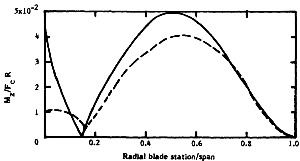
(f) In-plane moment (magnitude).
