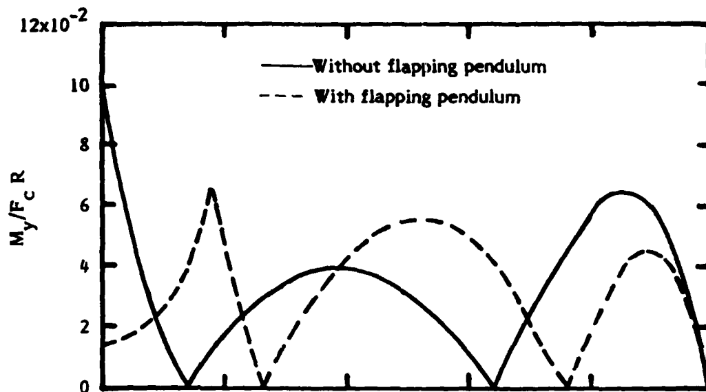
(e) Out-of plane moment (magnitude).
