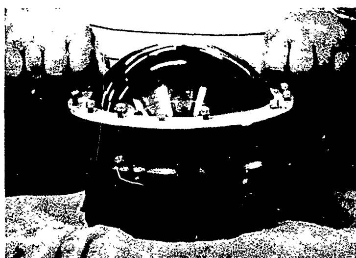
Figure 53. The bolt holes are lined up and screws are inserted through the window retainer into the mounting ring.
