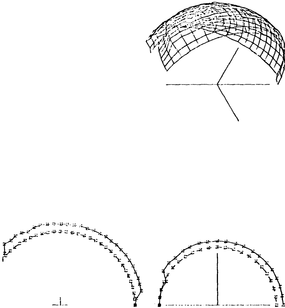
Figure 2 Deformed configuration of the discontinuous hemispherical shell structure due to an internal blast (deflection magnification: 1000)
