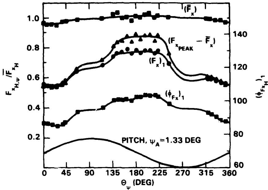
Figure 11a - F_x Component
