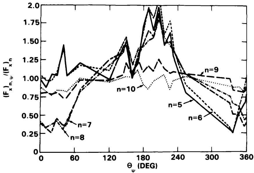
Figure 14b - Harmonics n = 5 to n = 10
