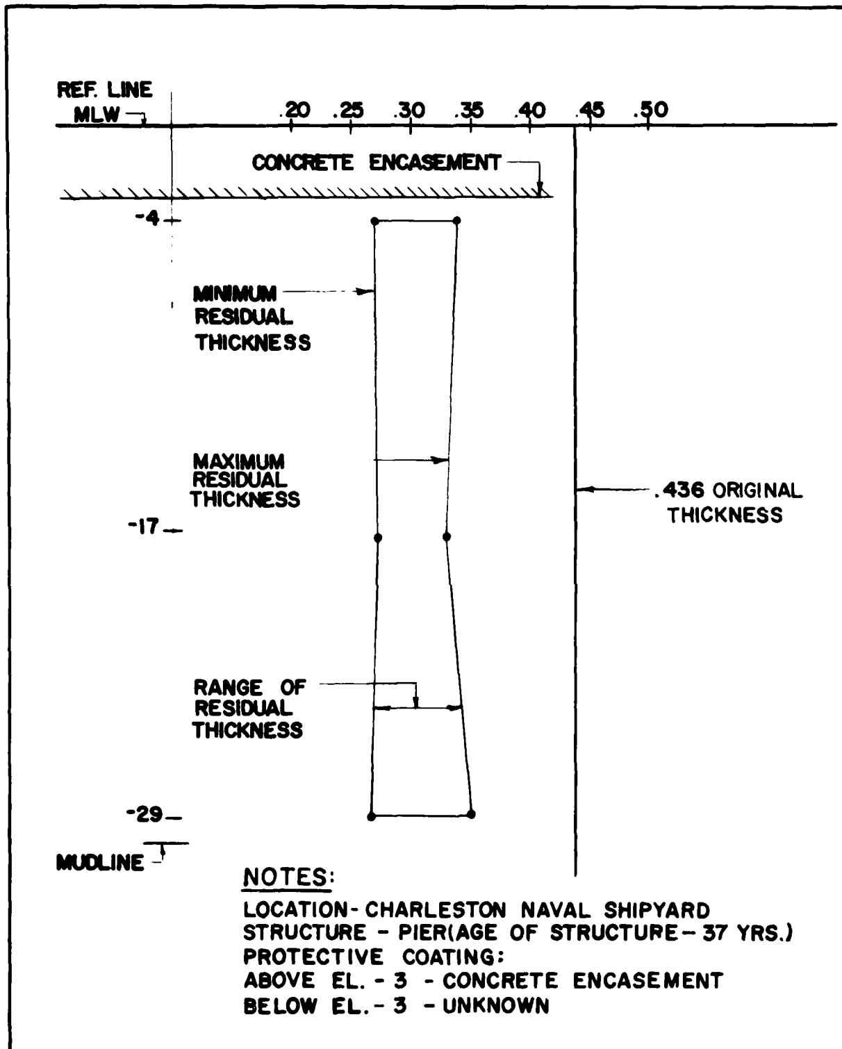
FIGURE 5 Measured Profile Envelope-Steel H-Piling 25.6-24
