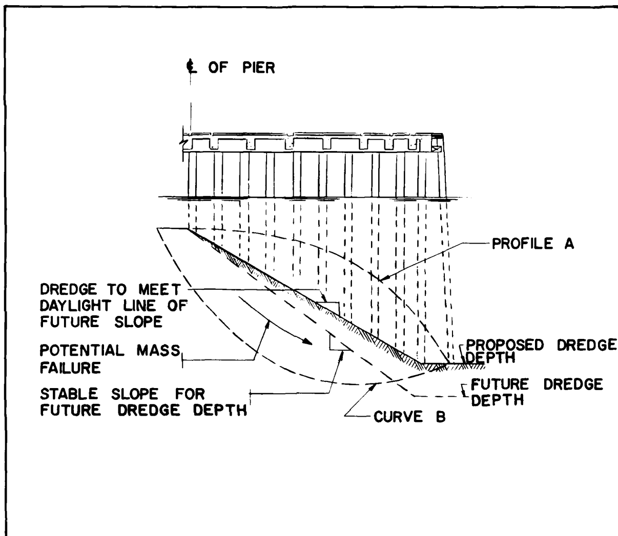
FIGURE 9 Dredging Under a Platform
