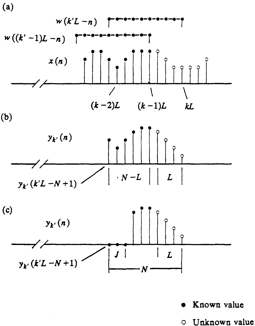
Fig. 3.3 Sequences for Proof of Conditions 3.4
