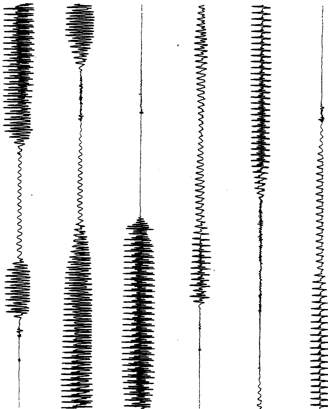
Fig. 4.5 Sequential Least-Squares Reconstruction
