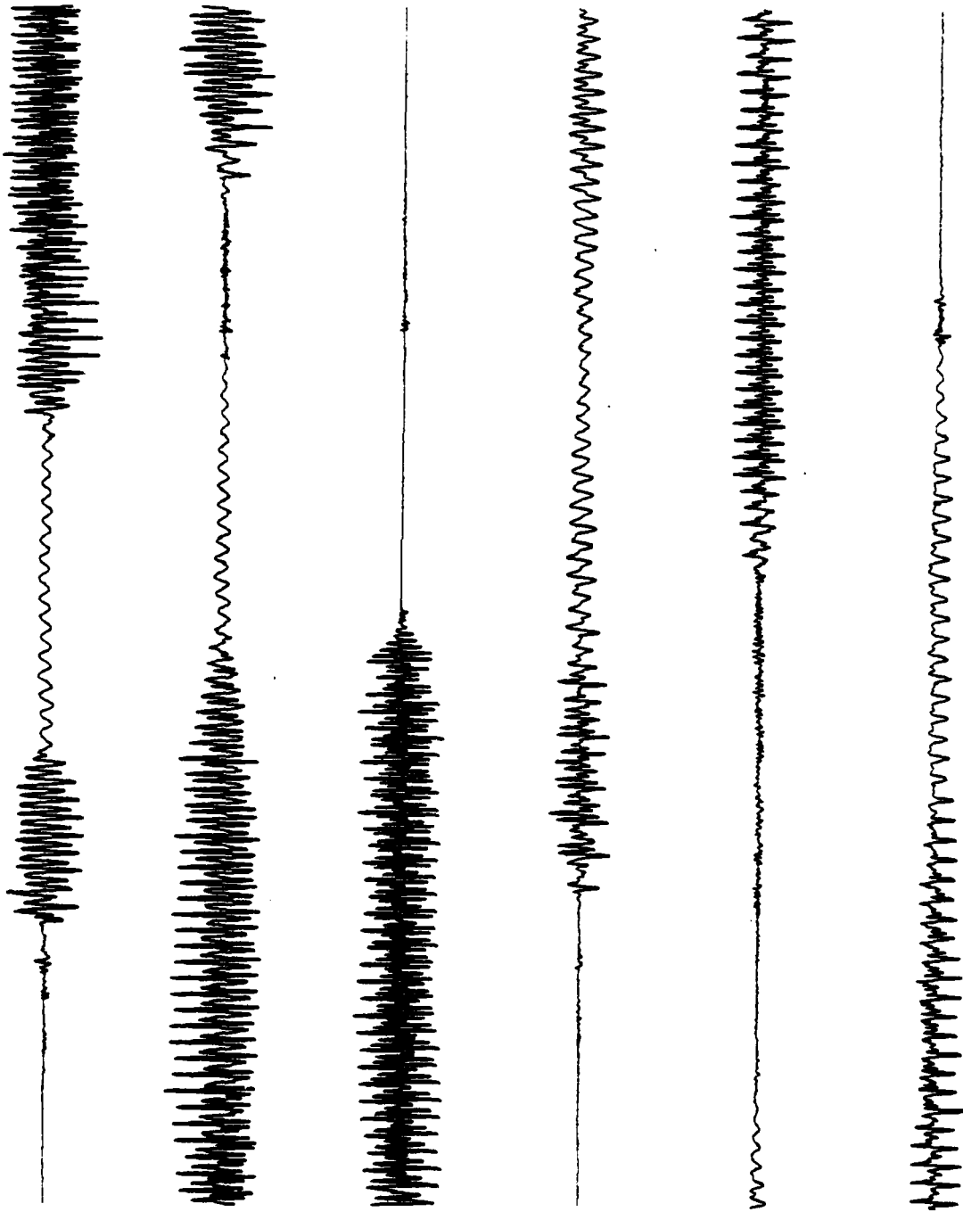
Fig. 4.6 Sequential Iterative Reconstruction
