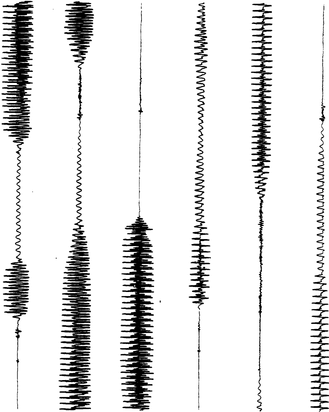
Fig. 4.4 Sequential Reconstruction Based on Theorem 2.1
