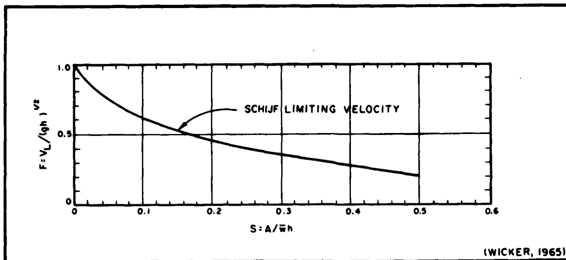
FIGURE 9 Sogreah Laboratory Squat Curve
