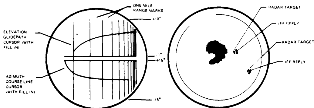
Az-el Beta Scan Display
