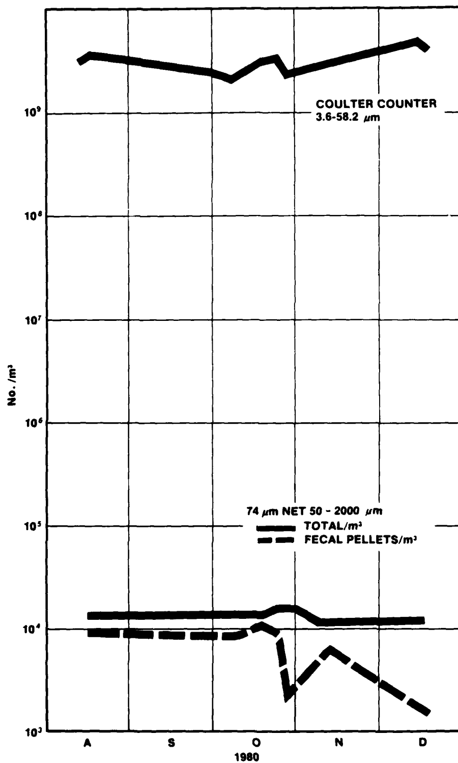
Figure 1. Concentration of Bottle and Net Particles/m 3
