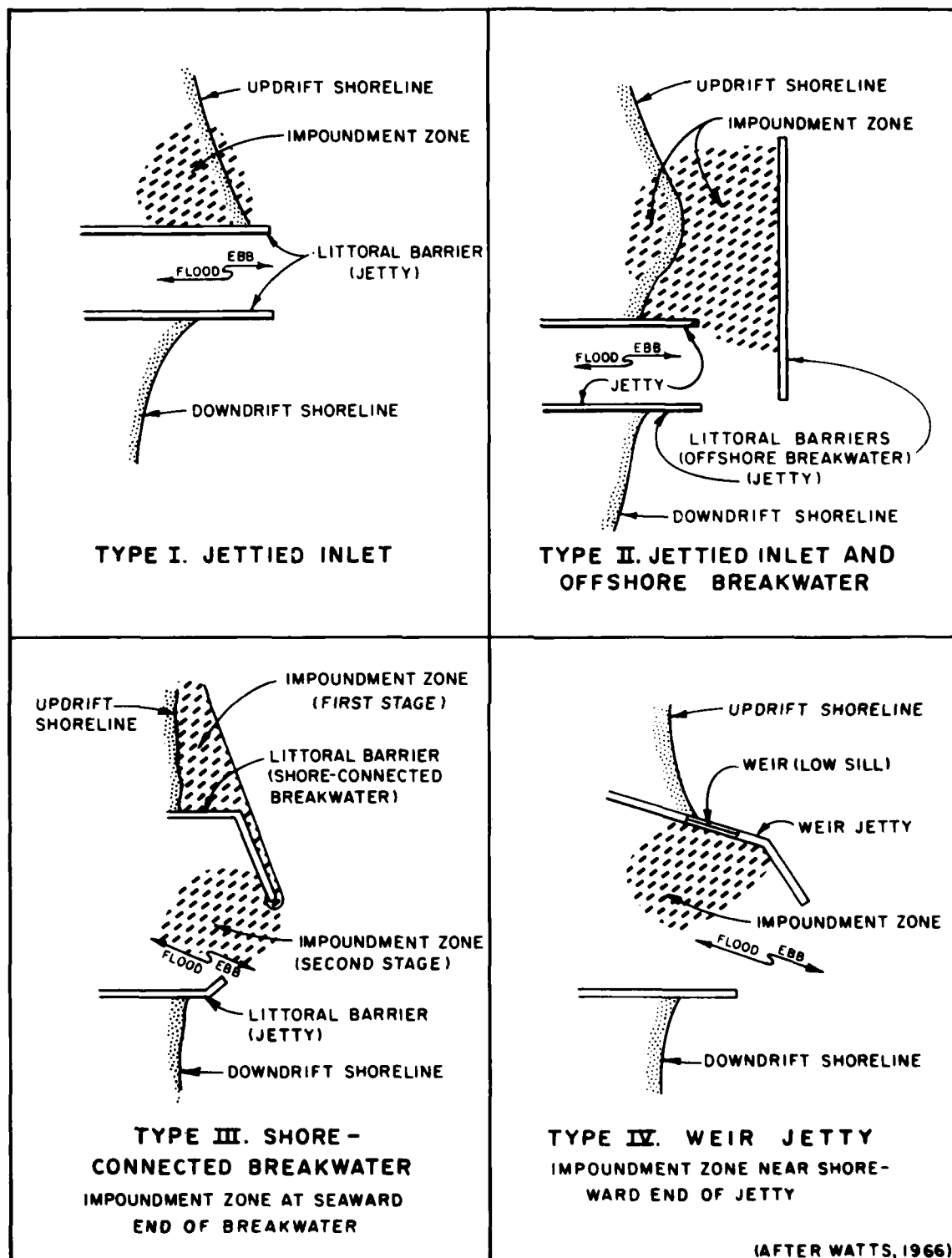
FIGURE 9 Harbor-Entrance Configurations
