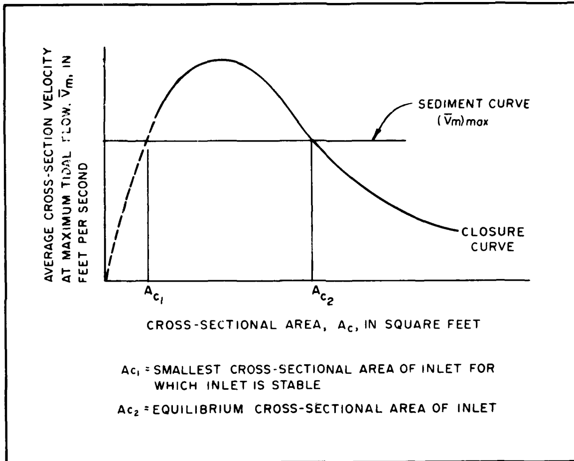
FIGURE 11 Inlet-Closure Curve
