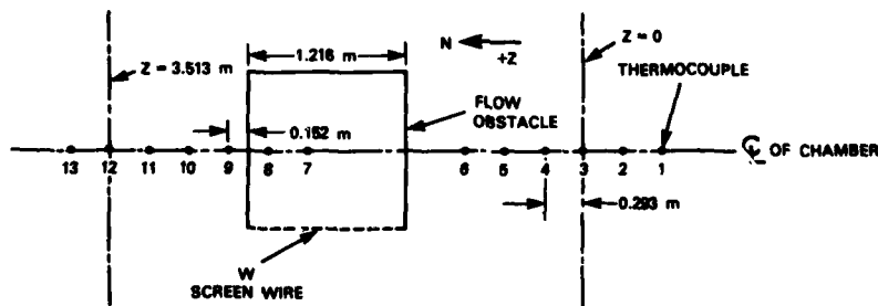
Fig. 2 - Plan-view schematic of FIRE I interior giving obstacle and thermocouple locations along the centerline relative to the vertical plane z = 0
