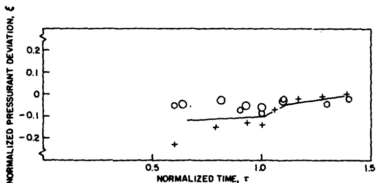
Fig. 5 - Model-prototype comparison with obstacle. Data are for location 10 in Fig. 2 (O) and homologous locations for UW model (+) and NRL 5-m 3 (O).
