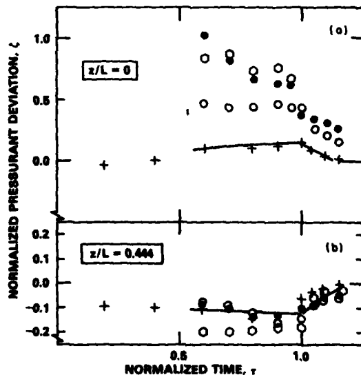
Fig. 6 - Model prototype comparison without flow obstacle. Example comparisons of centerline data for NRL FIRE I (O) and 5-m 3 experiment with 25.4-mm (e) and 15.2-mm (O) nozzles and for UW model experiment with initial pressures of 1 and 6 atm (+).
