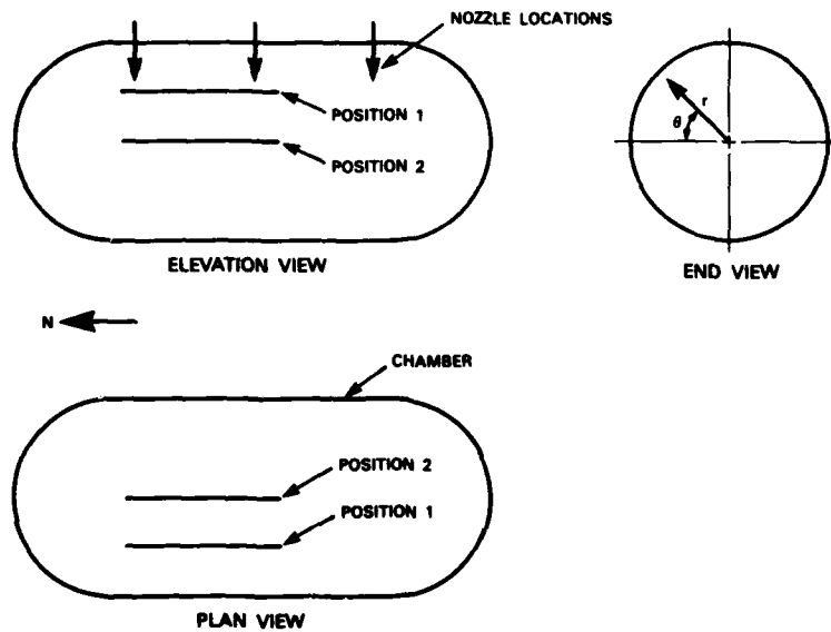
Fig. 1 - Elevation, plan, and end views of FIRE I, showing three nozzle locations and two thermocouple array positions. Chamber diameter is 5.85 m (19.2 ft).
