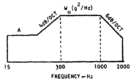
Fig.10 Frequency spectrum for random vibration test
