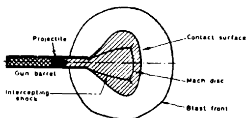
Fig.34 Precursor blast field
