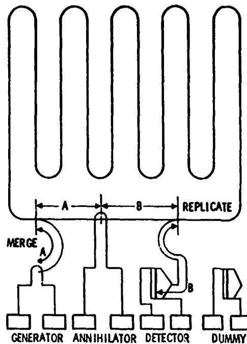
Figure 1.4.3.1 BUBBLE DOMAIN MEMORY SYSTEM
