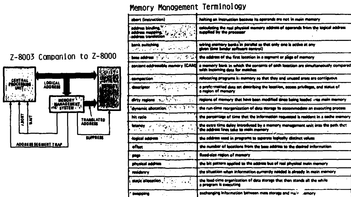
FIGURE 1.5.3.1 NEW CHIPS PROVIDE VIRTUAL MEMORY MANAGEMENT
