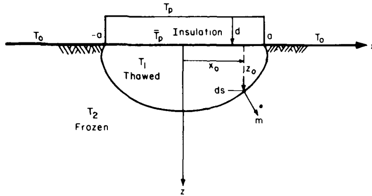
Figure 1. Insulated semi-infinite strip.
