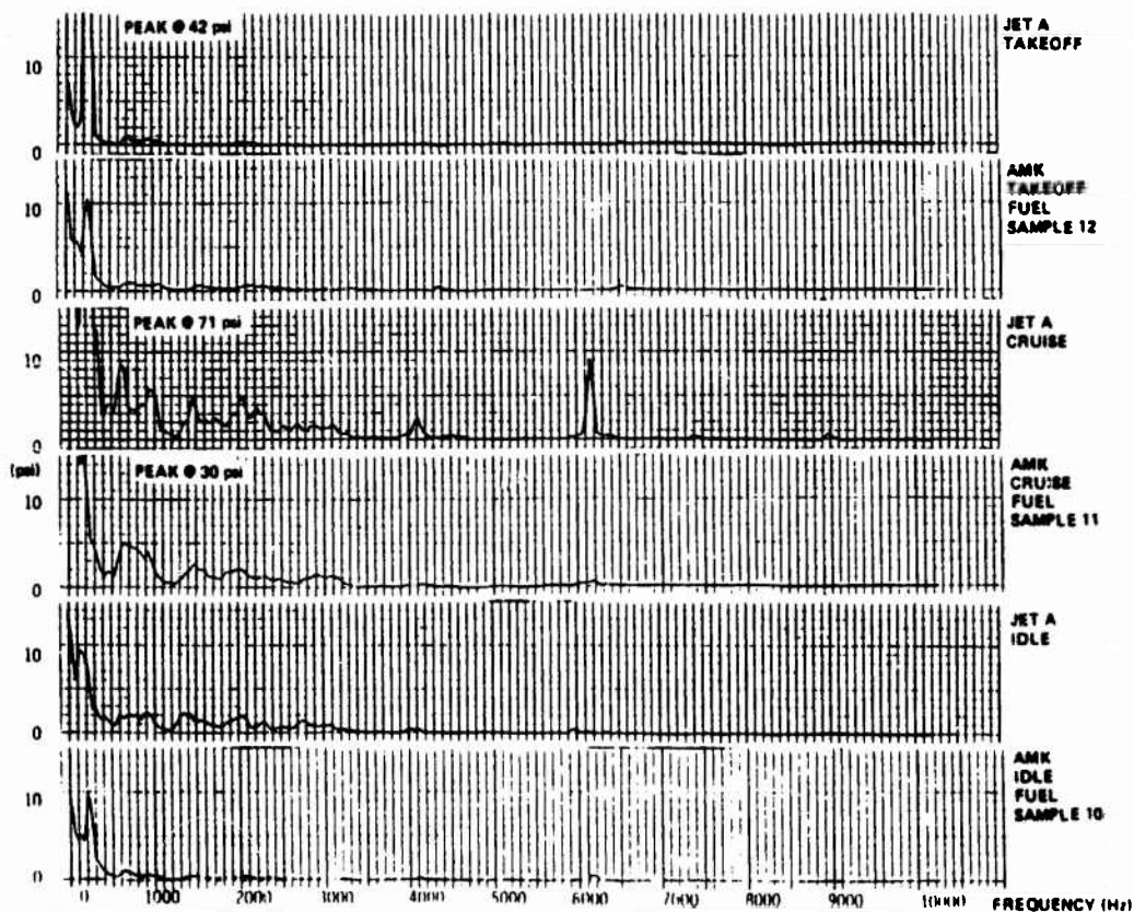
FIGURE 26B. PUMP DISCHARGE PRESSURE PULSATION, DIFFUSER #2
