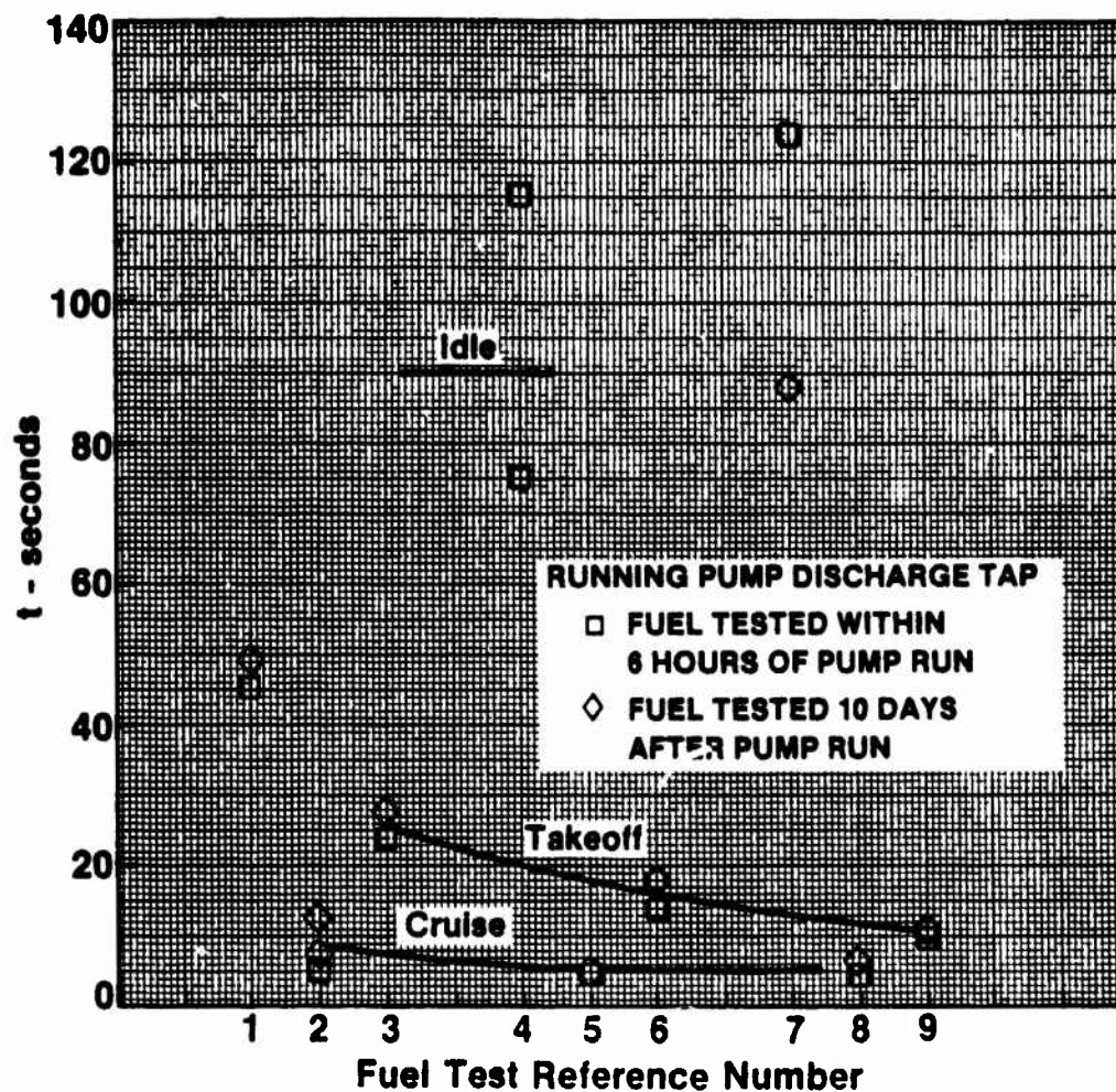
FIGURE 16. FILTER FLOW TIMES FOR DEGRADED AMK - 1st TEST SERIES
