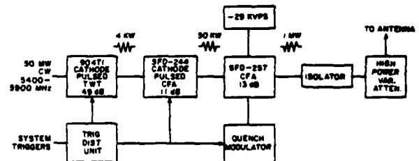
Figure 1. AN/MPS-36 Transmitter Amplifier Chain
