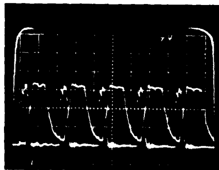
Figure 6. Display of Quench Voltage Pulser and RF Output Envelopes in Burst Mode Operation
