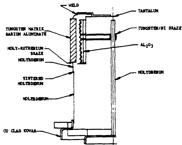
FIGURE 1 A2960 CATHODE
