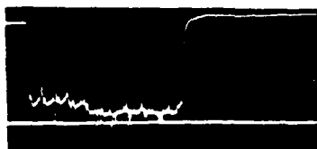
Fig. 22 External beam current with bumpers excited with waveform of Fig. 21
