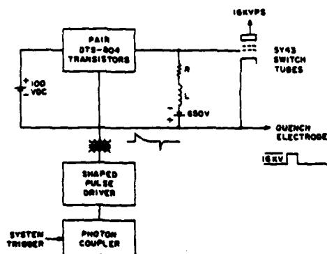
Figure 5. Transistorized Bootstrap Grid Pulser for Switch Tubes
