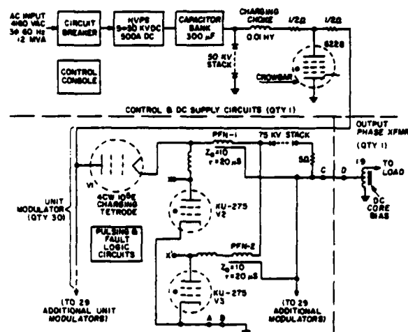
Figure 3. 2.5 Gigawatt Modulator
