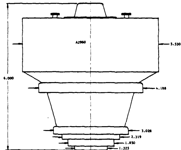
FIGURE 7 A2960 OUTLINE
