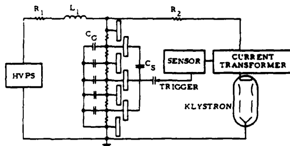
Figure 2 - Simplified Schematic With Improved Multigap Crowbar
