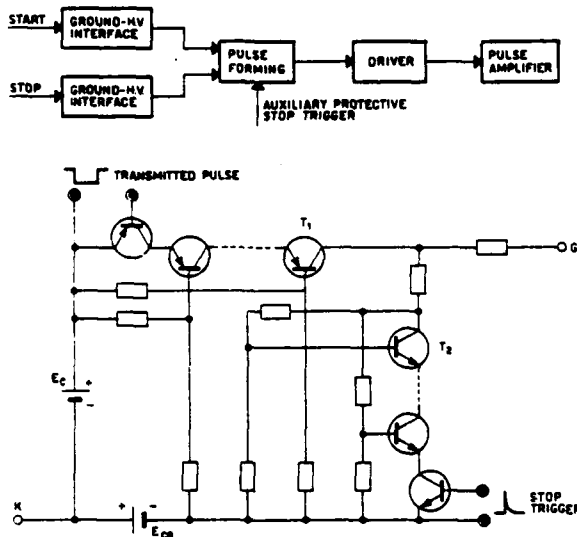
Figure 2. Grid modulator schematic
