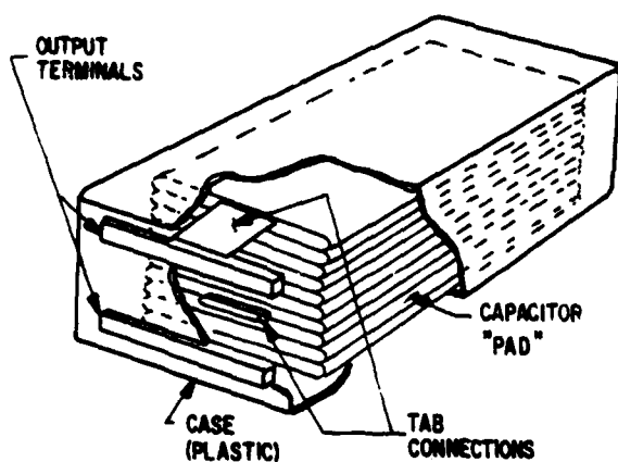
Figure 8. Construction of Generalized Plastic Cased Capacitor
