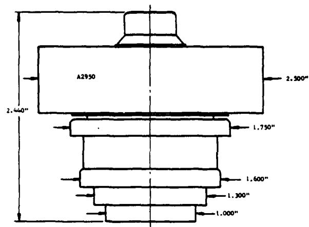
FIGURE 3 A2950 OUTLINE
