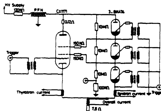
FIG. 4: THYRAGNITRON ELECTRICAL CIRCUIT
