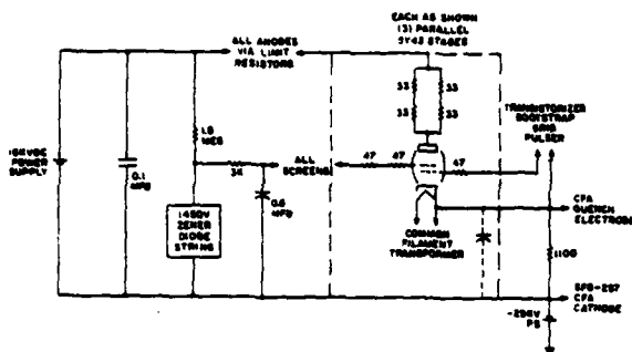
Figure 4. Quench Pulser for SFD-257 Crossed Field Amplifier
