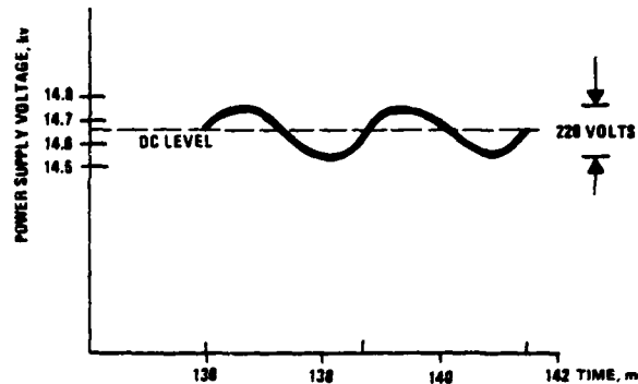
FIGURE 5A. ECAP PREDICTED VOLTAGE VARIATION OF POWER SUPPLY AT CONSTANT PRF OF 360 PPS
