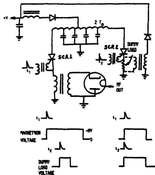
CASE A: t_1 AND t_2 TIME DISPLACED CASE B: t_1 AND t_2 TRIGGER SIMULTANEOUSLY
