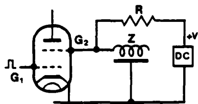
Fig. 10a. For Tetrodes e.g. CX1157 CX1529/GHT9 CX1528/GHT8
