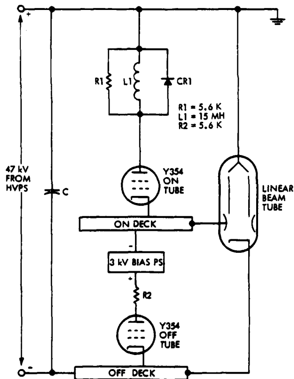
FIG. 4. MODULATOR WITH PASSIVE ASSIST NETWORKS
