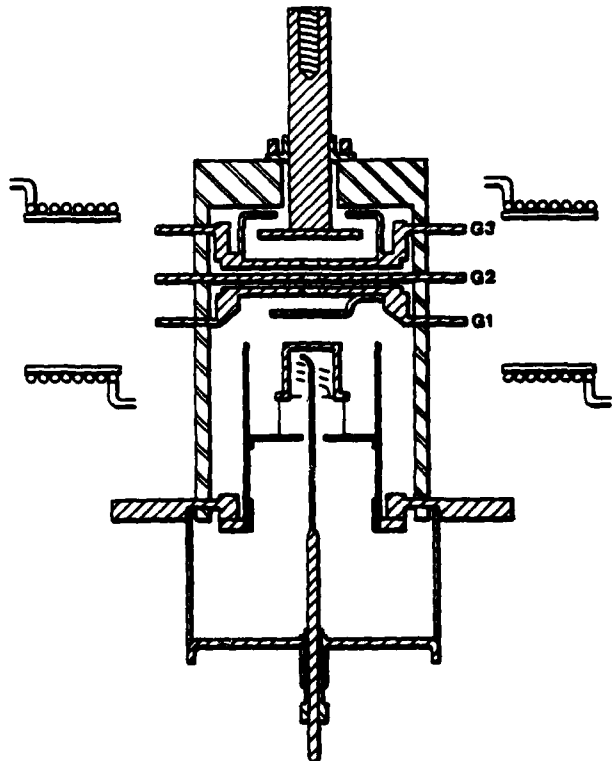
Fig.1 Diagram of Triple Grid Thyatron with Magnetic Field Coils
