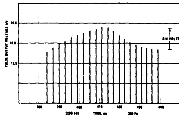
FIGURE 6B. ECAP PREDICTION OF PULSE AMPLITUDE OUTPUT UNDER PRF VARIATION
