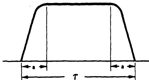
Figure 3 Pulse waveform to be used as goal for synthesis-parabolic rise and fall with flat top.
