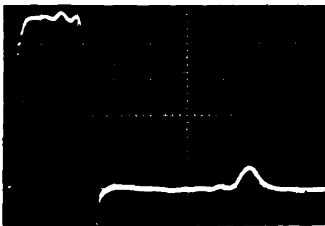
(b) RSR Stack Current Under Shorted Load Operation (2000 A/Div Vert, 10 \mu Sec/Div Horiz)
