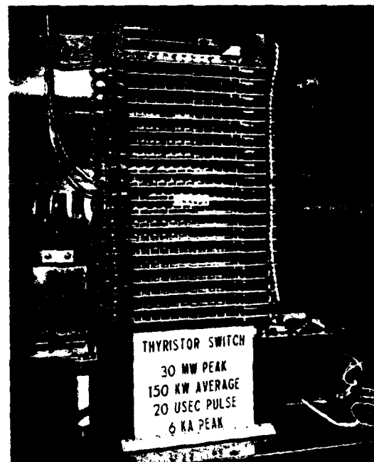
Figure 3. Thirty Megawatt Switch
