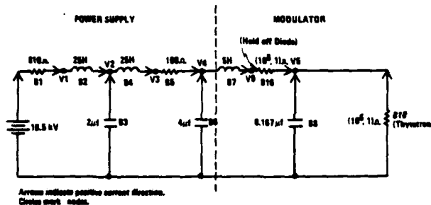
FIGURE 4. ECAP POWER SUPPLY AND MODULATOR MODEL
