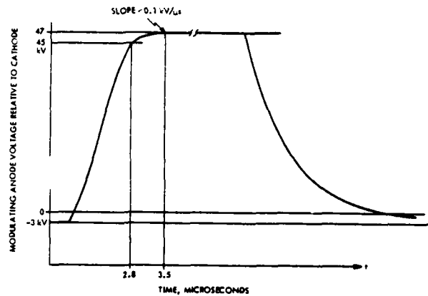
FIG. 5. MODULATOR WAVEFORM WITH PASSIVE ASSIST
