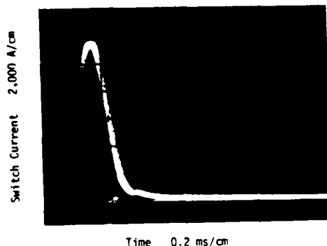
Figure 9: Single pulse of current through the switch (includes load current and first half cycle of the arc quench current). Load resistance, 0.2Ω; firing voltage, 2000V.
