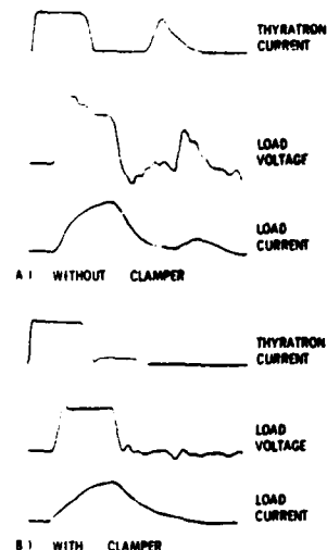
LOAD VOLTAGE AND CURRENT WAVEFORMS
