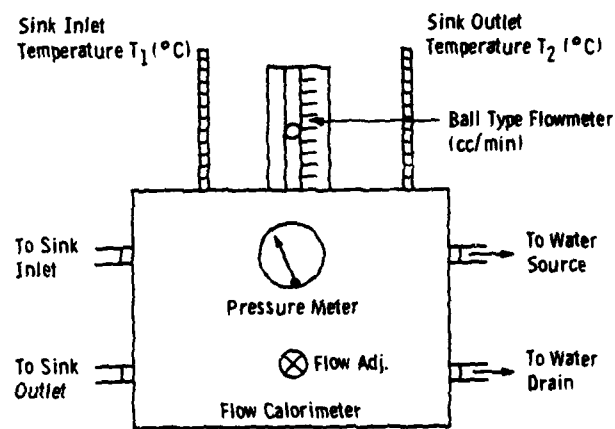
Fig. 3 - Flow Calorimeter Power Measuring System
