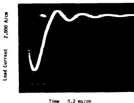
Figure 10: Single pulse of current to 0.2Ω load delivered by switch. Firing voltage, 2000V. Oscillations after main pulse are decay of arc quench circuit.
