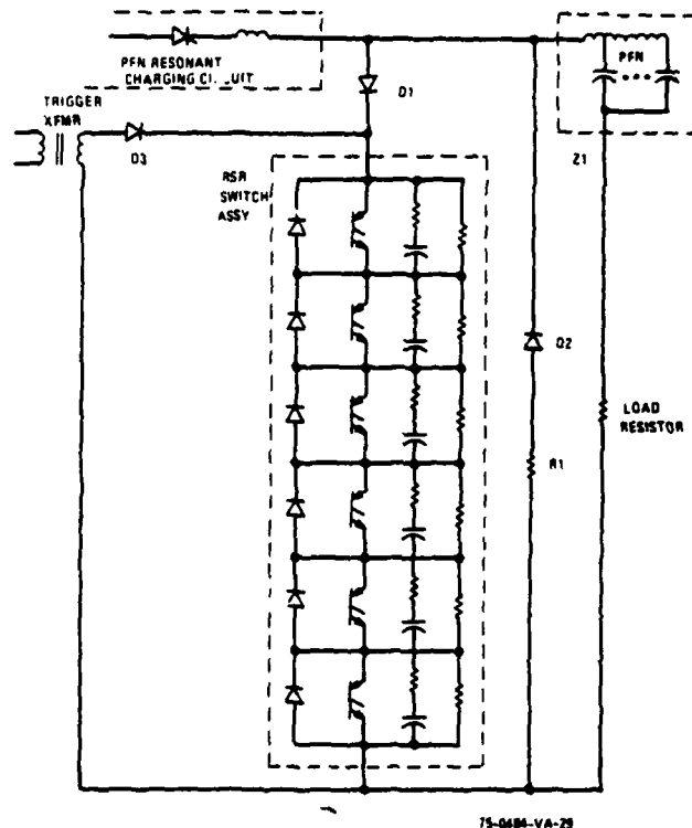
Figure 3. Module Breadboard Circuit
