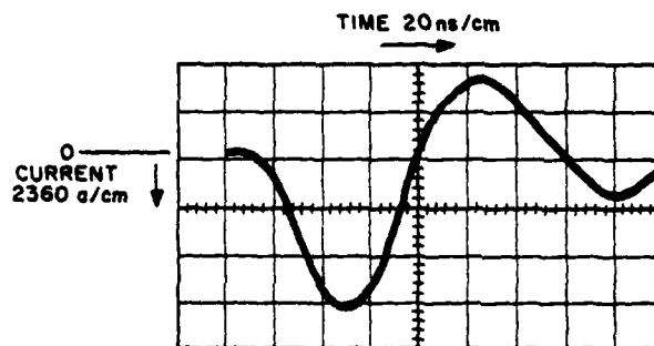
HY-1102 IN FIG. 5 APPARATUS 0.01μf, 0.45 OHM LOAD, 19kV
