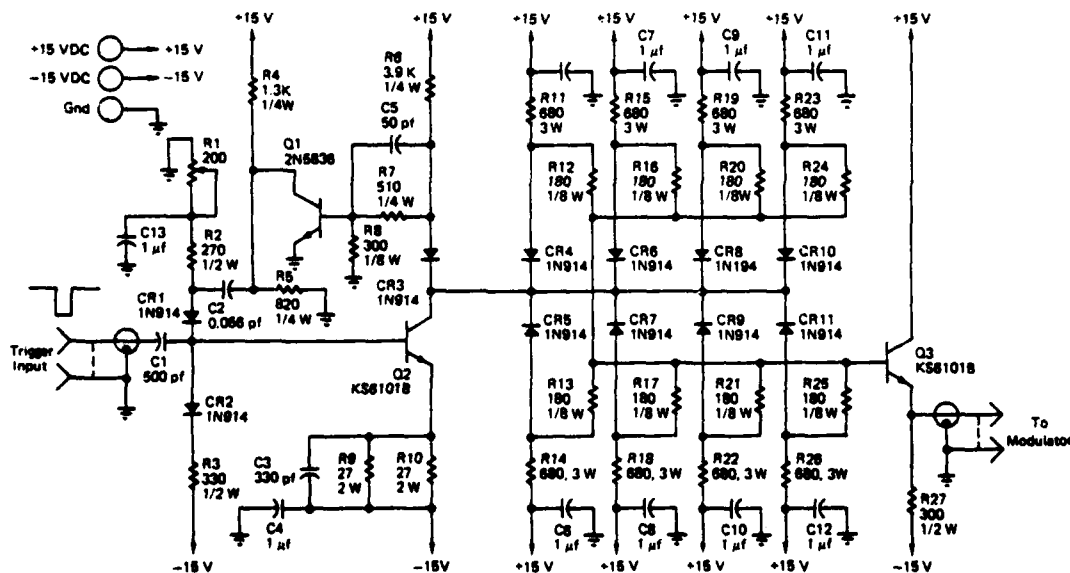
Figure 2 The Modulator Driver Schematic
