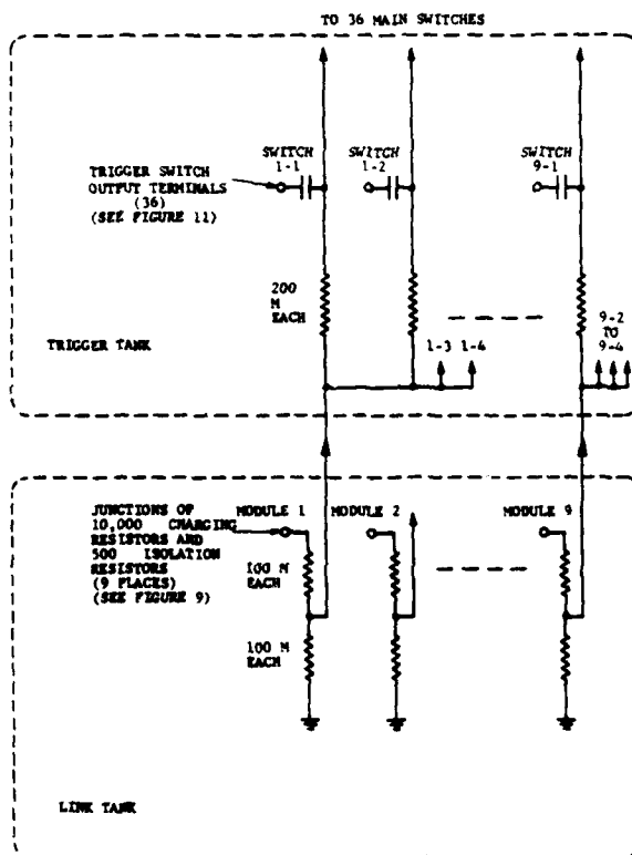
Figure 13. Trigger Bias Distribution
