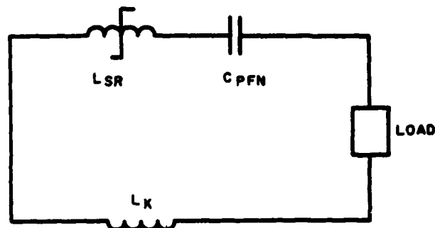
FIGURE IV PFN Equivalent Circuit At PFN Discharge
