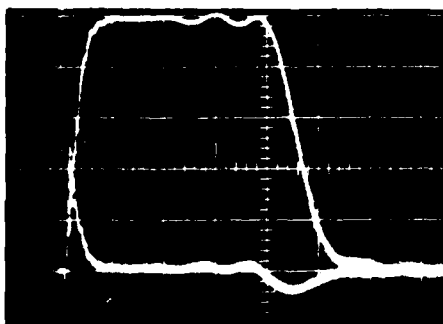
(a) Full Load Pulse Current (1000 A/Div Vert, 5 \mu Sec/Div Horiz)
