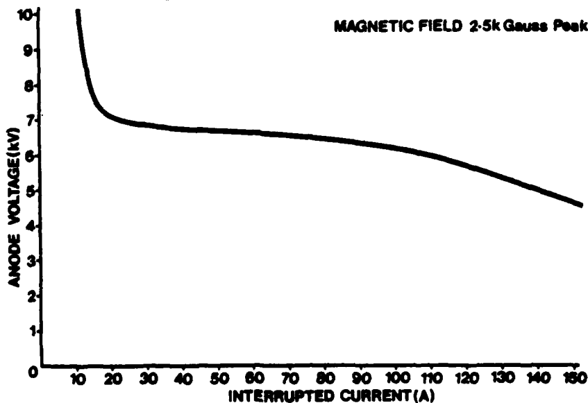
Fig. 5 Limit of Reliable Interruption
