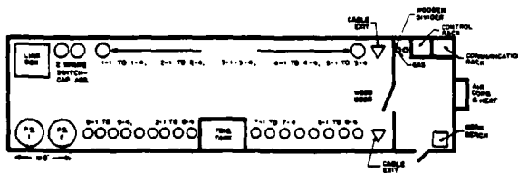
Figure 17. Van Layout
