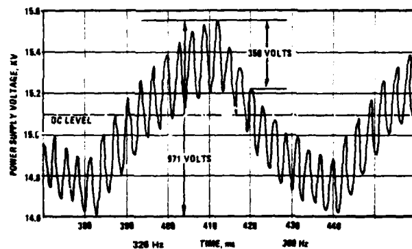
FIGURE 6A. ECAP PREDICTION OF POWER SUPPLY OUTPUT VOLTAGE UNDER PRF VARIATION
