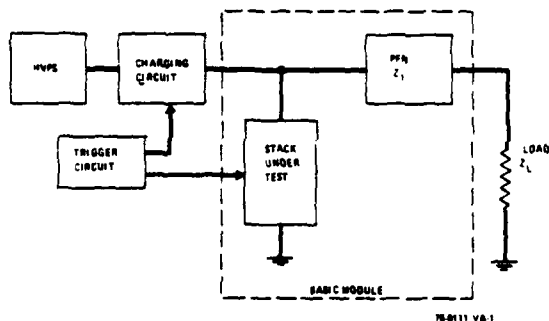
Figure 1. Block Diagram
