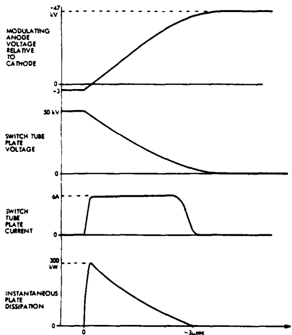
FIG. 3. RISE TIME WAVEFORMS
