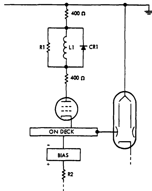
FIG. 6. PORTION OF MODULATOR, SHOWING MODIFICATIONS TO PROTECT CR1 DURING ARCING.
