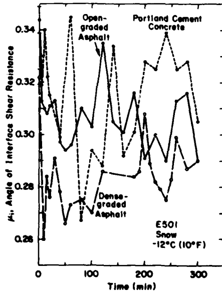
Figure 25. Comparison of variation in coefficient of friction for three pavement types following application of salt on snow at rate of 300 lb/LM, air temperature 10°F, surface friction gauge data.
