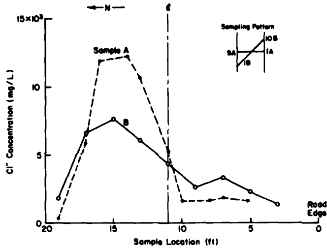
Figure C2. Chloride distribution, test 1, test site 1, 23 January, 1978. Initial snow depth 1 in.
