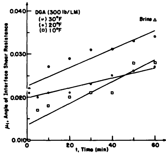
Figure 28. Coefficient of friction change with time, trafficking tests on dense-graded asphalt, 300 lb/LM, for three temperatures.
