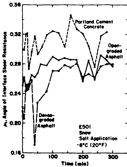
Figure 24. Comparison of variation in coefficient of friction for three pavement types following application of salt on snow at rate of 300 lb/LM, air temperature 20°F, surface friction gauge data.
