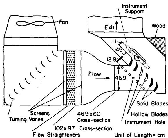
Fig. 2 Schematic of wind tunnel and cascade
