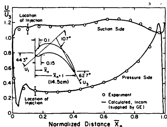
Fig. 3 Normalized mainstream velocity profile on blade, Ma_3 = 0.065 , Re_3 = 2.32 \times 10^5 , \alpha = 35 deg
