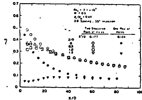
Figure 10 Local Distribution of Effectiveness for M=0.5
