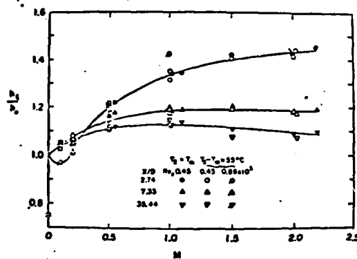
Figure 14 Variation of the Center-Line Heat Transfer Coefficient With Blowing Rate
