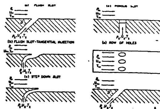
Figure 2 Film Cooling Geometries
