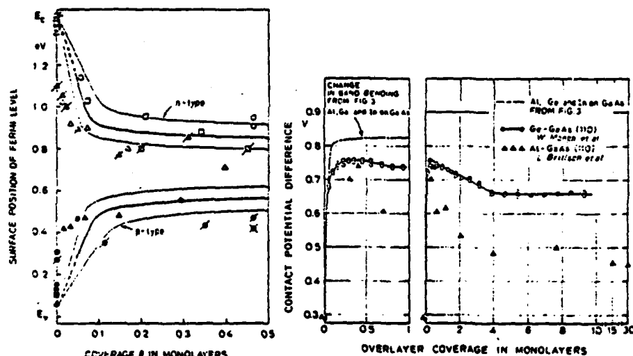
Fig. 3. The Fermi level position E_s in the energy gap of GaAs as a function of metal coverage on both n-type and p-type samples (GaAs(110), 300 K; E_{s1}^n = E_{cs} - (0.55 \pm 0.05) \text{ eV} ; E_{s1}^p = E_{cs} - (0.88 \pm 0.05) \text{ eV} ; N_{As} = (0.06 \pm 0.04) \times 10^{18} \text{ cm}^{-3} ); the data points are from the work of Skeath et al. 7 for three different metals ( \square , aluminum; \circ , gallium; \triangle , indium) obtained by the photoemission technique described in the text and in refs. 5, 8 and 9; —, results determined by Mönch and Gant 12 for germanium on GaAs by contact potential difference measurement techniques; \square , experimental uncertainty of Mönch and Gant.
