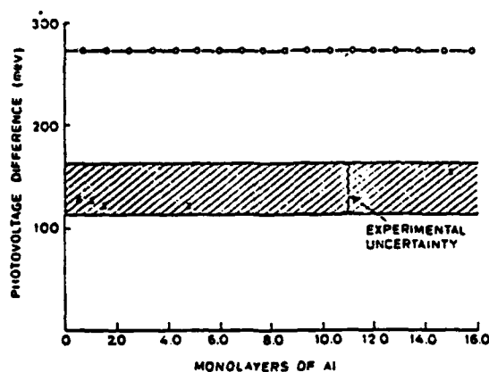
Fig. 7. The difference in photovoltage found by Brillson and Kruger 37 in going from the lowest to the highest intensity light (see Fig. 6 and Table I): —, theoretical upper limit (270 mV) for the photovoltage at 5 \times 10^{18} photons \text{cm}^{-2} \text{s}^{-1} for a real Schottky barrier height of 0.7 eV (see eqn. (2) and text); x, experimental points of Brillson and Kruger 37 . Within experimental error, the photovoltage is independent of layer thickness, in agreement with the conclusion drawn from Fig. 4.
