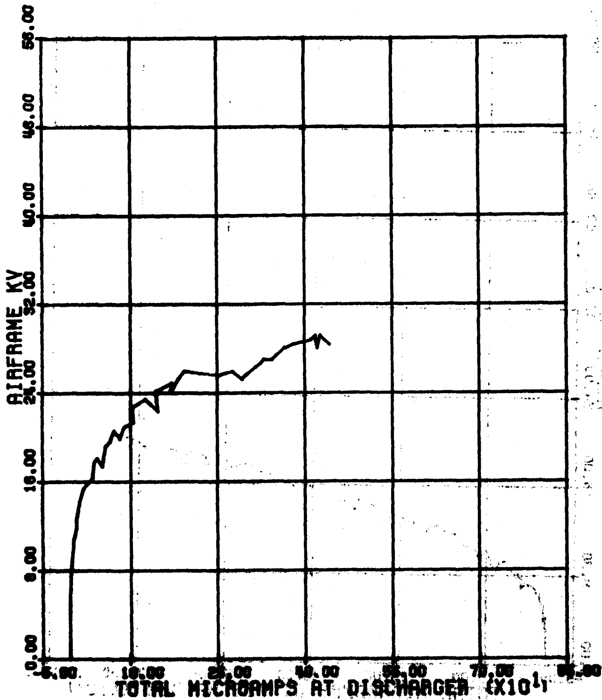
Figure 3-22. H019E11 28-MAY-81 DISCHARGE-DAYTON AREA DETECTOR-CAN., BROADBAND-WIDE POSITIVE POINT CORRELATION
