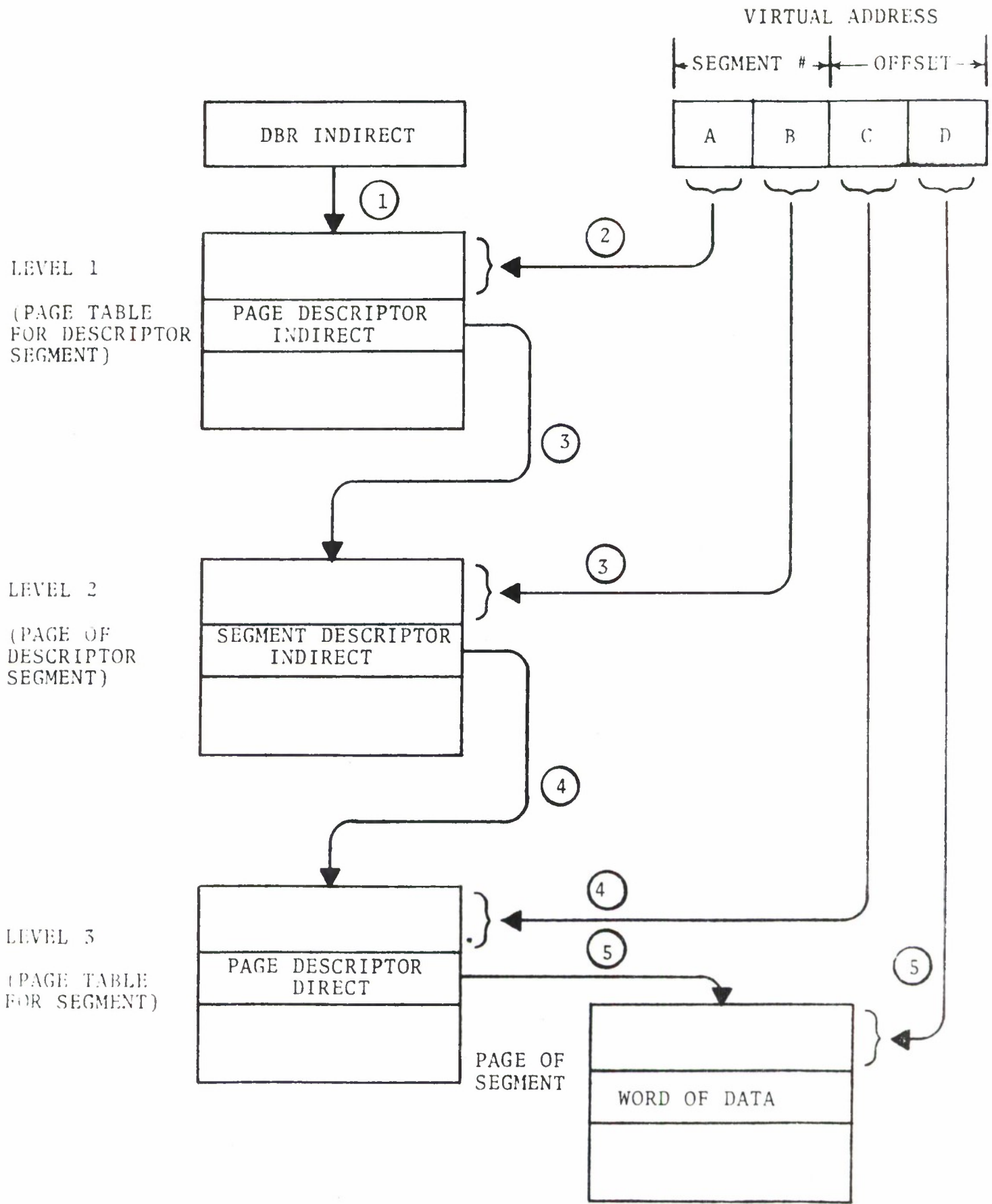
Figure 3. ADDRESS TRANSLATION
