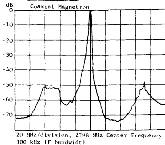
Figure 2-7, ASR
