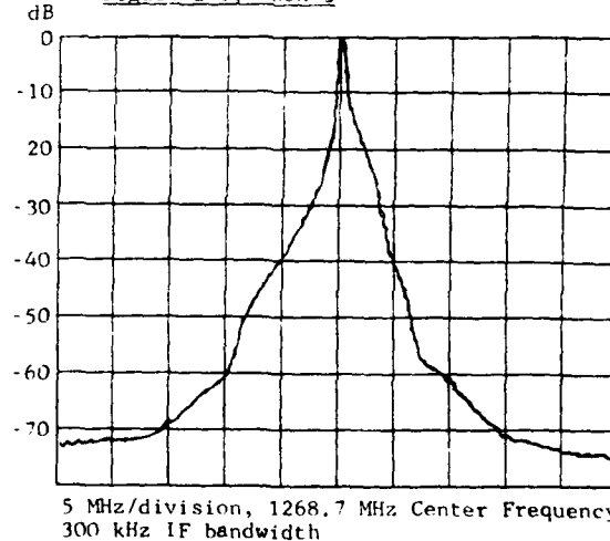
Figure 2-6, ARSR 3
