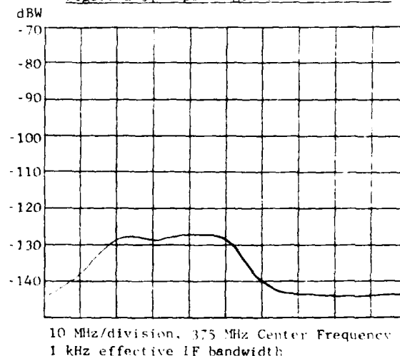
Figure 2-3, Super-Regenerative Receiver
