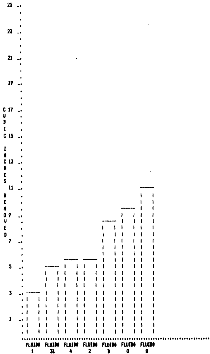
Figure 3.3-12. Cubic Inches of Metal Removed to .010" Flank Wear vs. Milling Fluids Tested.
