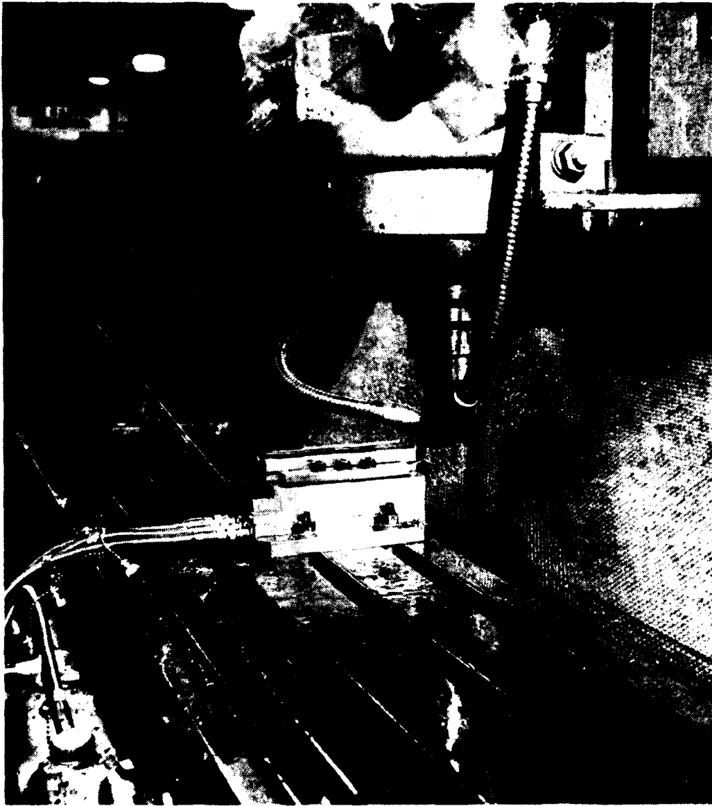
Figure 3.3-2. Photograph of the Milling Testing Arrangement.
