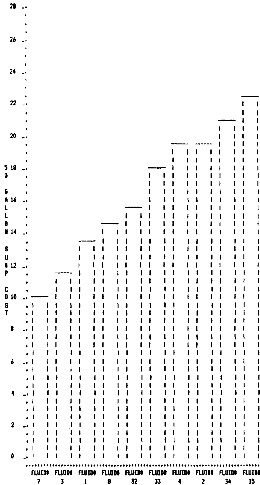
Figure 3.3-35. Price to Fill a 50 Gallon Sump vs. Turning Fluids Tested.
