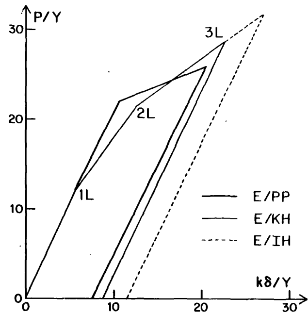
Fig. 9 Load-deflection curves.
