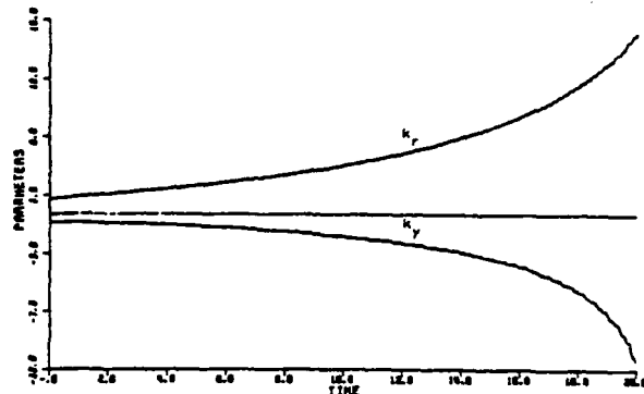
Figure 5: Simulation of CAL with unmodeled dynamics and r(t)=0.3 + 1.85\sin 16.lt . (System eventually becomes unstable).
