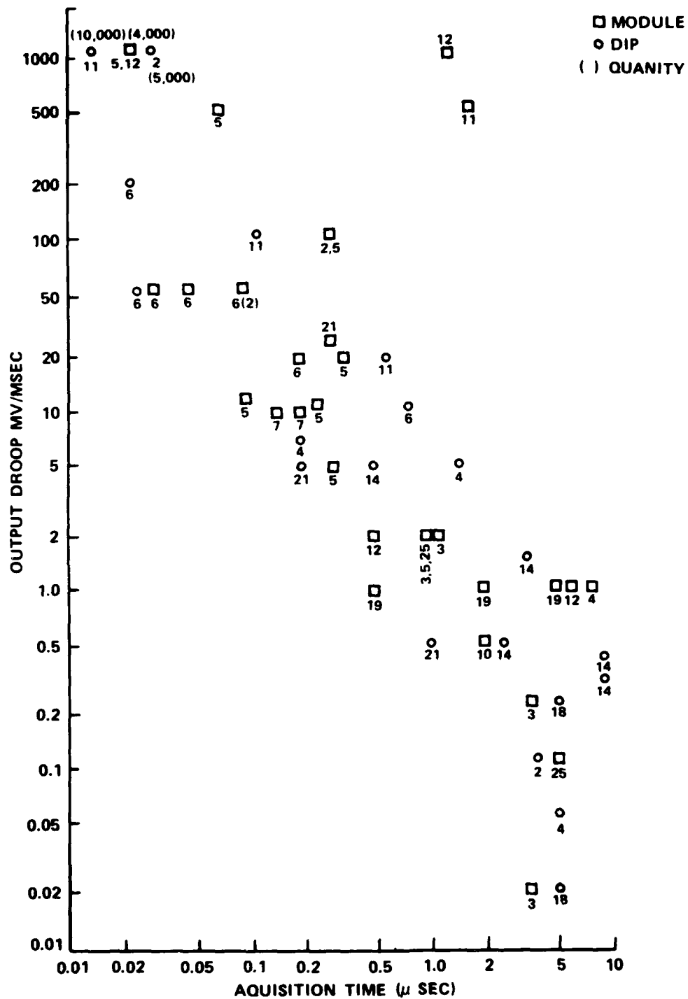
Figure 3. Sample and Hold Output Droop Rate.
