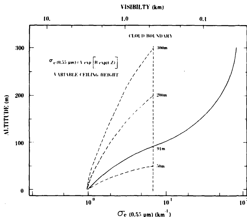
Figure 4a. The vertical profile of the 0.55μm extinction coefficient for various cloud ceiling heights. The solid line shows the averaged profile using table 1a.
