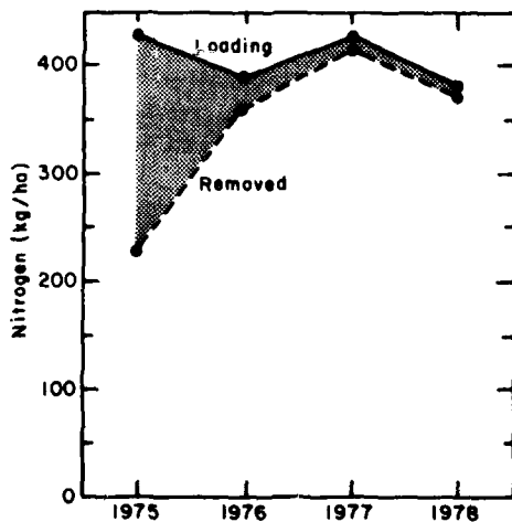
Figure 6. Nitrogen loading and net N removed during the initial 4 years following the establishment of a poplar plantation (after Cole and Schiess 1978).
