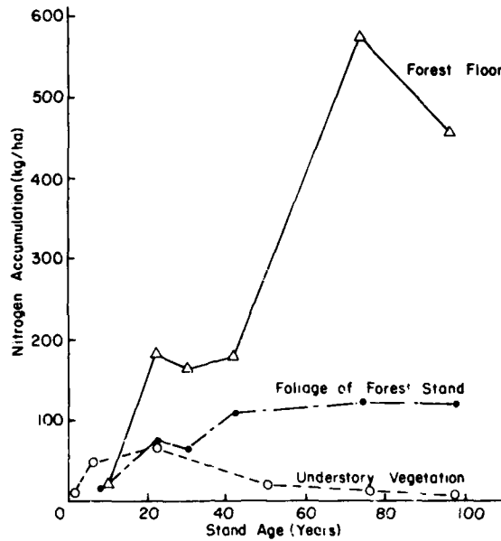
Figure 9. Accumulation of total N in an undisturbed Douglas-fir forest in the three compartments: 1) forest floor, 2) understory vegetation, and 3) foliage of forest stand (after Cole et al. 1975).
