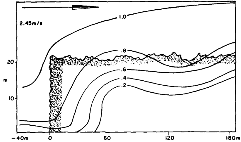
Figure 1. Vertical cross section of wind speed normalized to a reference wind speed above the canopy with wind blowing into the forest (after Fritschen et al. 1970).
