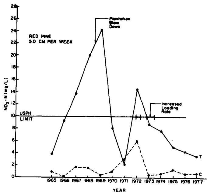
Figure 8. Average annual nitrate-N concentration in soil water at the 120-cm soil depth in the Penn State red pine forest ecosystem irrigated with municipal wastewater at 5.0 cm/wk during the growing season for the period 1965 to 1977.
